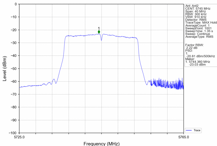
802.11n(HT20)_LCH_5745MHz_Ant2_NTNV
