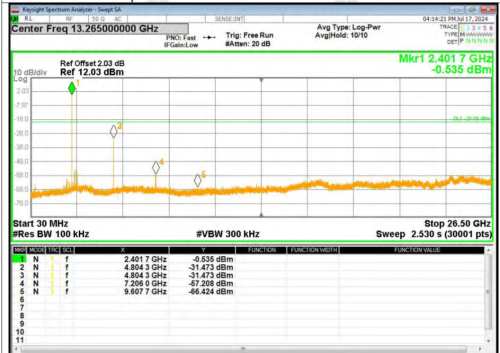
Tx. Spurious NVNT 1-DH5 2402MHz Ant1 Emission
