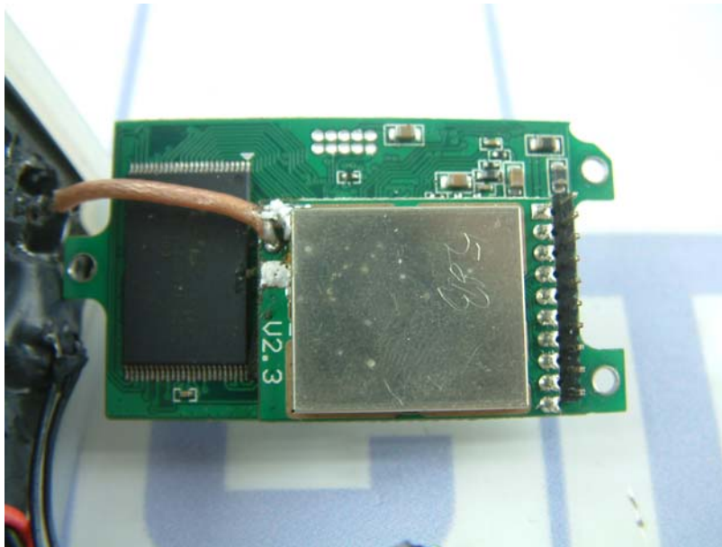
PCB 2 side 2
