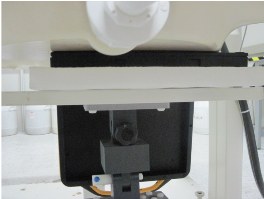
Body SAR Bottom of Laptop 0mm for GPRS/WCDMA
