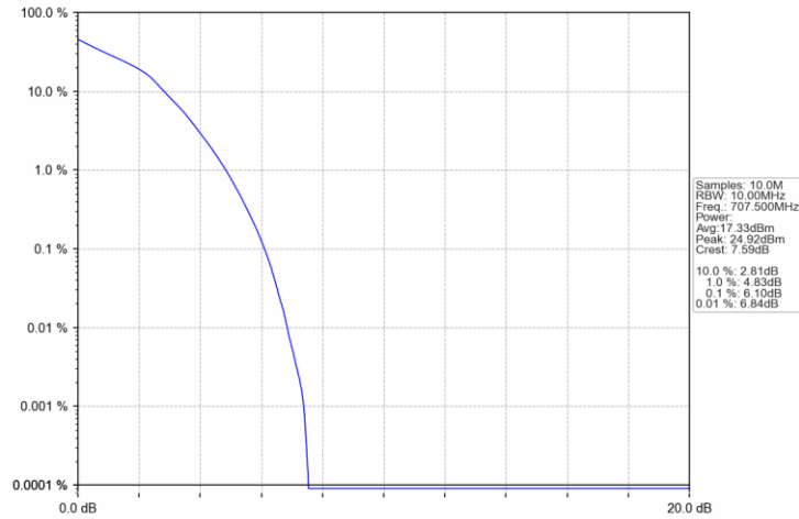
Band12_10MHz_16QAM_MCH_707.5MHz_RB_50_0_NTNV
