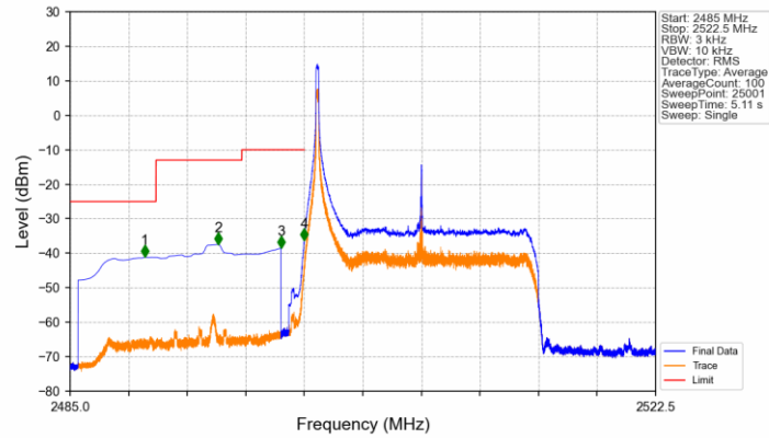
Band7_15MHz_QPSK_LCH_2507.5MHz_RB_1_0_NTNV
