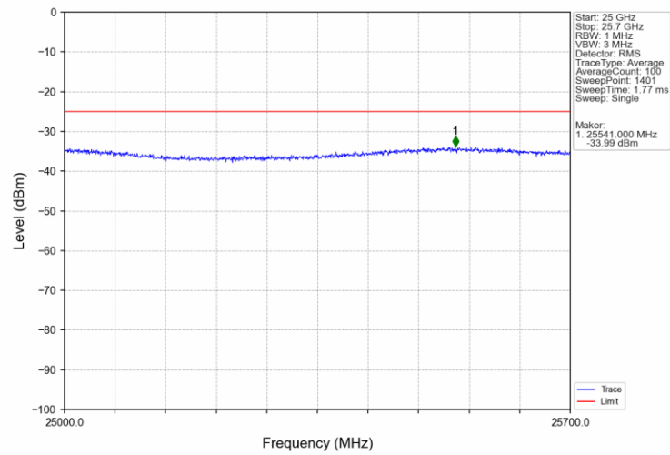
Band7 15MHz 16QAM MCH 2535MHz RB 1 0 NTV
