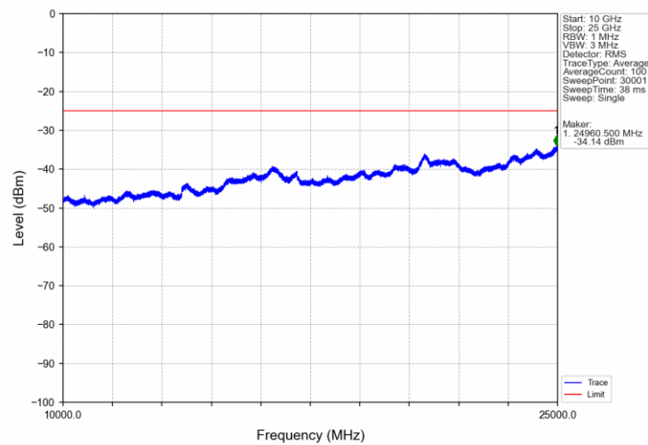
Band7 5MHz 16QAM LCH 2502.5MHz RB 1 0 NTV
