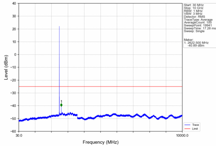
Band7 5MHz 16QAM LCH 2502.5MHz RB 1 0 NTV
