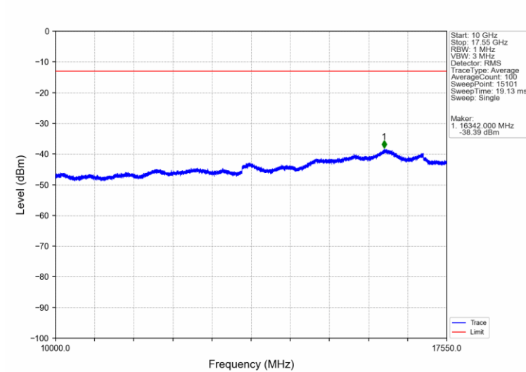
Band4_1.4MHz_QPSK_LCH_1710.7MHz_RB_1_0_NTNV
