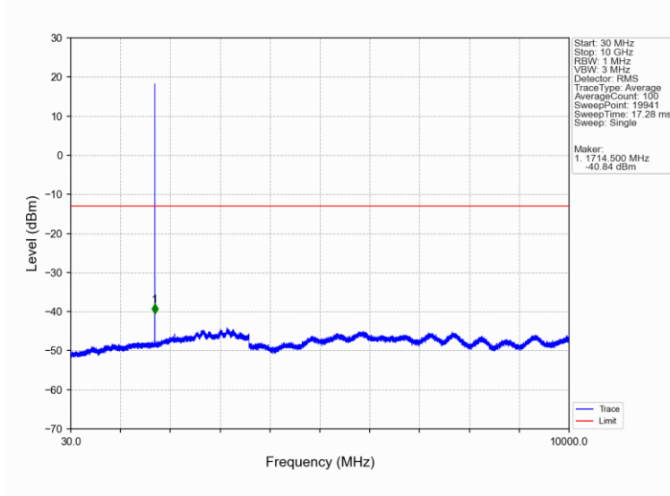
Band4_1.4MHz_QPSK_LCH_1710.7MHz_RB_1_0_NTNV
