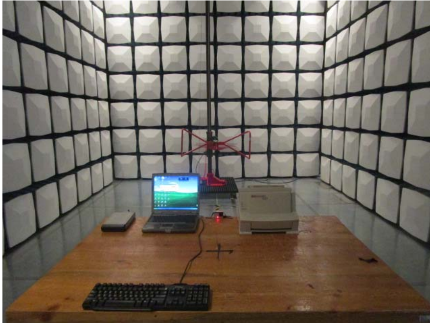
Conducted Emissions - Front View (Downloading)
