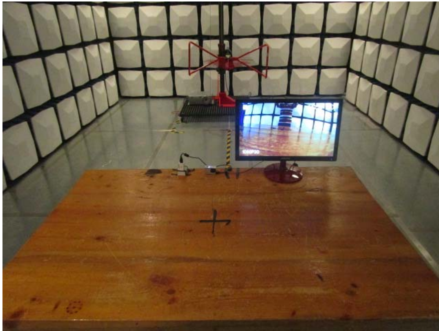
Conducted Emissions - Front View (HDMI)
