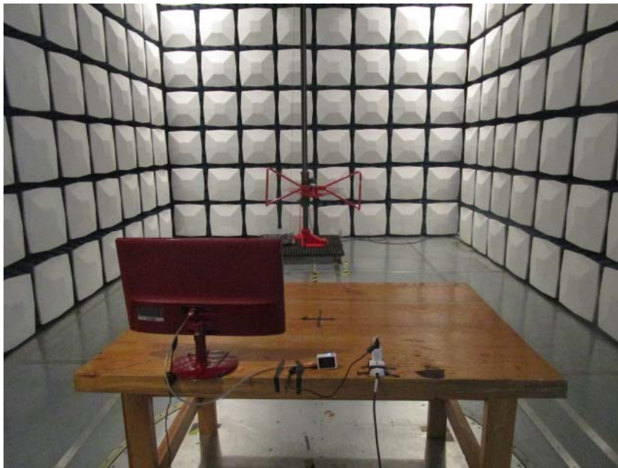
Radiated Emissions Below 1GHz –Rear View (HDMI)
