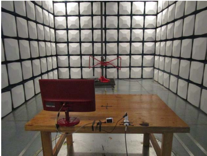
Conducted Emissions – Side View (HDMI)
