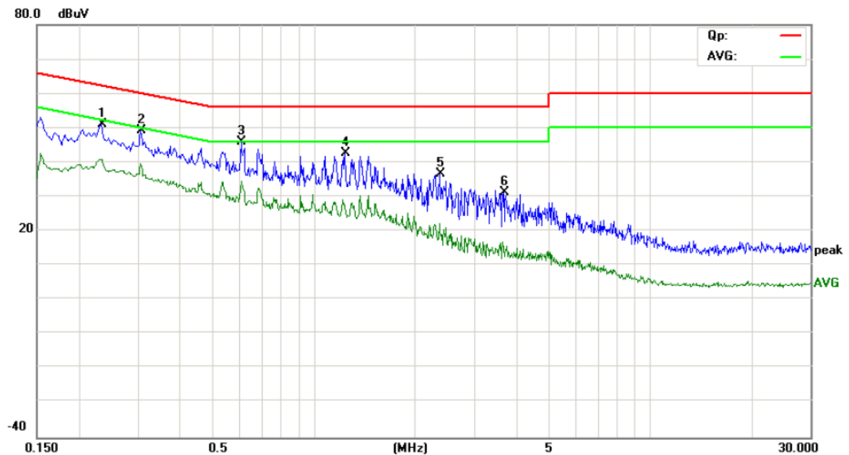
Conducted Emission Measurement
