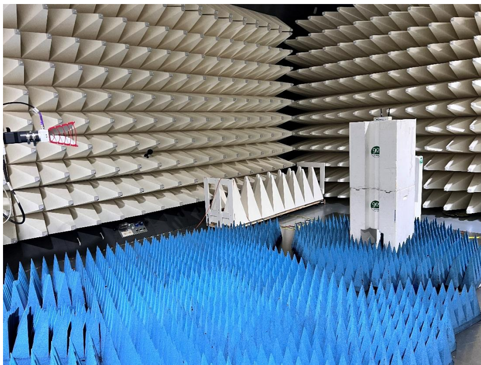
5. Radiated Emission test setup High Range 1
