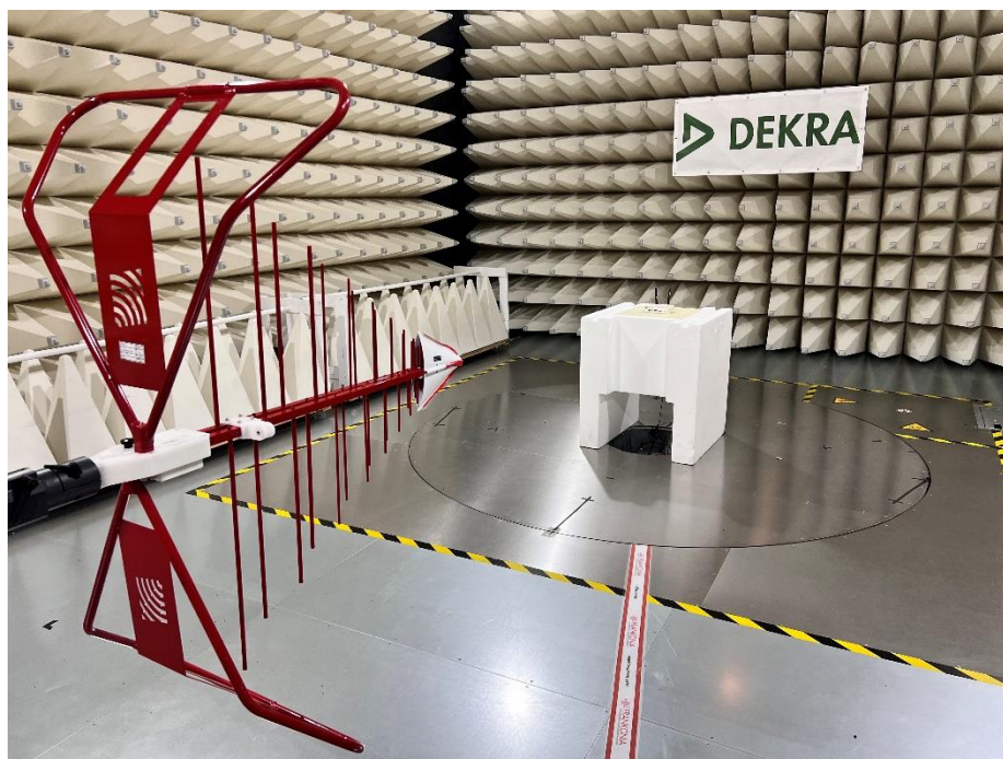
4. Radiated Emission test setup Low Range
