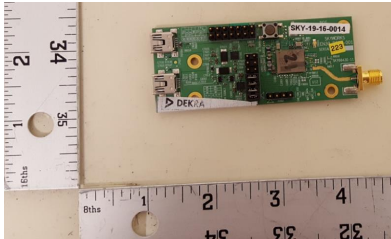
Figure B1. DUT top view
