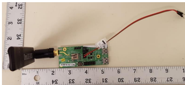
Figure B3. DUT Antenna and power cable attached view
