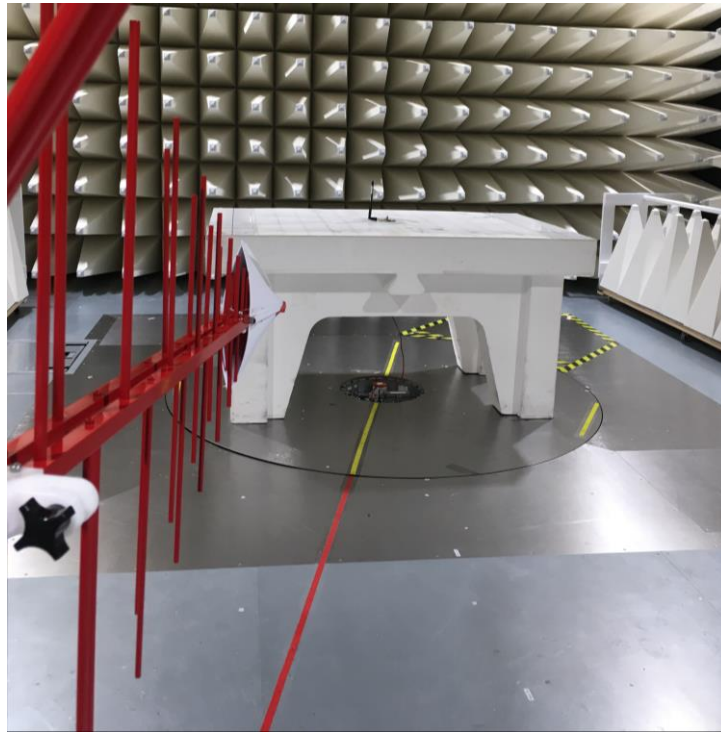
Figure B4. Low range Radiated emission Set up Biconical log antenna
