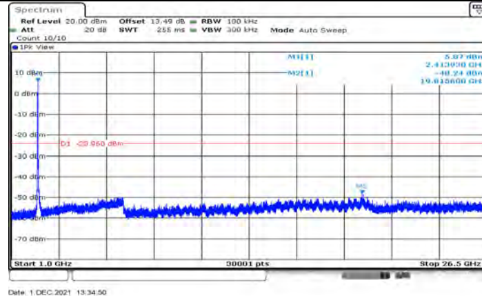
11G_Ant1_2412_1000-26500
