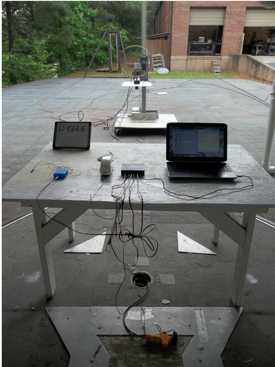
Rear View Radiated Emissions Test Setup with Loop Antenna
