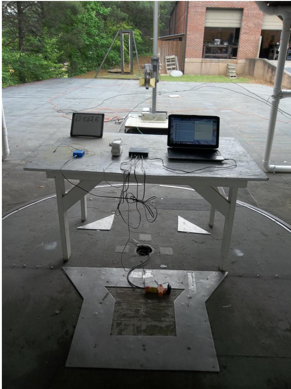
Rear View Radiated Emissions Test Setup with Horn Antenna
