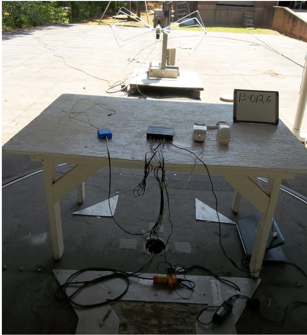
Rear View Radiated Emissions Test Setup with Biconical Antenna
