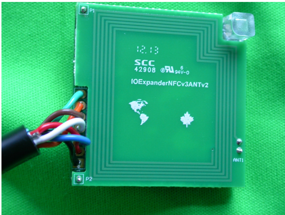
Figure 2: Transmitter/main board – internal photo – bottom
