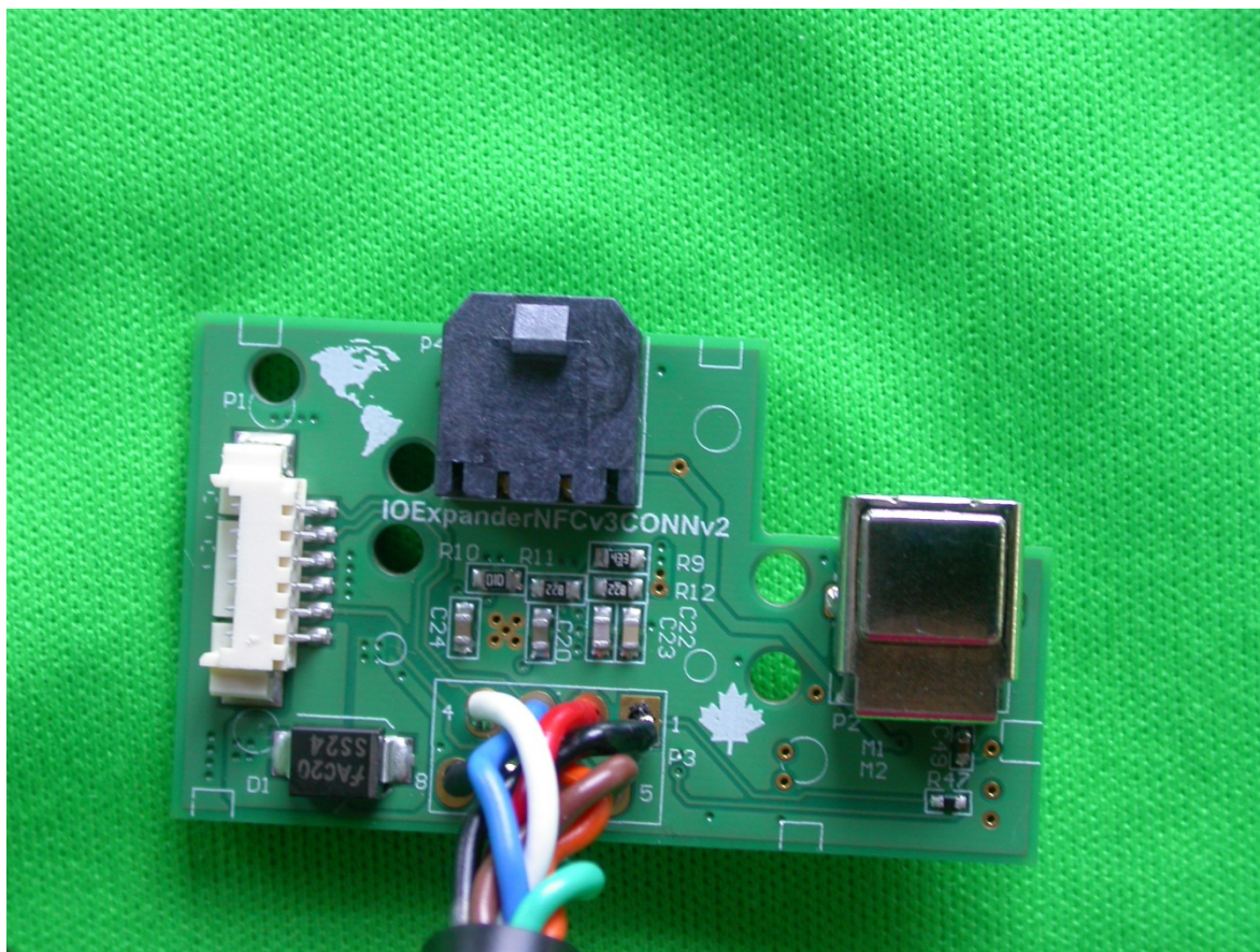
Figure 3: Interface board – internal photo 1
