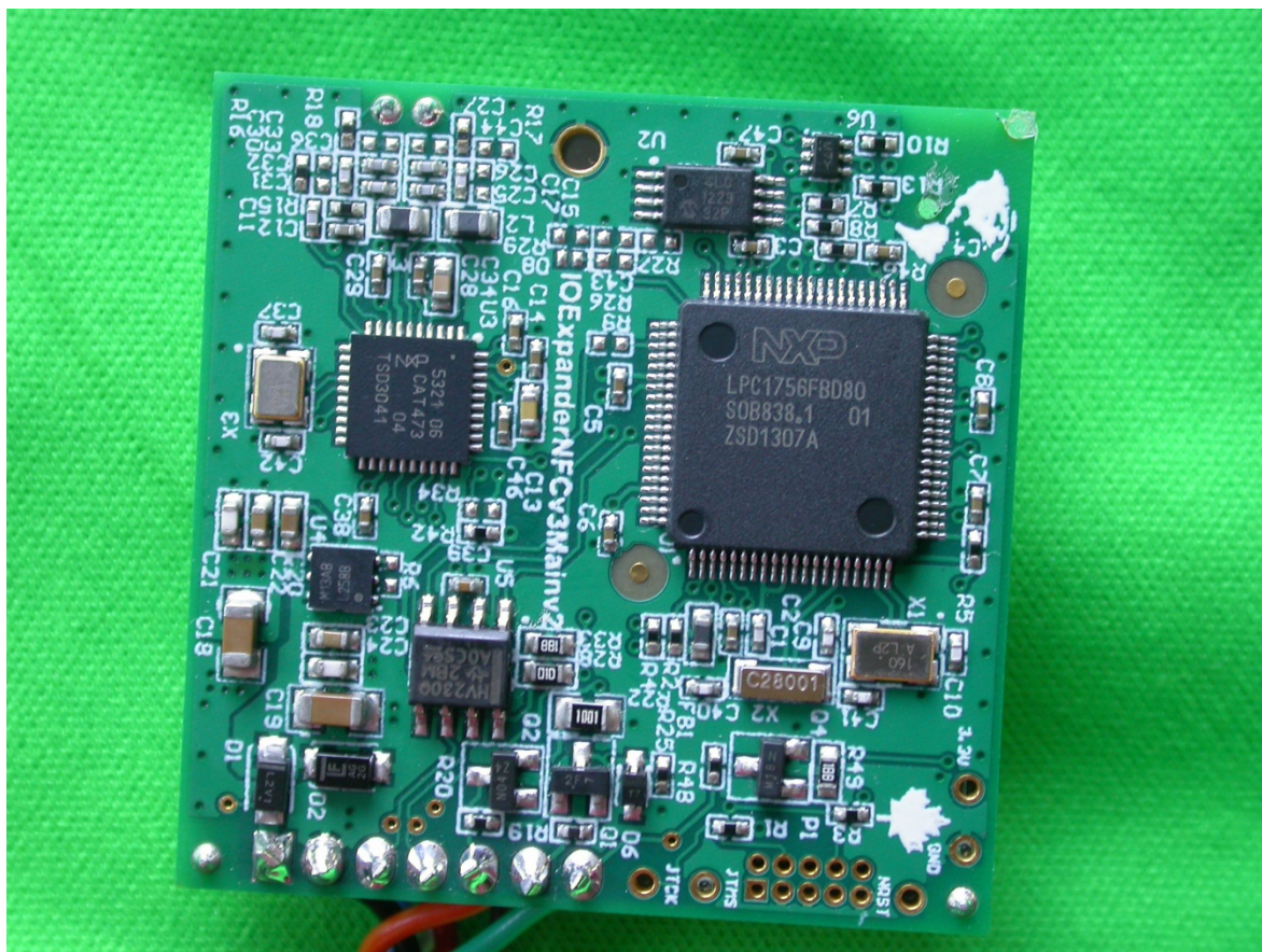
Figure 1: Transmitter/main board – internal photo – top
