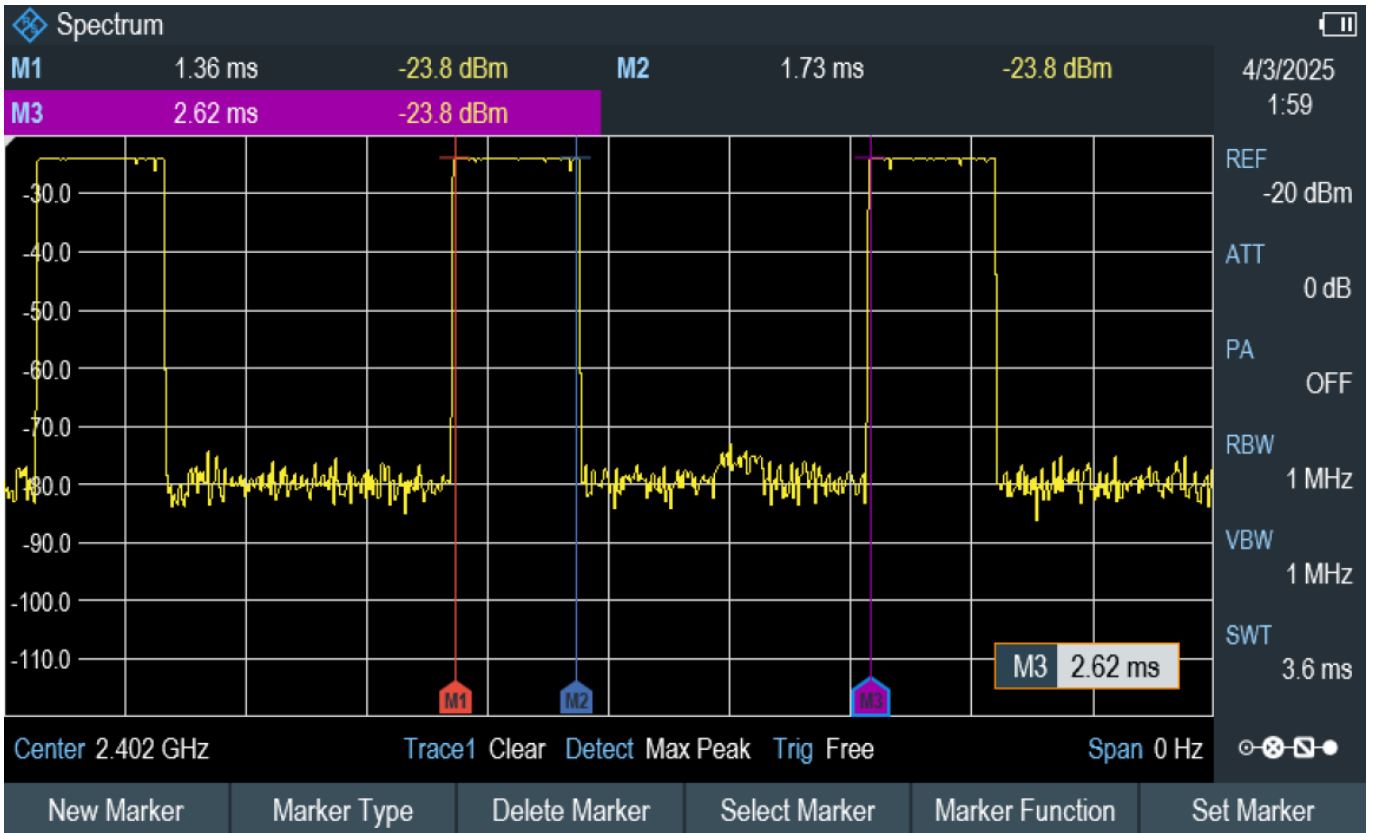
Time-domain plot for SRD transmission signal
