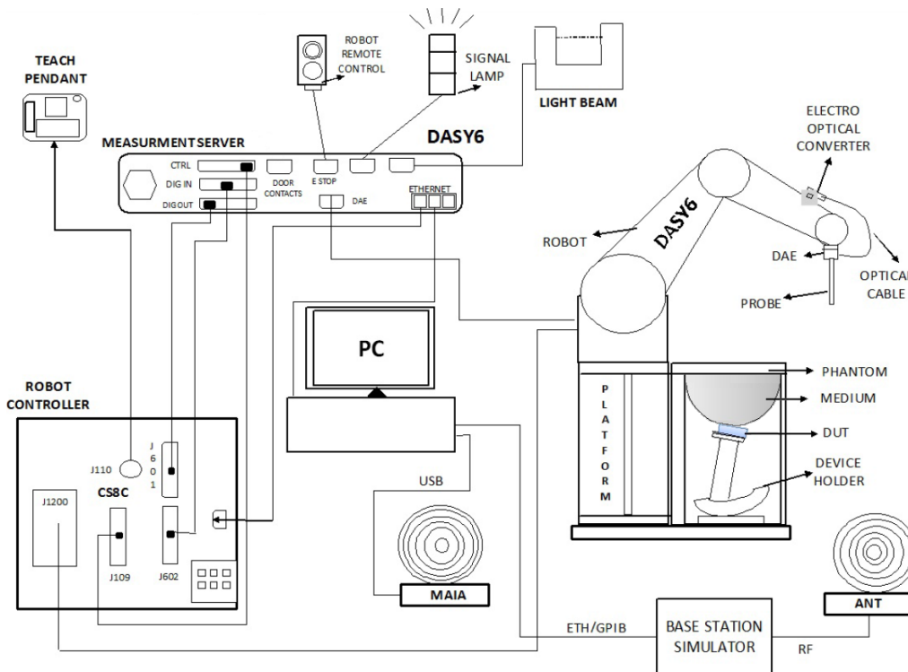
Fig-4.1 SPEAG DASY6 System Setup
