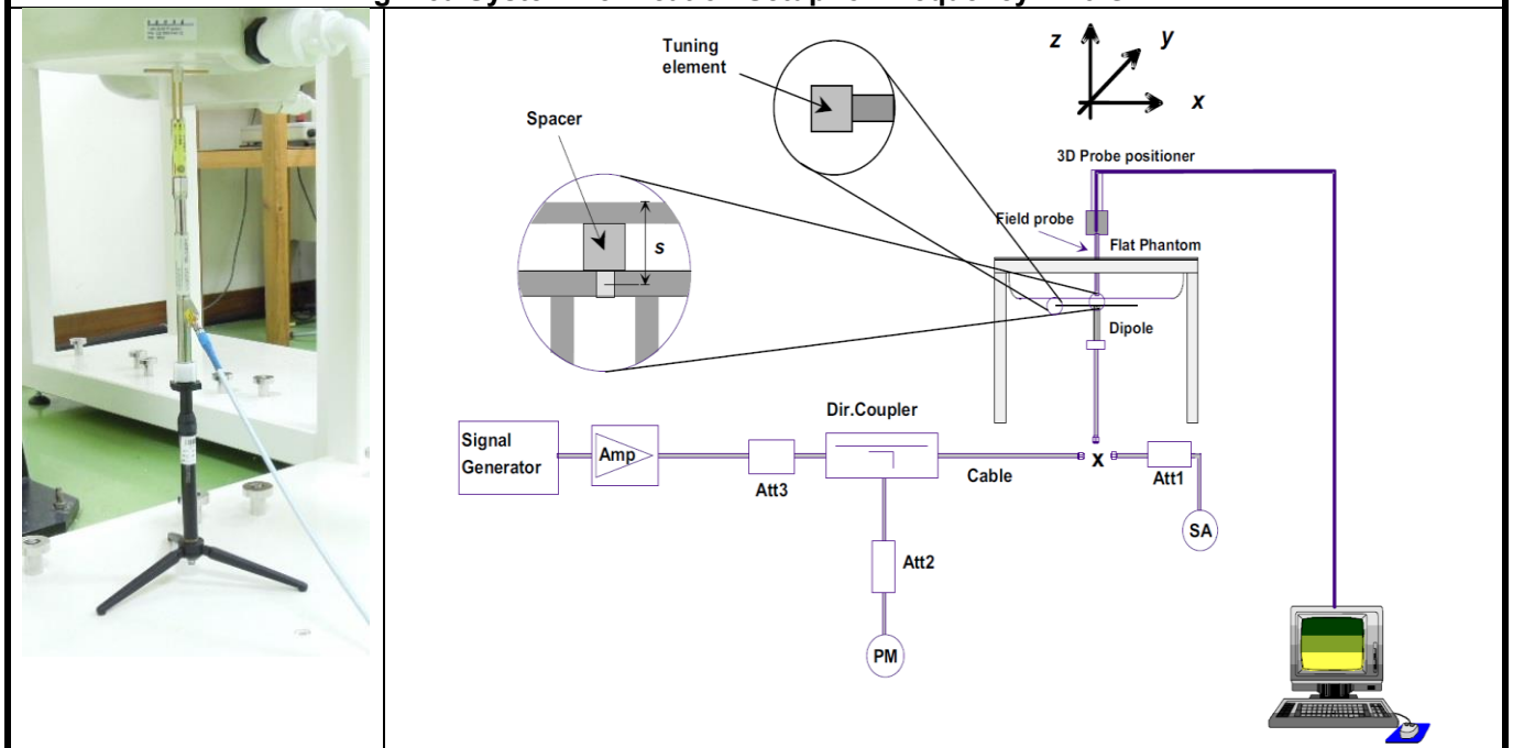
Fig-4.3b System Verification Setup for Frequency > 6 GHz
