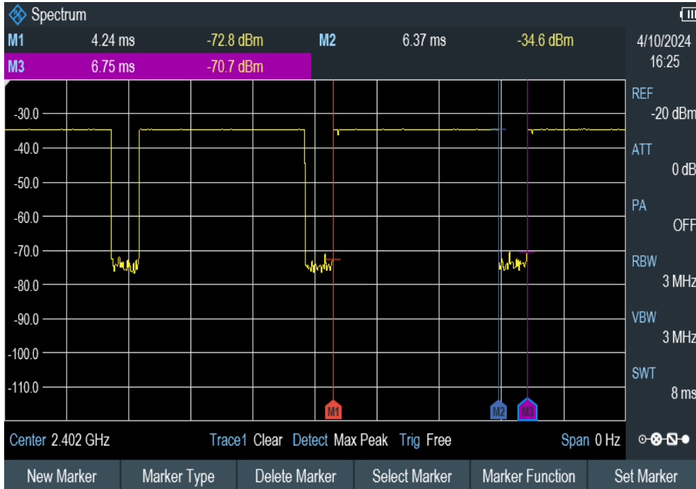
Time-domain plot for SRD transmission signal
