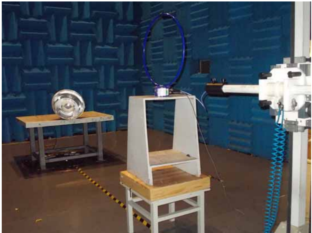
VERTICAL POLARIZATION
