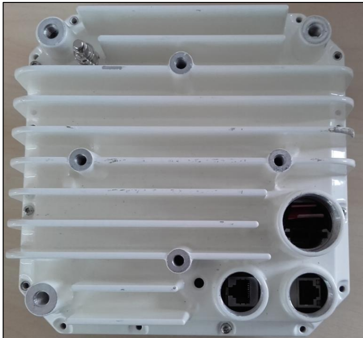
Figure 6: Rear view of Liberator-V1000 Dual-port showing 3 cable ports (all open): 2 Gigabit Ethernet copper ports with RJ45 sockets, and a single port with for insertion of optical SFP module.
