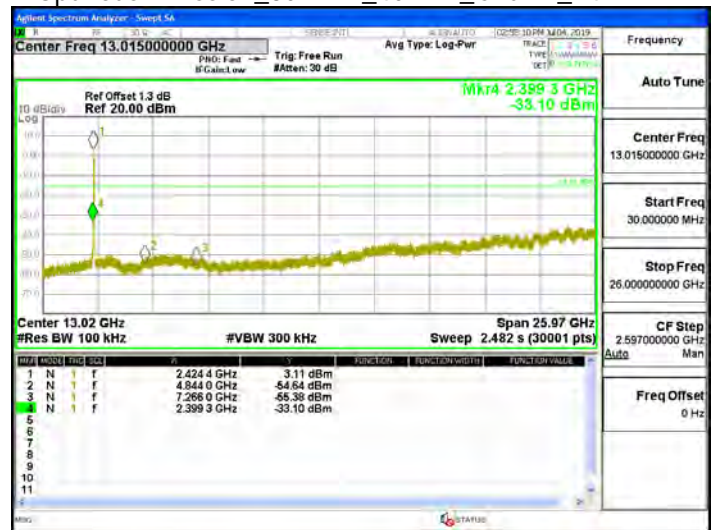
Spurious Emission_802.11n_40MHz_Chain1_2437MHz
