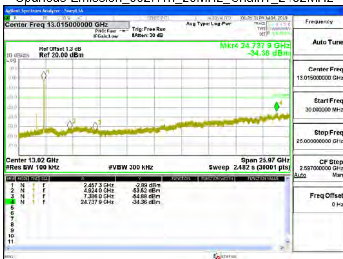
Spurious Emission_802.11n_20MHz_Chain1_2462MHz
