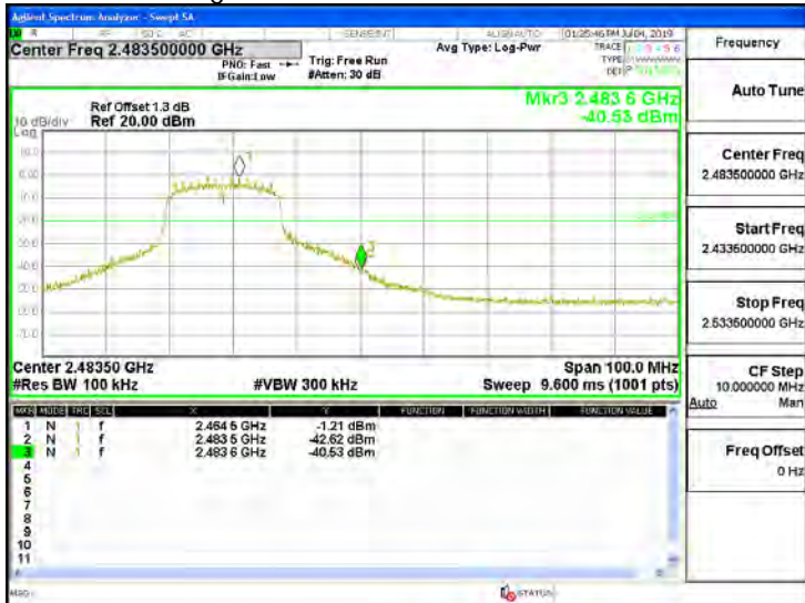
Band Edge_802.11n_20MHz_Chain1_2462MHz
