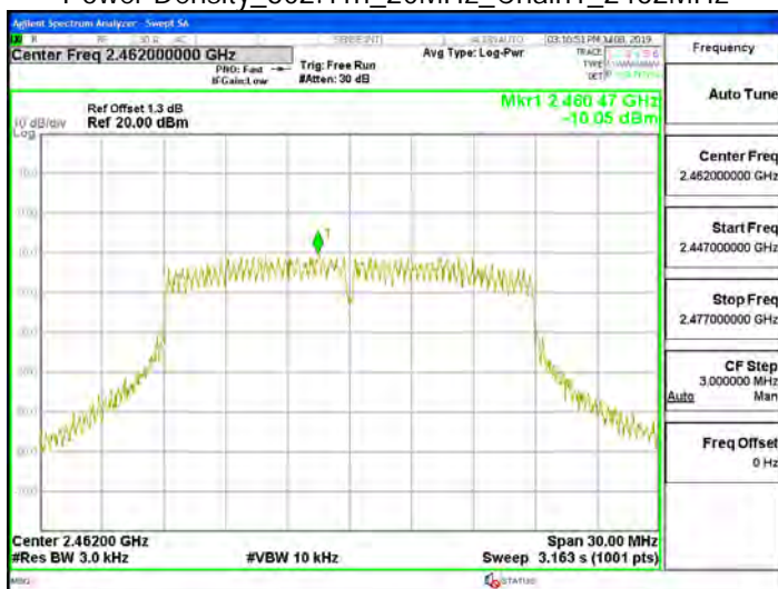
Power Density_802.11n_20MHz_Chain1_2462MHz
