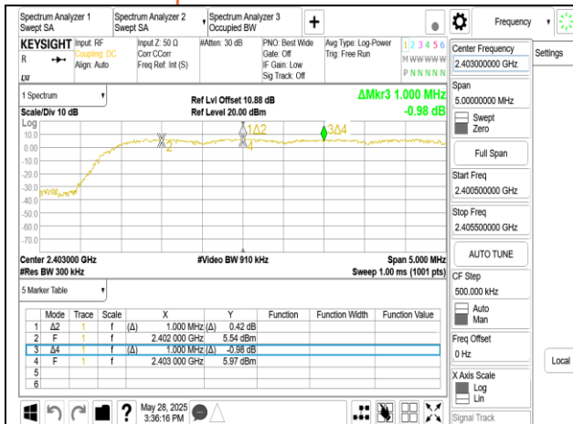
8DPSK 3M_DH5_CH0CH1CH2
