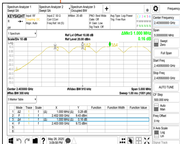
GFSK 1M_DH5_CH0CH1CH2
