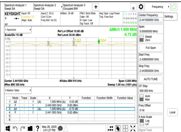
8DPSK 3M_DH5_CH38CH39CH40
