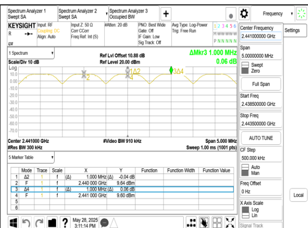
GFSK 1M_DH5_CH38CH39CH40
