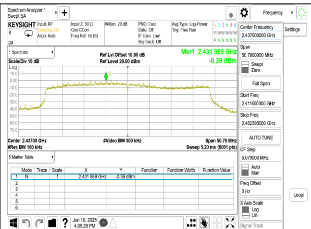
802.11ax_40MHz_Chain0_2437MHz
