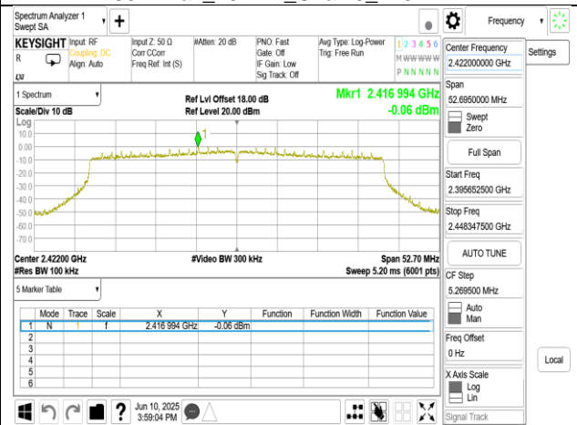
802.11ax_40MHz_Chain1_2422MHz
