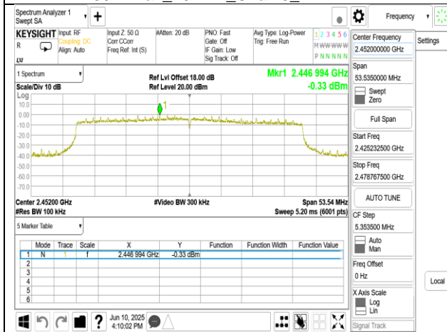
802.11ax_40MHz_Chain0_2452MHz
