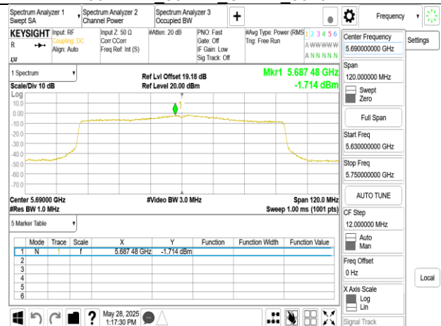
802.11ax 80MHz Chain1 5690MHz UNII 2C
