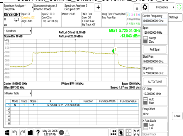
802.11ax_80MHz_Chain0_5690MHz_UNII 3
