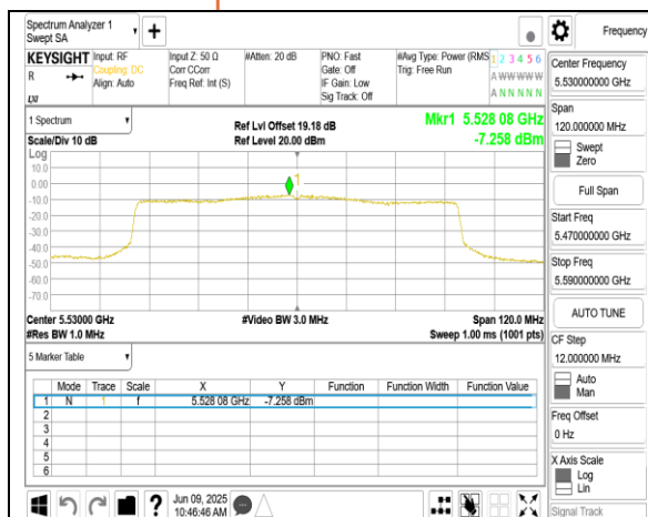
802.11ax_80MHz_Chain0_5530MHz
