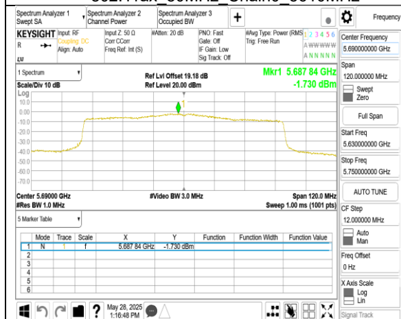
802.11ax_80MHz_Chain0_5690MHz_UNII 2C
