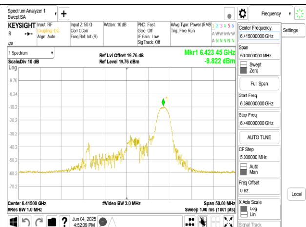
802.11ax_20MHz_Chain1_6415MHz_RU26_8
