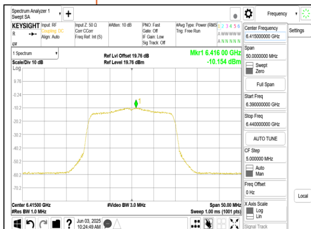
802.11ax_20MHz_Chain1_6415MHz
