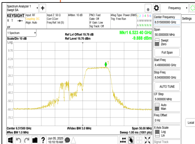
802.11ax 20MHz Chain1 6515MHz RU106_54
