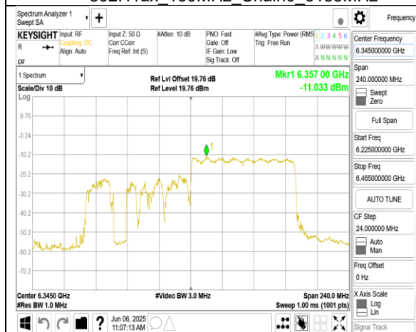
802.11ax_160MHz_Chain0_6345MHz_RU996_S67
