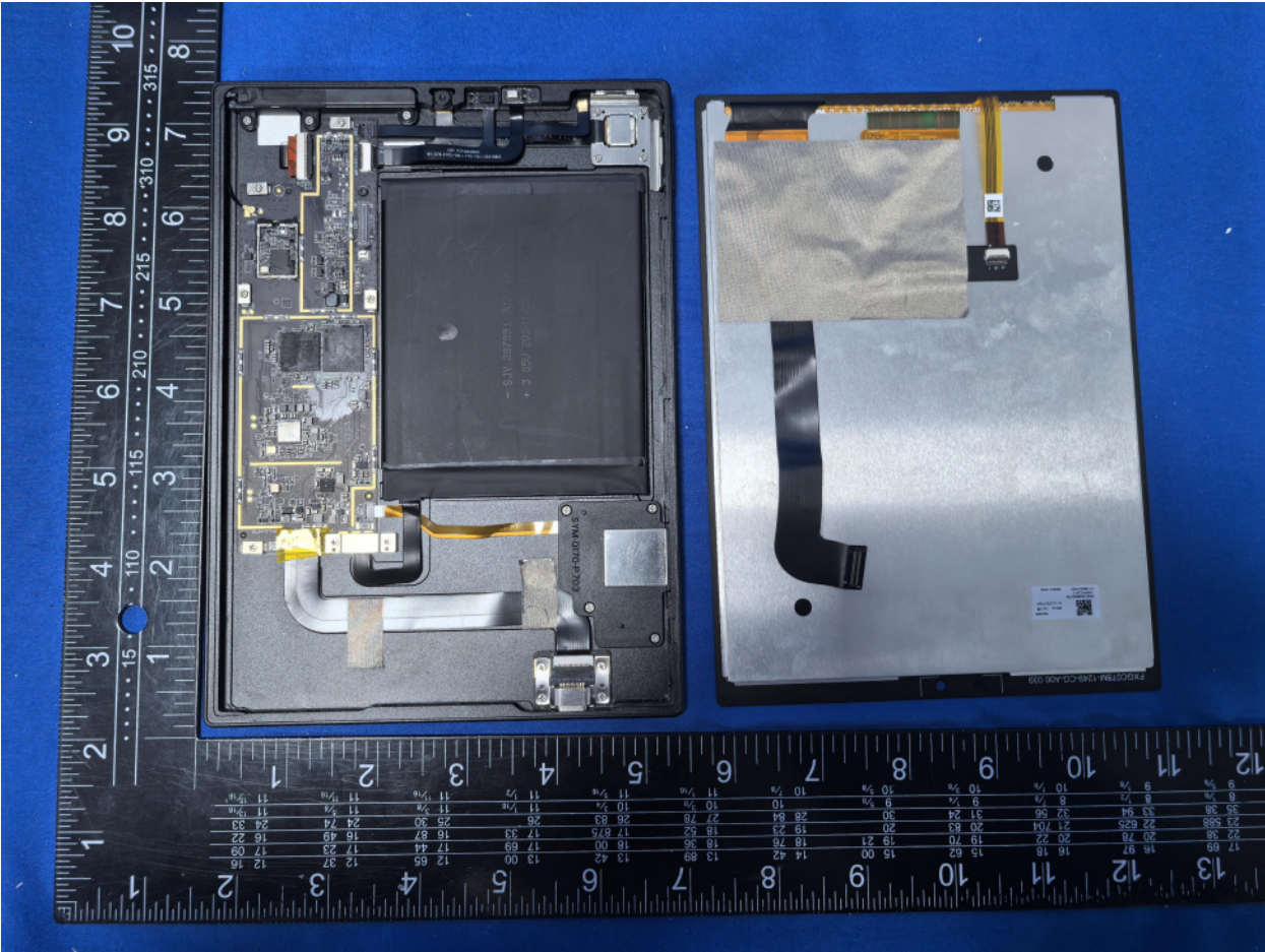
EUT Internal View 1
