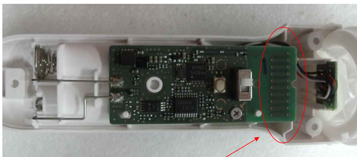
Receiving Antenna
