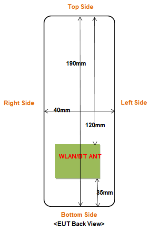
Fig 7.1 Block Diagram for EUT Antenna Position
