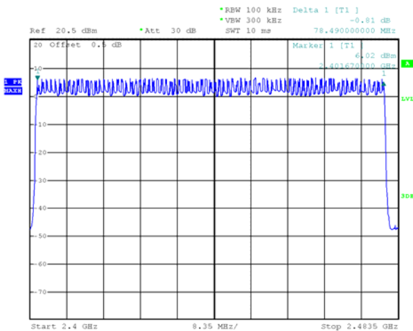
Modulation: 8DPSK
