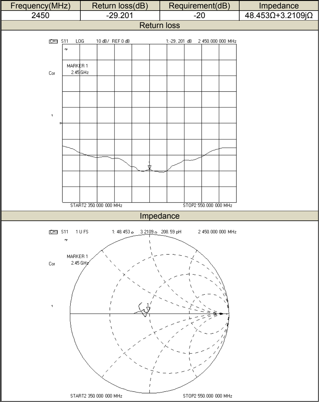
Return Loss and Impedance in Head liquid(2021-08-25)
