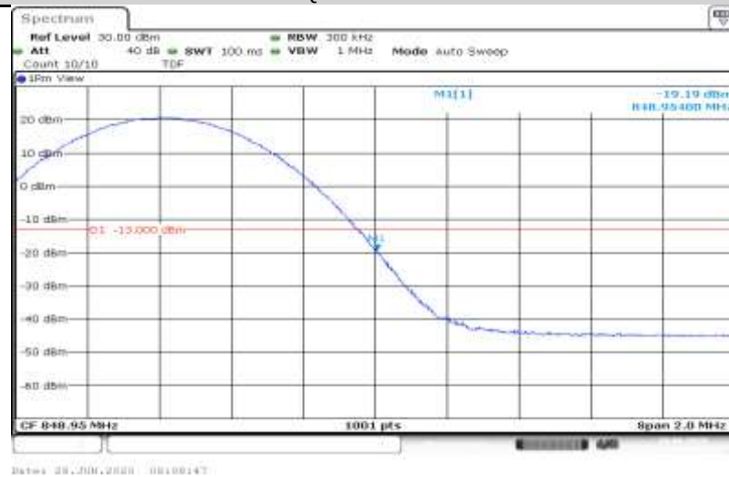
5-5-10MHz-5MHz-16QA M-20550-20622-50RB#0-25RB#0
