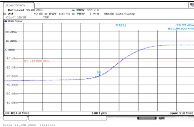
5-5-10MHz-5MHz-16QA M-20550-20622-0RB#0-1RB#24
