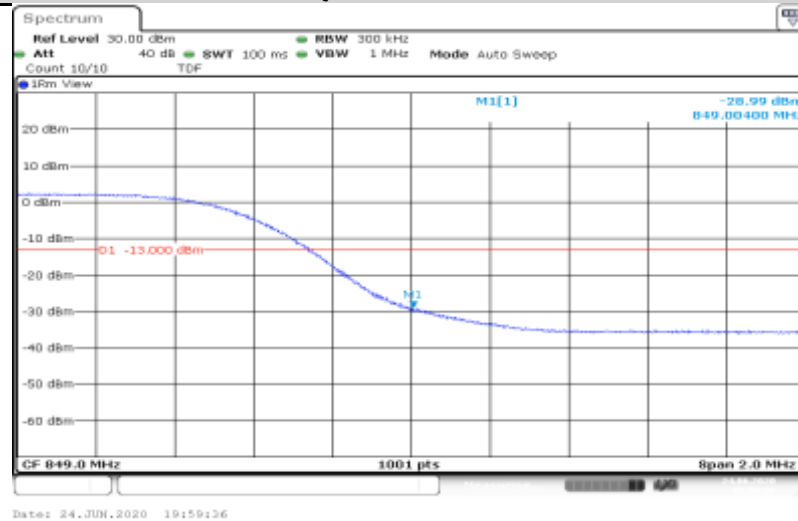
5-5-10MHz-10MHz-16QAM-20450-20549-1RB#0-0RB#0
