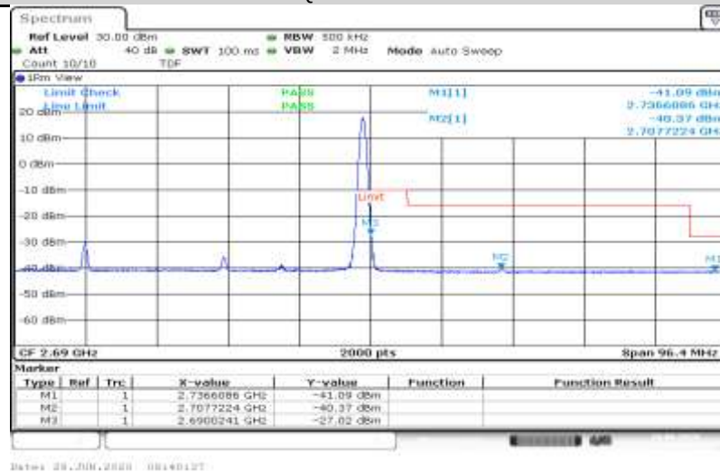
41-41-20MHz-20MHz-QPSK-41292-41490-100RB#0-100RB#0
