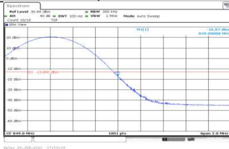
5-5-5MHz-10MHz-16QA M-20528-20600-25RB#0-50RB#0
