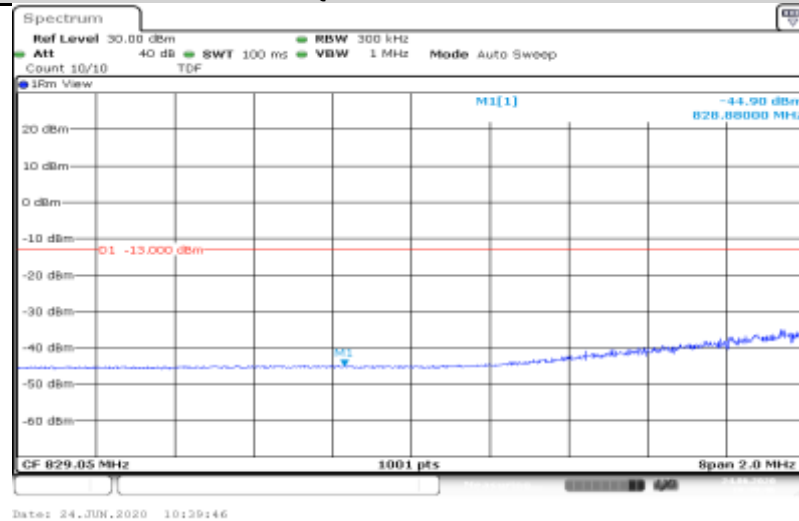
5-5MHz-10MHz-QPSK-20528-20600-0RB#0-1RB#49
