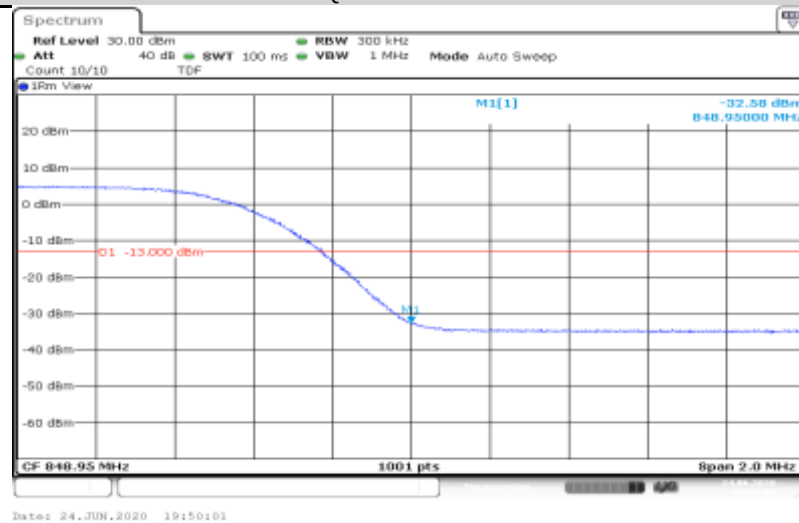
5-5-5MHz-10MHz-QPSK-20428-20500-1RB#0-0RB#0
