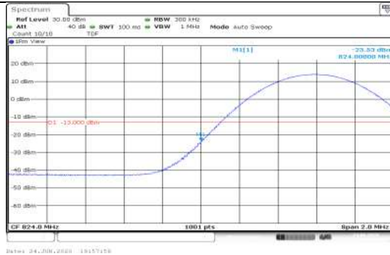
5-5-10MHz-10MHz-QPSK-20501-20600-0RB#0-1RB#49
