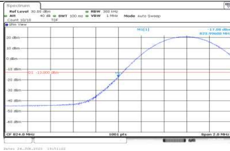
5-5-10MHz-10MHz-16QA M-20450-20549-50RB#0-50RB#0
