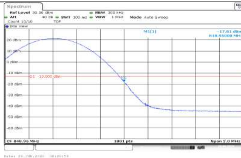
5-5-10MHz-5MHz-QPSK-20550-20622-50RB#0-25RB#0
