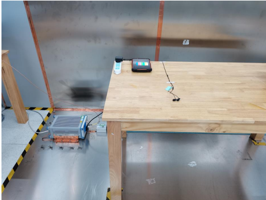
Photograph 1: Set-up photo for Conducted Emission
