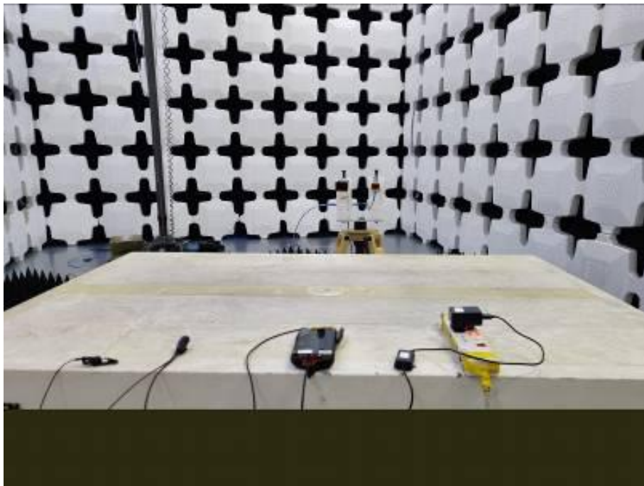
12. Radiated Emissions (Part 15B Charging mode Type C Wire + Headset) (26.5G-30GHz)
