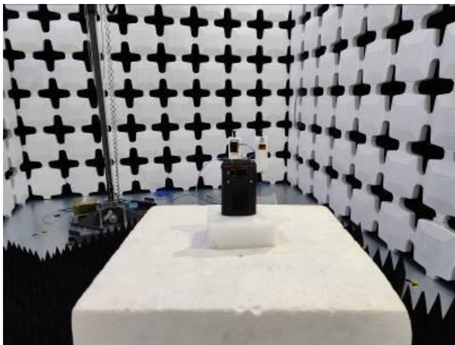
16. Radiated Emissions (Part 15C&E 18G-26.5GHz)
