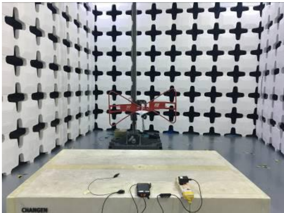
6. Radiated Emissions (Part 15B Charging mode Type C Wire + Headset) (below 1GHz)
