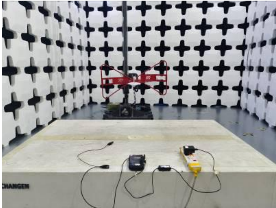
5. Radiated Emissions (Part 15B Charging mode Magnetic wire+Headset) (below 1GHz)
