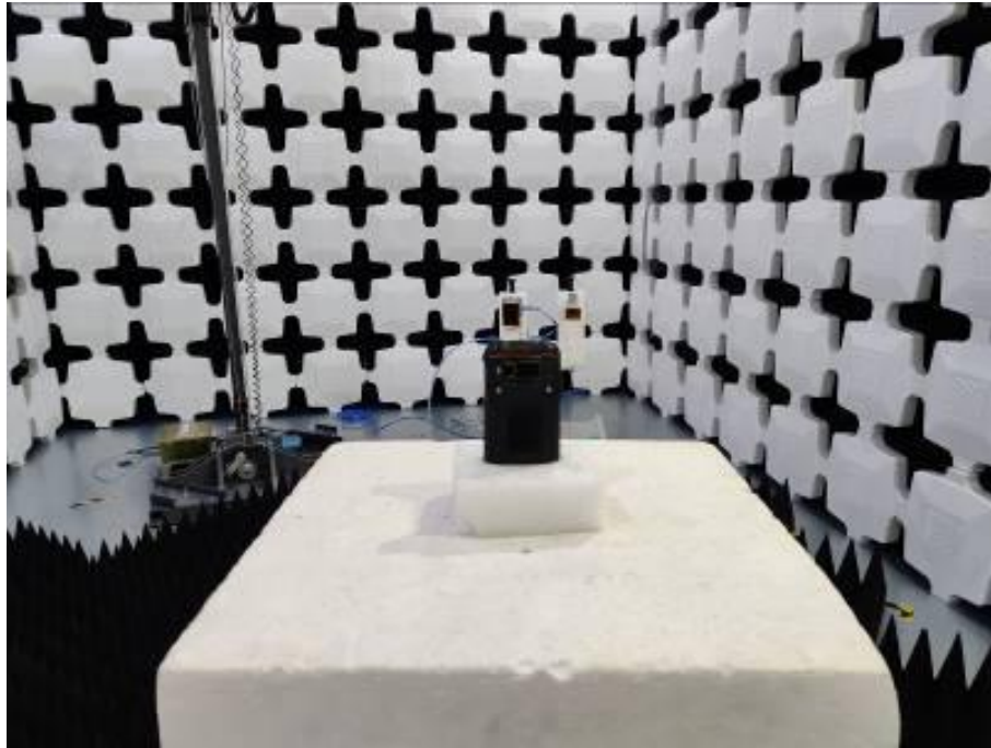
19. Radiated Emissions (Part 22/24/27,18G-26.5GHz)
