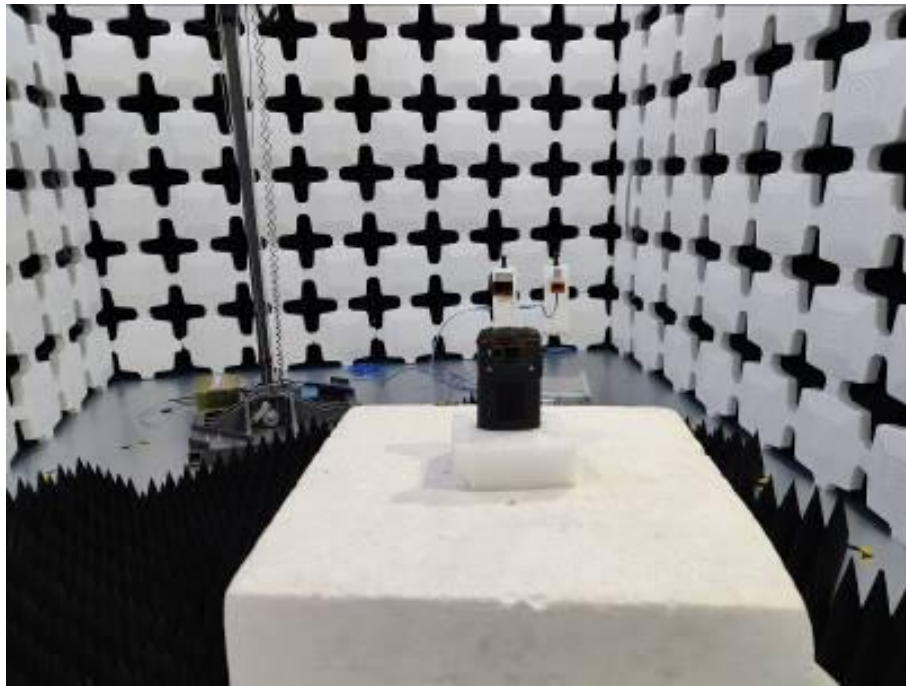
17. Radiated Emissions (Part 15E 26.5G-40GHz)
