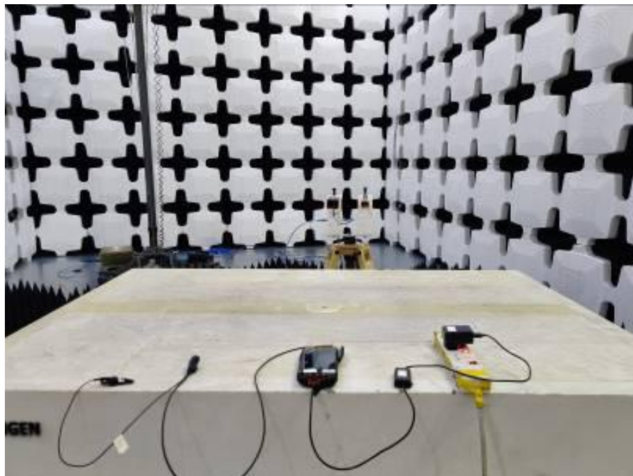
10. Radiated Emissions (Part 15B Charging mode Type C Wire + Headset) (18G-26.5GHz)
