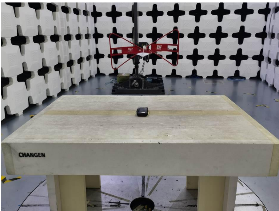
14. Radiated Emissions (Part 15C&E 30M-1GHz)
