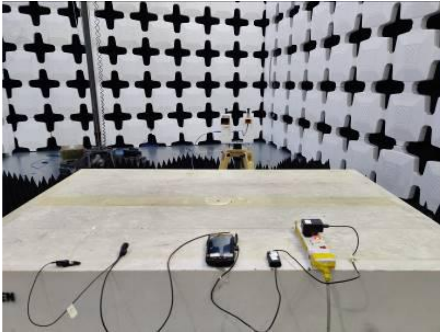
11. Radiated Emissions (Part 15B Charging mode Magnetic Wire+Headset) (26.5G-30GHz)
