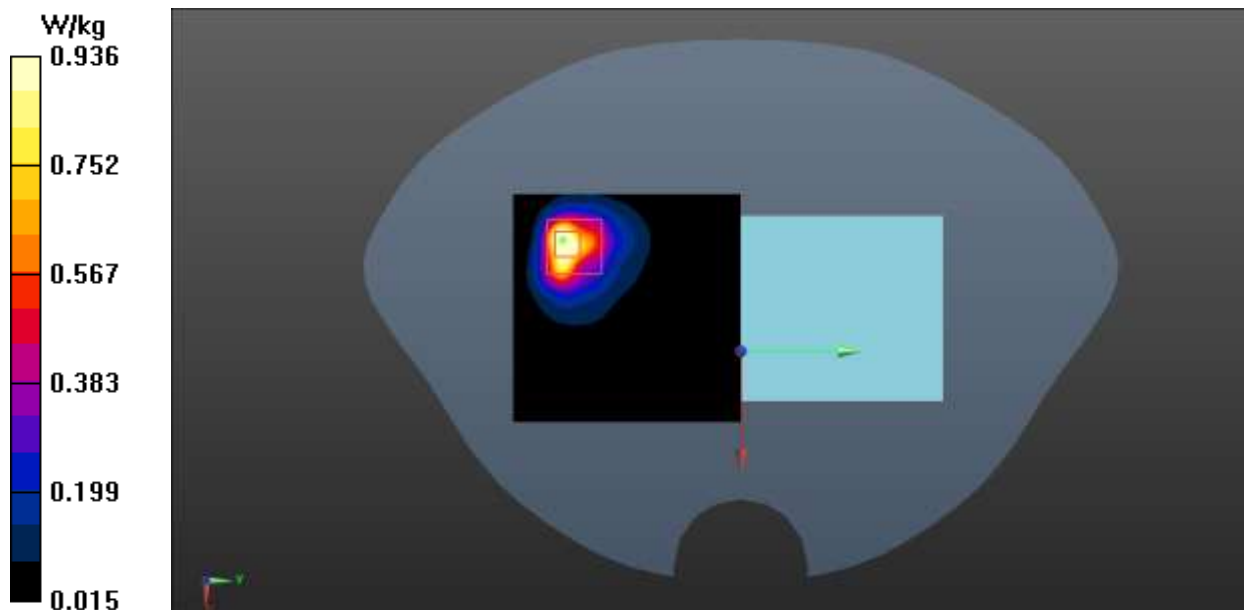
Fig.34 WLANB 5G Body
