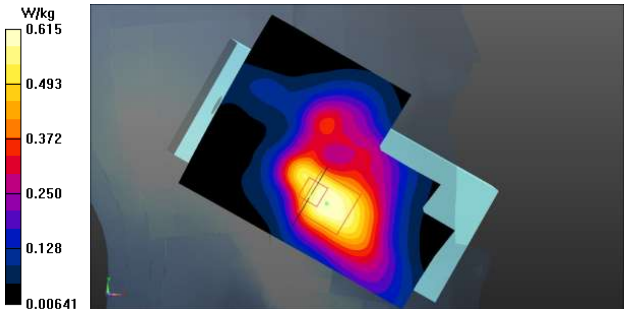
Fig.25 LTE Band 30 Head
