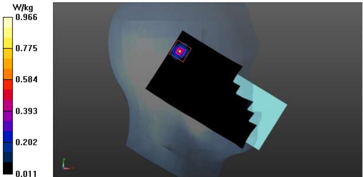
Fig.33 WLAN 5G Head
