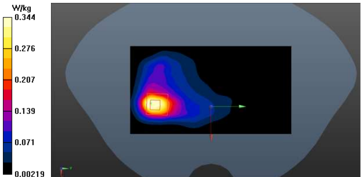
Fig.32 WLAN 2.4G Body
