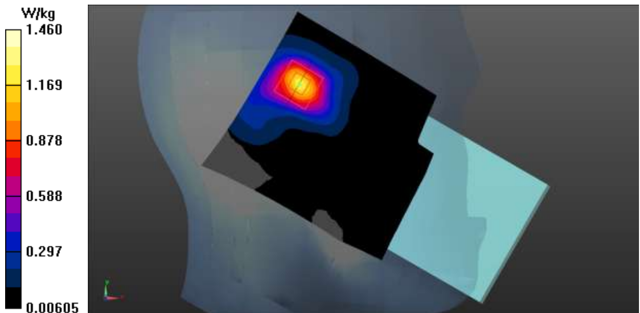
Fig.31 WLAN 2.4G Head
