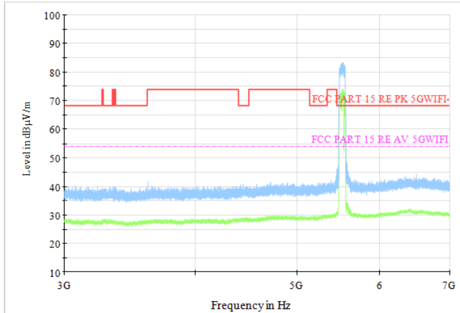
Fig. 110 Transmitter Spurious Emission (802. 11ac-VHT80, CH106 5530MHz)
