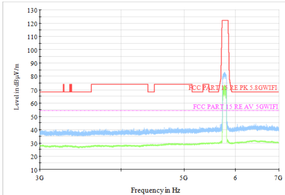
Fig. 114 Transmitter Spurious Emission (802. 11ac-VHT80, CH155 5775MHz)
