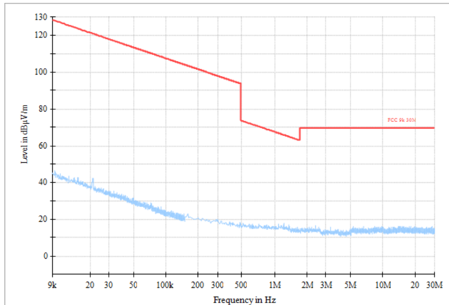
Fig. 120 Radiated Spurious Emission (All Channel, 9 kHz ~30 MHz)
