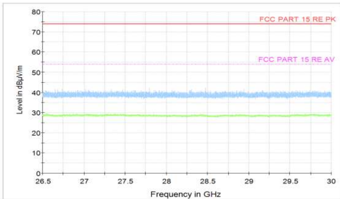
Figure A.45 Radiated Emission (Set.1, Camera Mode, 26.5GHz to 30GHz)
