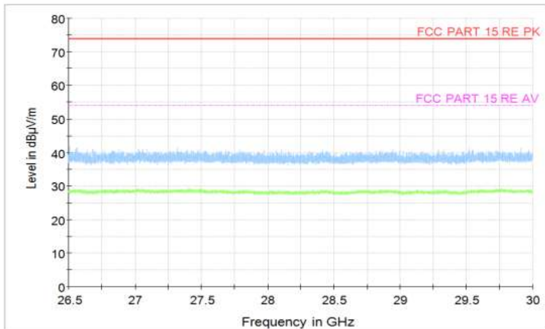
Figure A.30 Radiated Emission (Set.1, Charging and LTE Band 14 idle , 26.5GHz to 30GHz)
