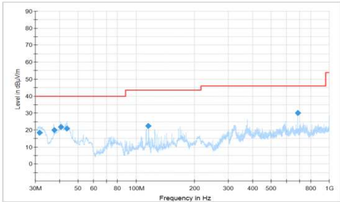
Figure A.16 Radiated Emission (Set.1, Charging and LTE Band 12 idle , 30MHz to 1GHz) Final_Result
