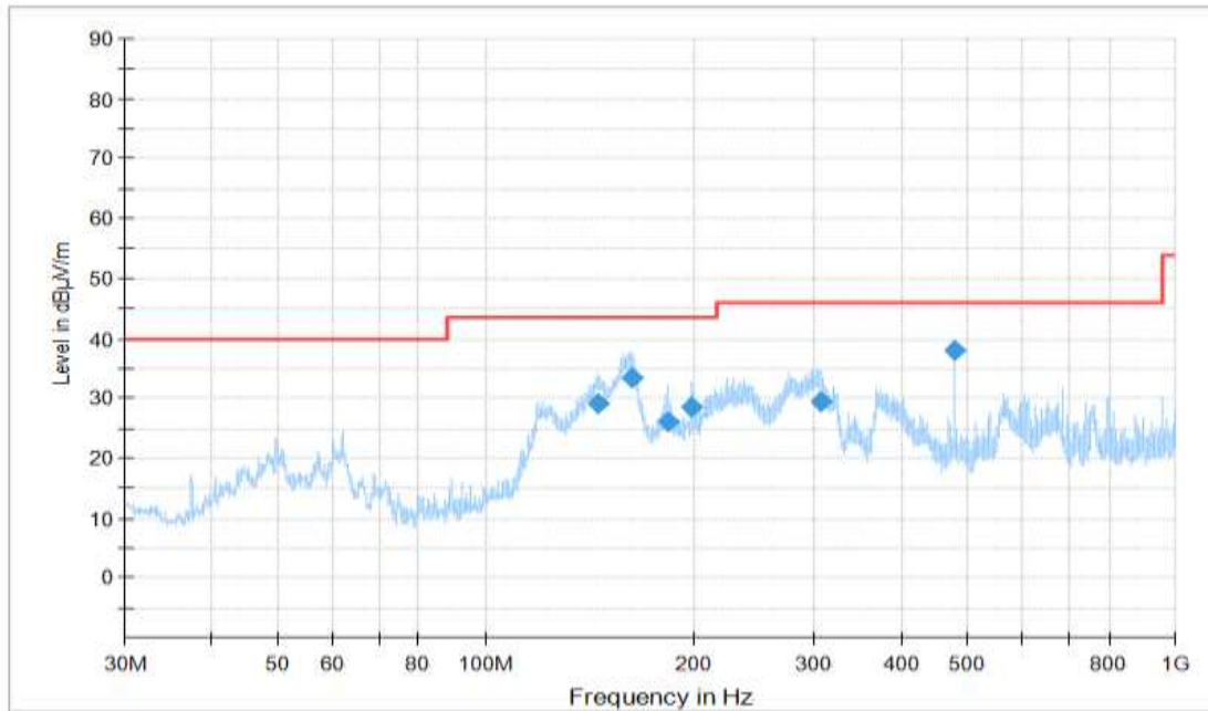
Figure A.56 Radiated Emission (Set.3, Data Transfer Mode: EUT To PC , 30MHz to 1GHz) Final_Result
