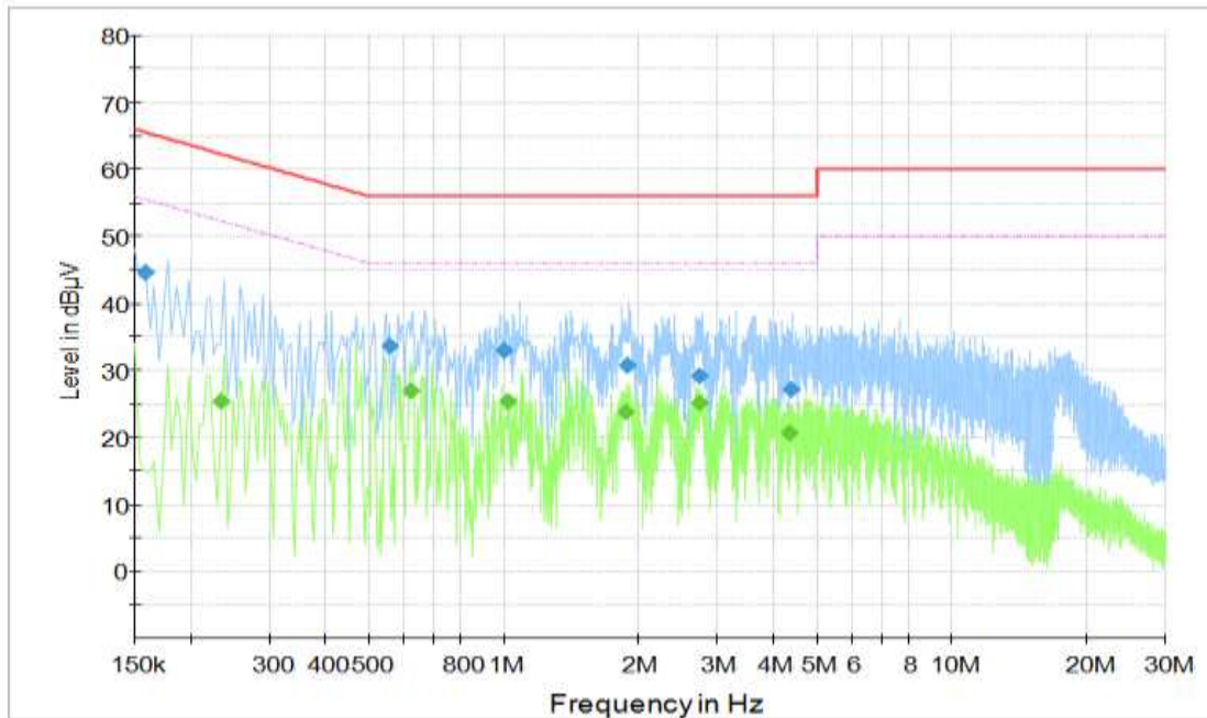
Figure B.9 Conducted Emission(Set.1, Video Player Mode)
