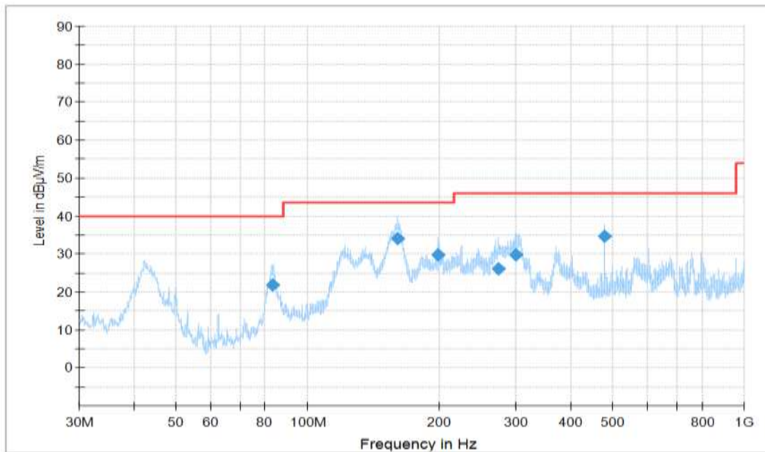
Figure A.71 Radiated Emission (Set.3, Data Transfer Mode: TF Card To PC , 30MHz to 1GHz)
