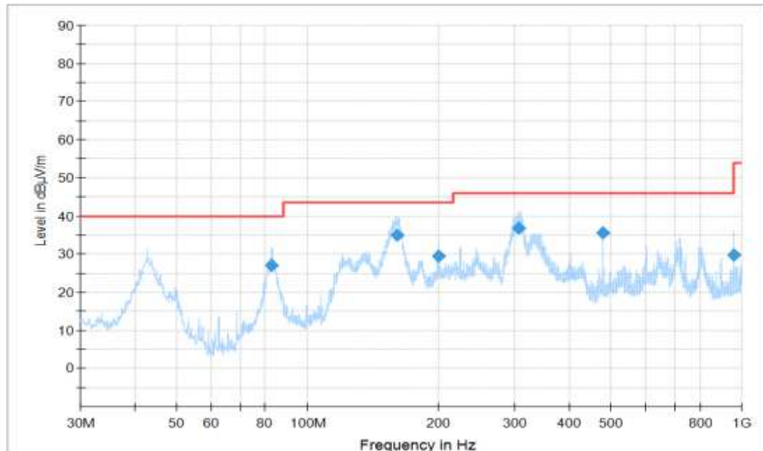
Figure A.66 Radiated Emission (Set.3, Data Transfer Mode: PC To TF Card , 30MHz to 1GHz)
