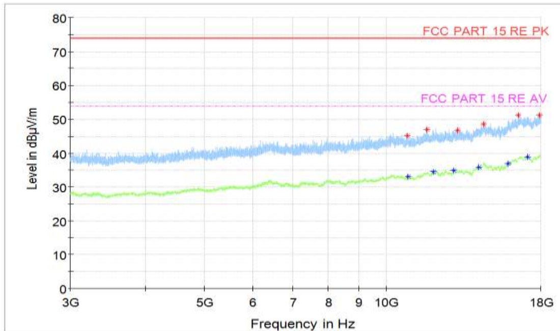
Figure A.68 Radiated Emission (Set.3, Data Transfer Mode: PC To EUT, 3GHz to 18GHz)
