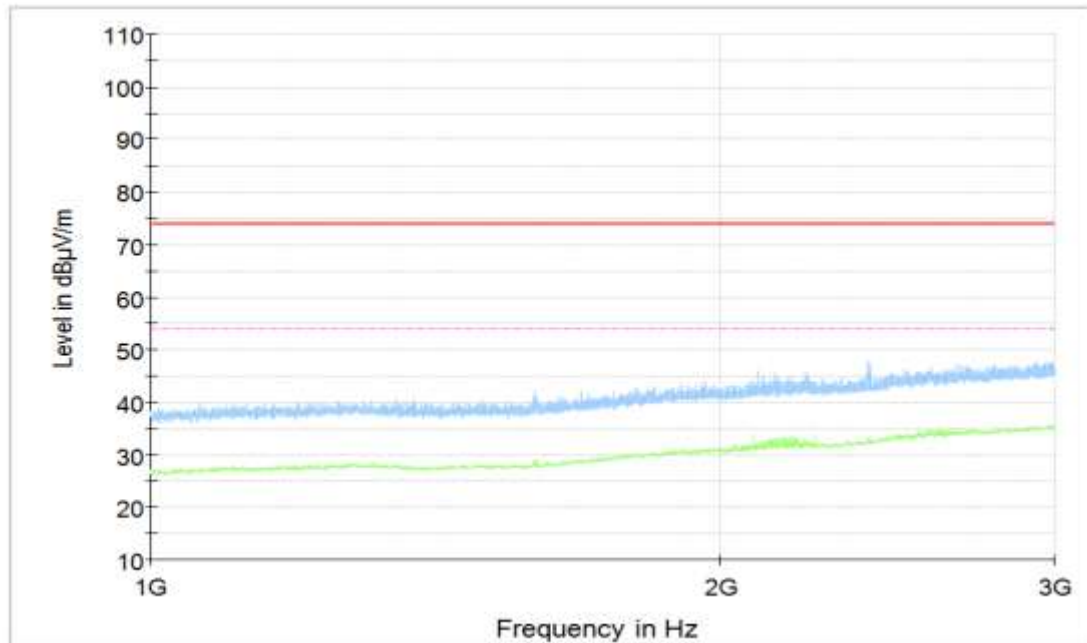
Figure A.72 Radiated Emission (Set.3, Data Transfer Mode: TF Card To PC, 1GHz to 3GHz)
