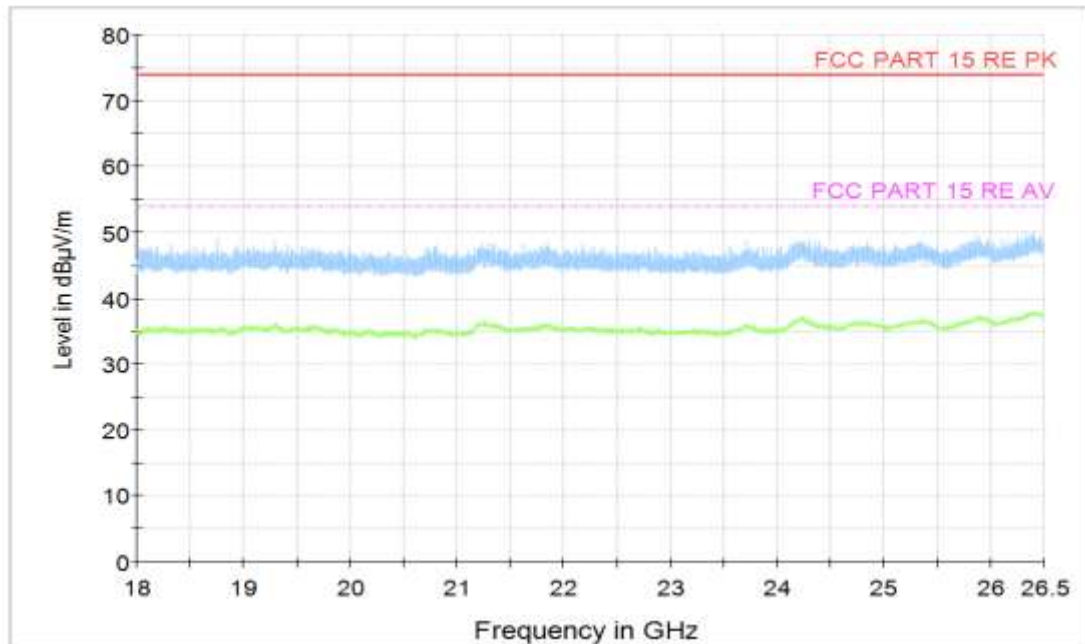
Figure A.49 Radiated Emission (Set.1, Video Player Mode, 18GHz to 26.5GHz)
