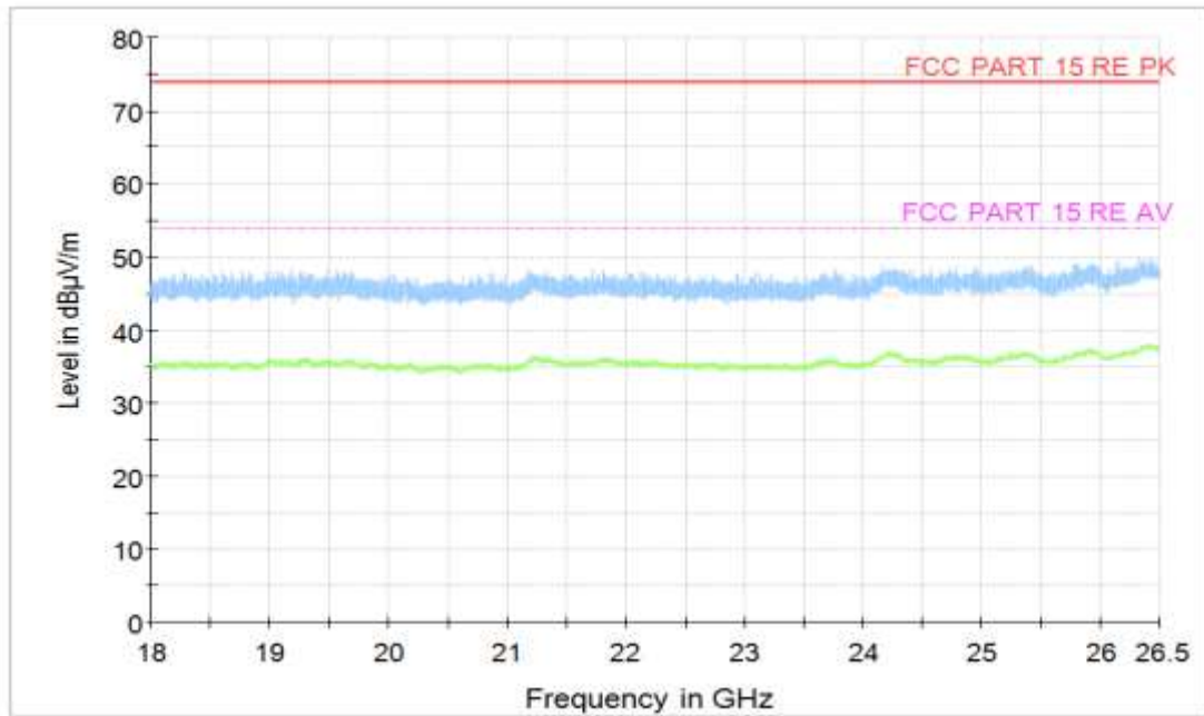
Figure A.59 Radiated Emission (Set.3, Data Transfer Mode: EUT To PC, 18GHz to 26.5GHz)
