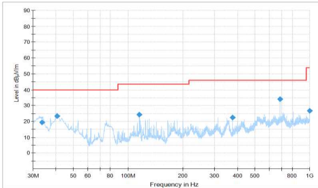
Figure A.46 Radiated Emission (Set.1, Video Player Mode , 30MHz to 1GHz)
