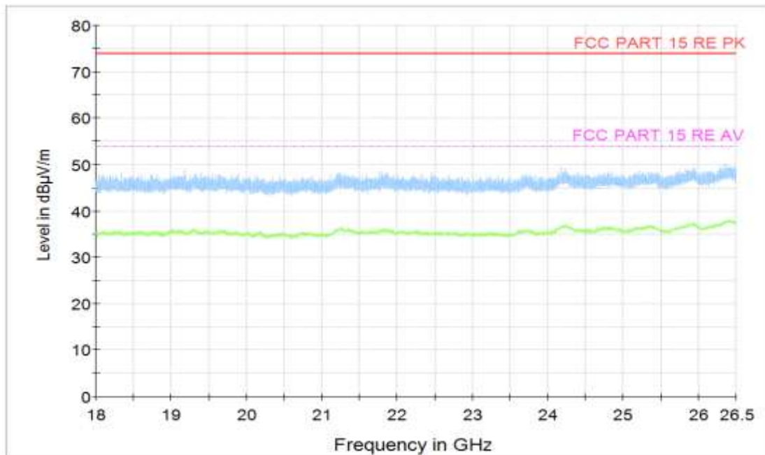
Figure A.69 Radiated Emission (Set.3, Data Transfer Mode: PC To TF Card, 18GHz to 26.5GHz)
