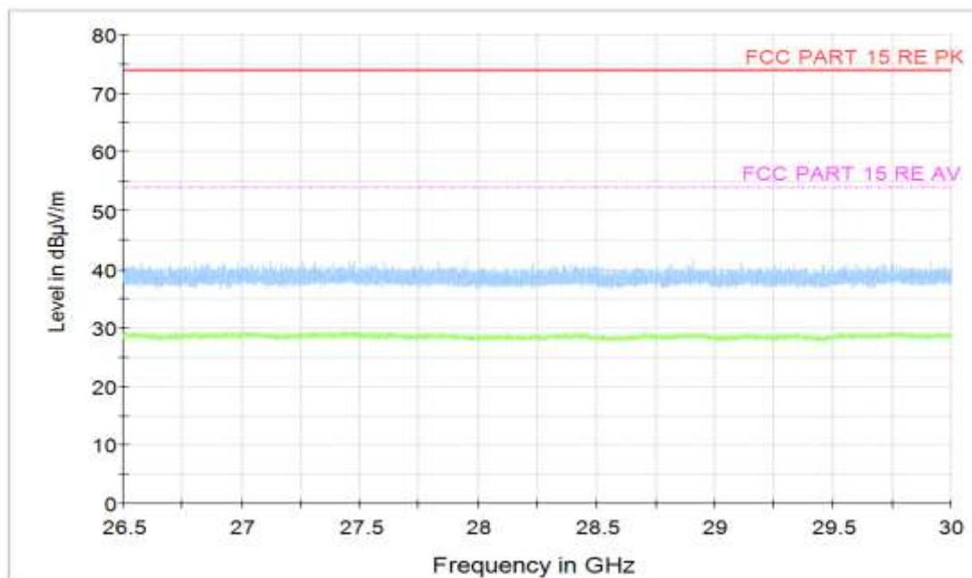
Figure A.5 Radiated Emission (Set.1, Charging and GSM850MHz idle , 26.5GHz to 30GHz)
