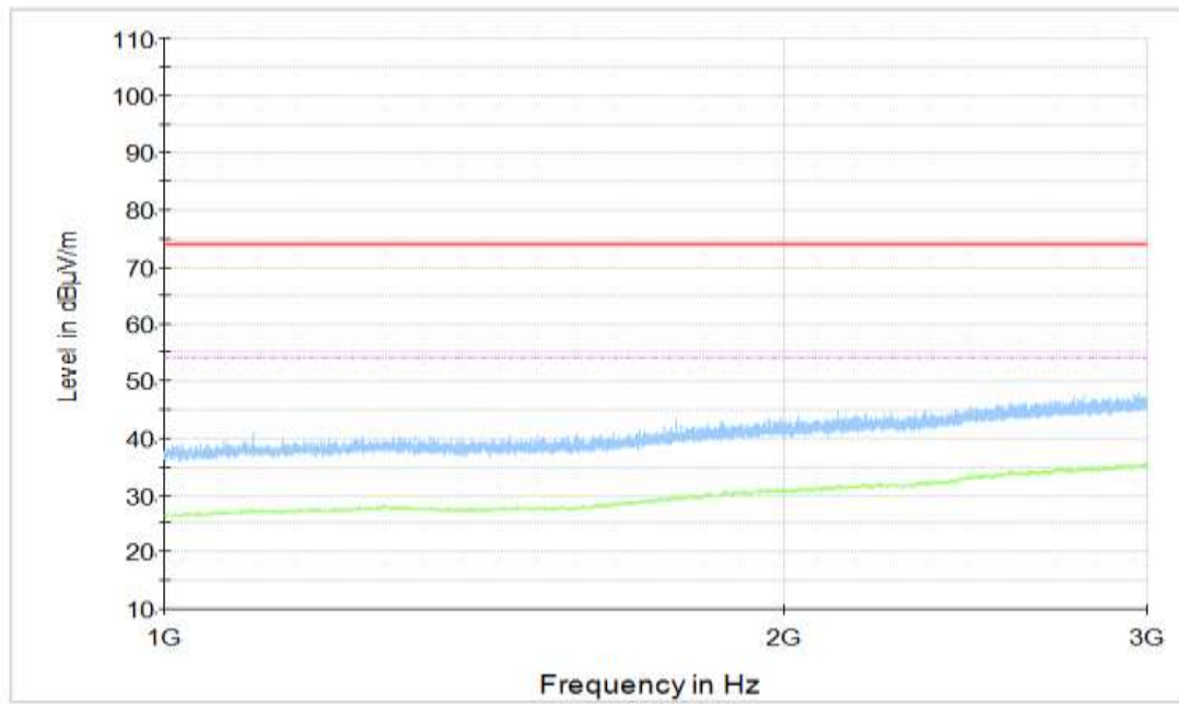
Figure A.42 Radiated Emission (Set.1, Camera Mode , 1GHz to 3GHz)
