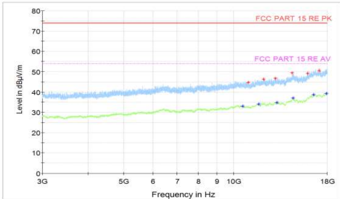
Figure A.43 Radiated Emission (Set.1, Camera Mode, 3GHz to 18GHz)
