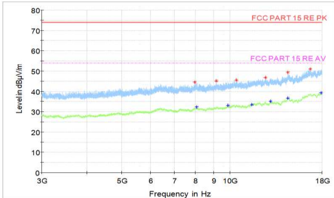
Figure A.28 Radiated Emission (Set.1, Charging and LTE Band 14 idle, 3GHz to 18GHz)
