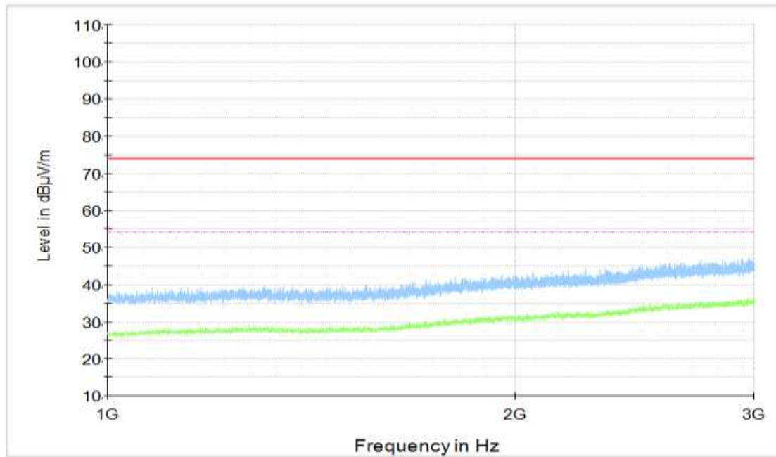
Figure A.27 Radiated Emission (Set.1, Charging and LTE Band 14 idle , 1GHz to 3GHz)
