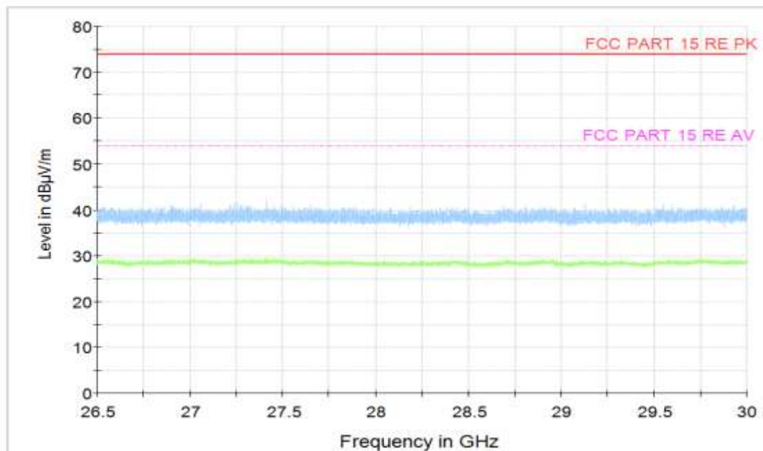
Figure A.15 Radiated Emission (Set.1, Charging and LTE Band 5 idle , 26.5GHz to 30GHz)
