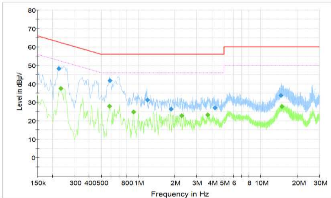
Figure B.4 Conducted Emission(Set.3, Data Transfer Mode: EUT To PC)
