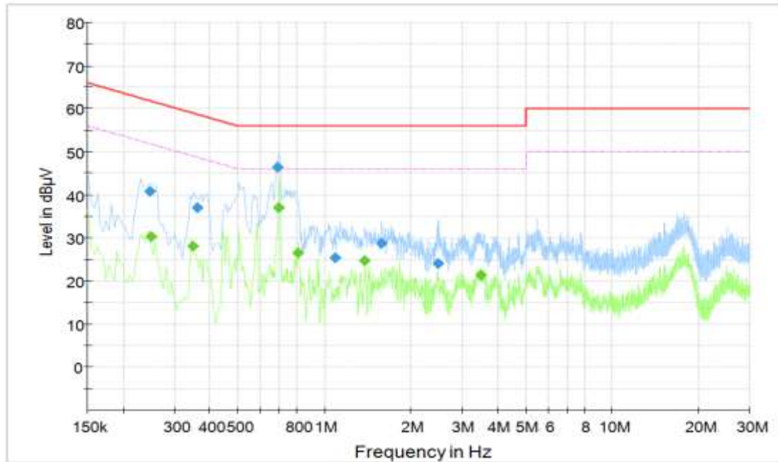
Figure B.14 Conducted Emission(Set.3, Data Transfer Mode: TF Card To PC)
