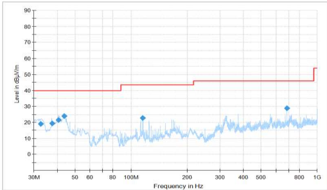
Figure A.21 Radiated Emission (Set.1, Charging and LTE Band 13 idle , 30MHz to 1GHz) Final_Result
