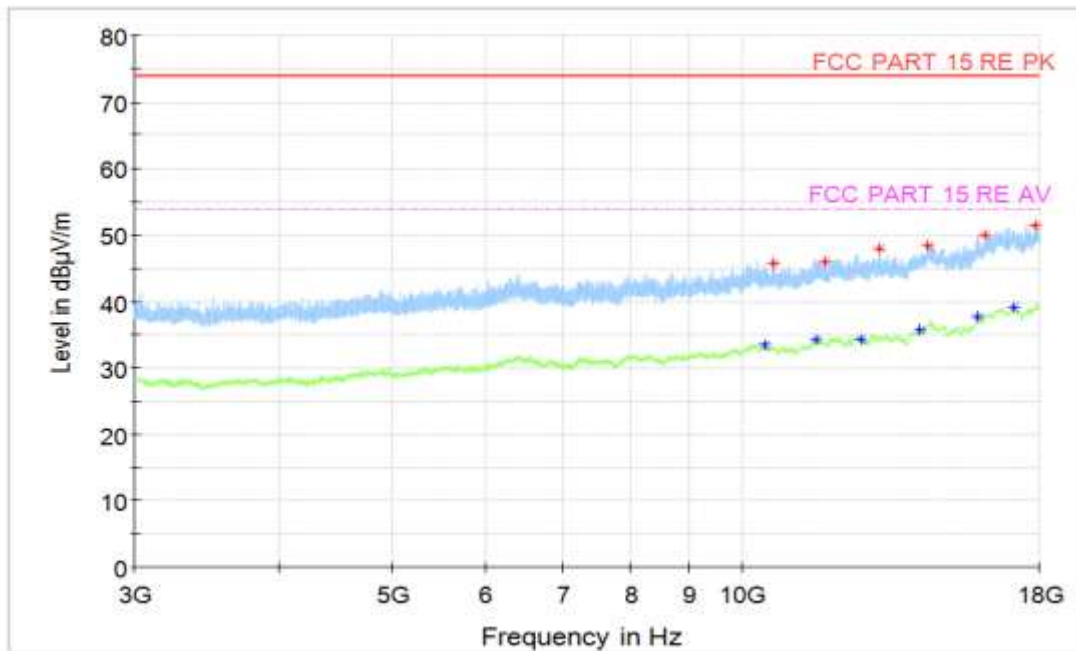
Figure A.73 Radiated Emission (Set.3, Data Transfer Mode: TF Card To PC, 3GHz to 18GHz)
