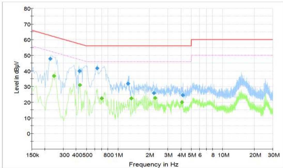
Figure B.6 Conducted Emission(Set.3, Data Transfer Mode: PC To TF Card)
