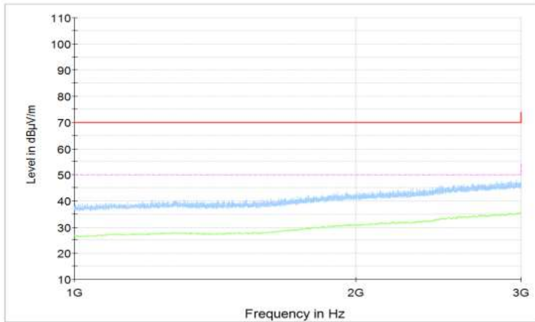
Figure A.52 Radiated Emission (Set.2, Video Player Mode , 1GHz to 3GHz)
