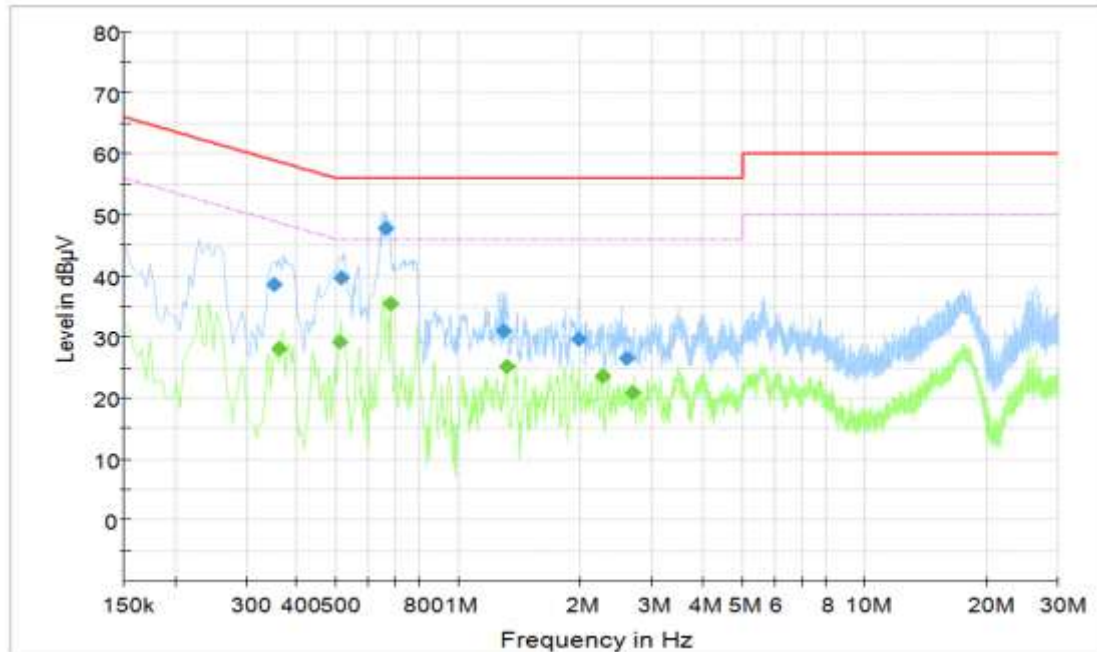
Figure B.12 Conducted Emission(Set.3, Data Transfer Mode: PC To EUT)
