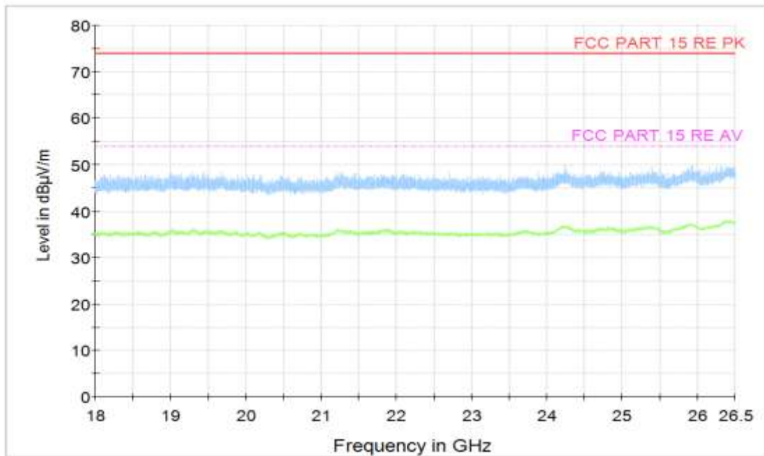
Figure A.39 Radiated Emission (Set.1, Charging and LTE Band 26 idle , 18GHz to 26.5GHz)
