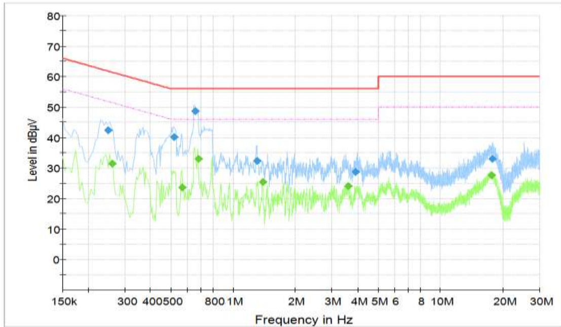
Figure B.11 Conducted Emission(Set.3, Data Transfer Mode: EUT To PC)
