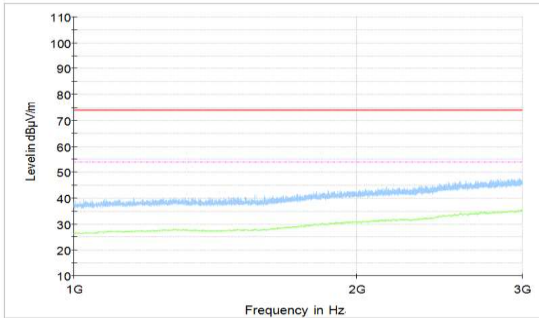
Figure A.47 Radiated Emission (Set.1, Video Player Mode , 1GHz to 3GHz)
