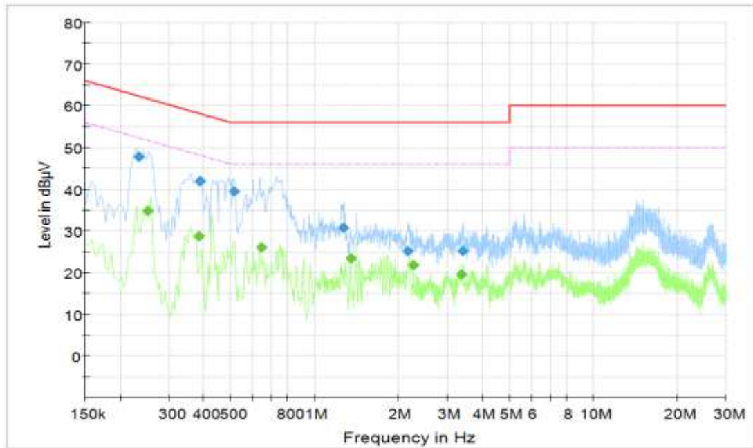
Figure B.7 Conducted Emission(Set.3, Data Transfer Mode: TF Card To PC)
