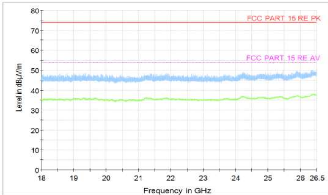
Figure A.54 Radiated Emission (Set.2, Video Player Mode, 18GHz to 26.5GHz)
