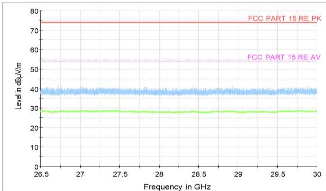
Figure A.40 Radiated Emission (Set.1, Charging and LTE Band 26 idle , 26.5GHz to 30GHz)
