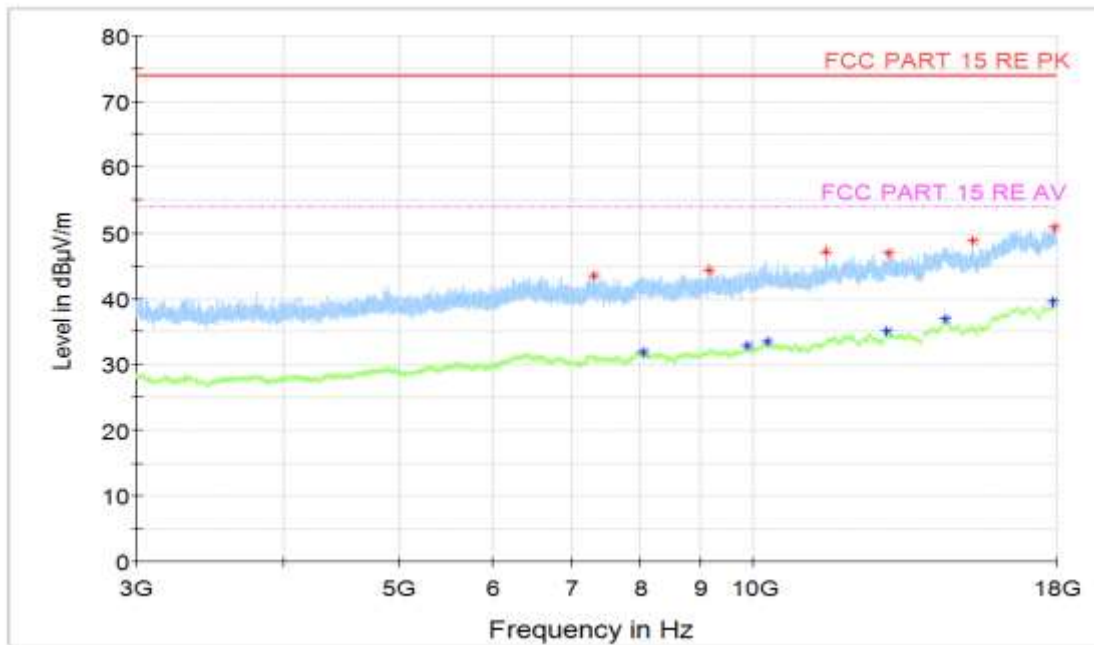
Figure A.23 Radiated Emission (Set.1, Charging and LTE Band 13 idle, 3GHz to 18GHz)
