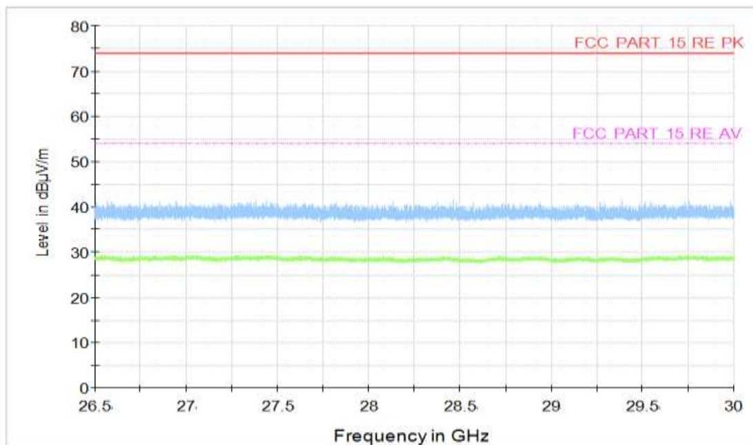
Figure A.50 Radiated Emission (Set.1, Video Player Mode, 26.5GHz to 30GHz)
