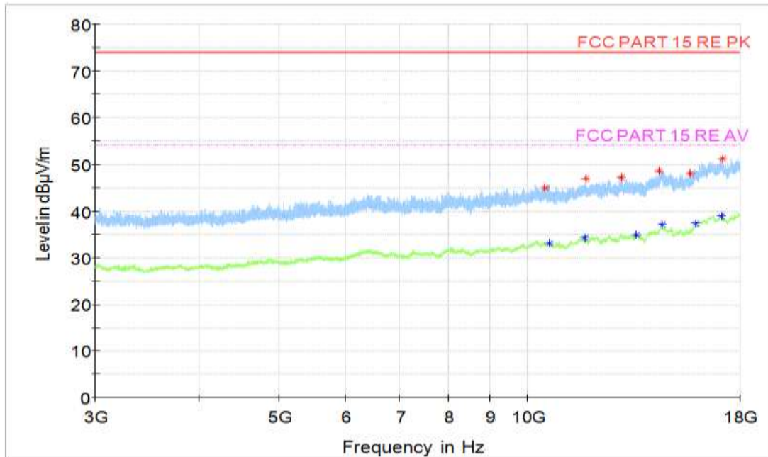
Figure A.48 Radiated Emission (Set.1, Video Player Mode, 3GHz to 18GHz)
