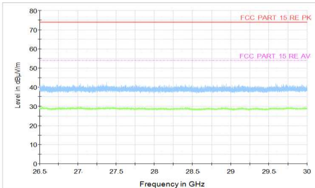
Figure A.70 Radiated Emission (Set.3, Data Transfer Mode: PC To TF Card, 26.5GHz to 30GHz)
