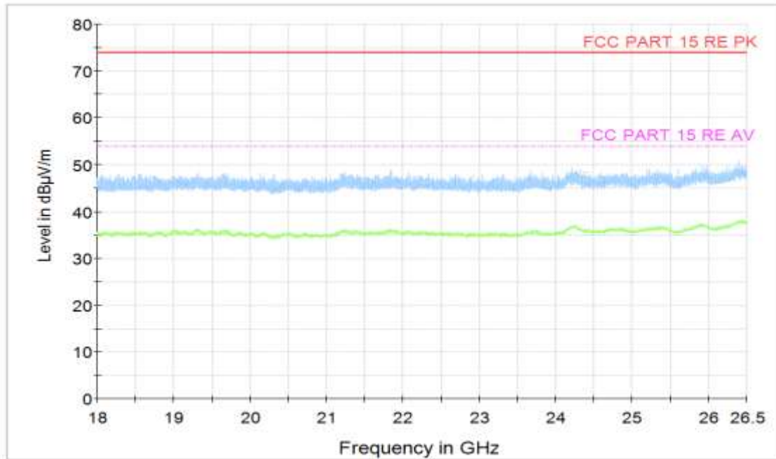
Figure A.19 Radiated Emission (Set.1, Charging and LTE Band 12 idle , 18GHz to 26.5GHz)
