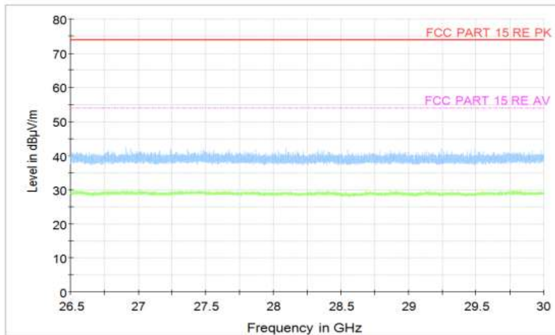
Figure A.75 Radiated Emission (Set.3, Data Transfer Mode: TF Card To PC, 26.5GHz to 30GHz)
