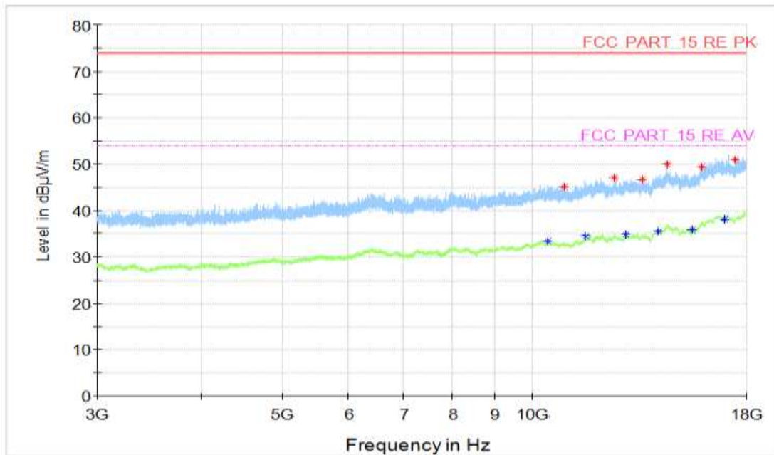
Figure A.58 Radiated Emission (Set.3, Data Transfer Mode: EUT To PC, 3GHz to 18GHz)
