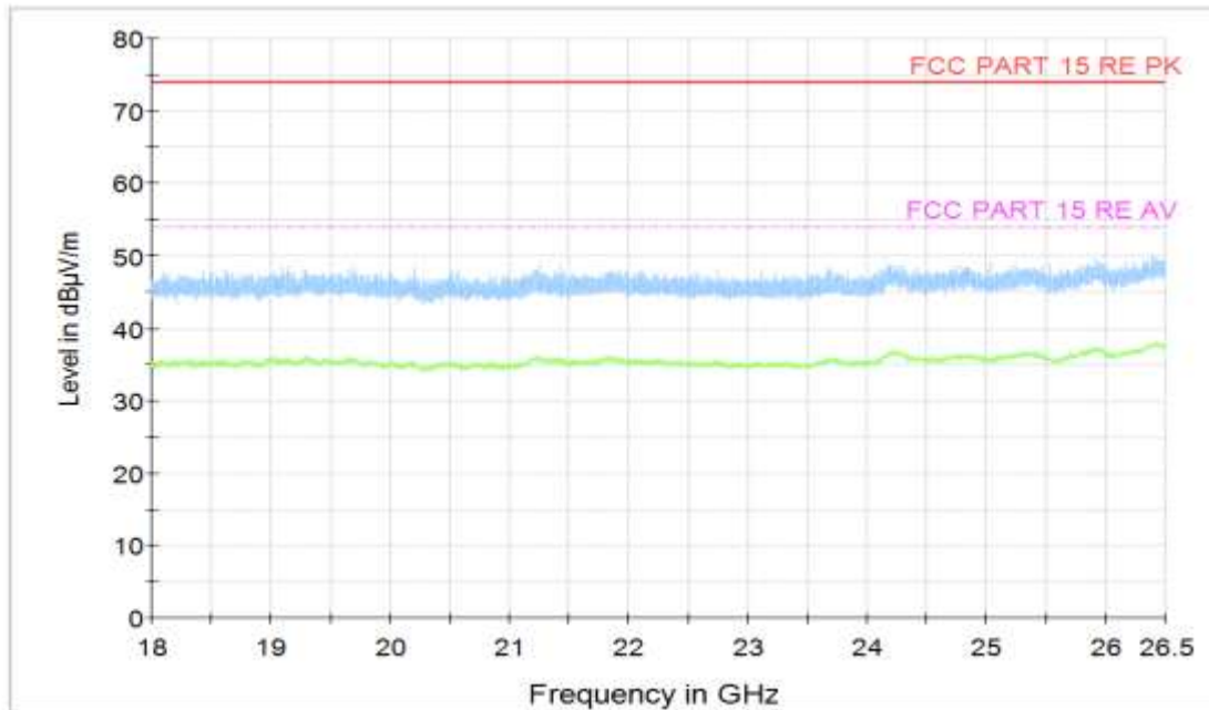
Figure A.29 Radiated Emission (Set.1, Charging and LTE Band 14 idle , 18GHz to 26.5GHz)
