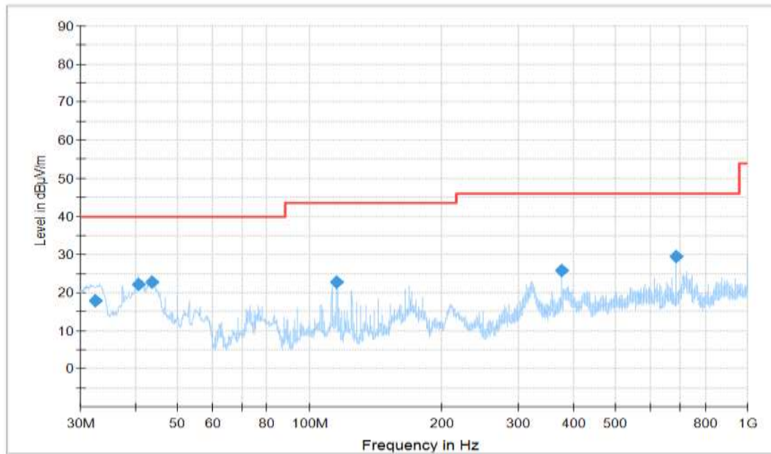
Figure A.26 Radiated Emission (Set.1, Charging and LTE Band 14 idle , 30MHz to 1GHz) Final_Result
