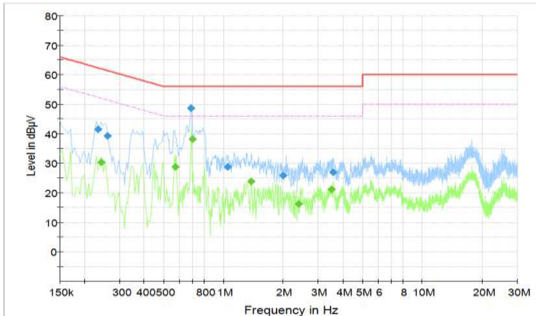
Figure B.13 Conducted Emission(Set.3, Data Transfer Mode: PC To TF Card)
