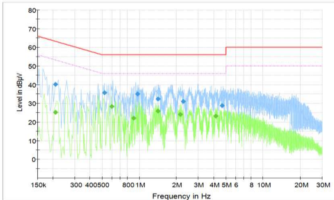
Figure B.10 Conducted Emission(Set.2, Camera Mode)
