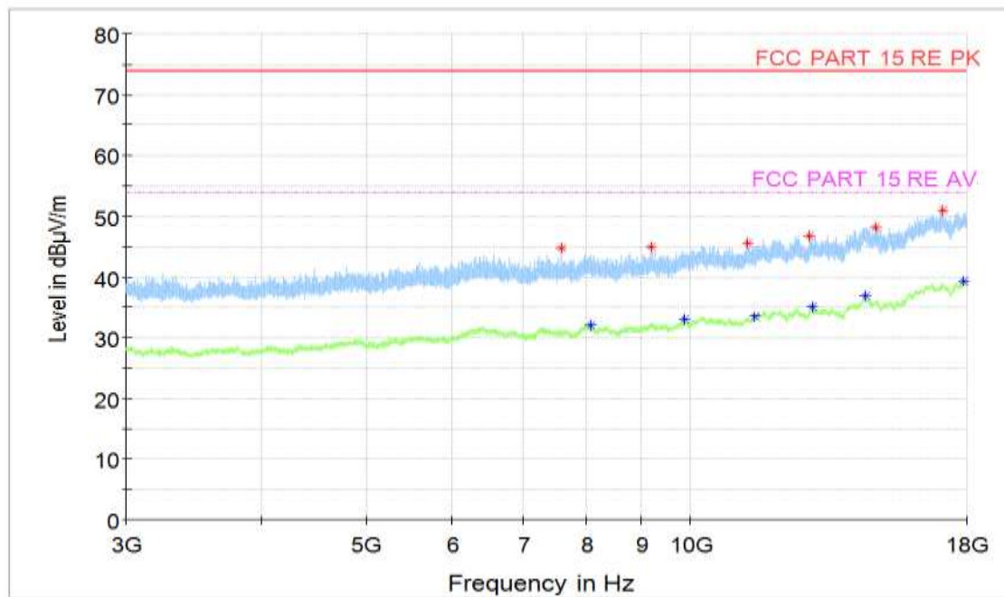
Figure A.38 Radiated Emission (Set.1, Charging and LTE Band 26 idle, 3GHz to 18GHz)
