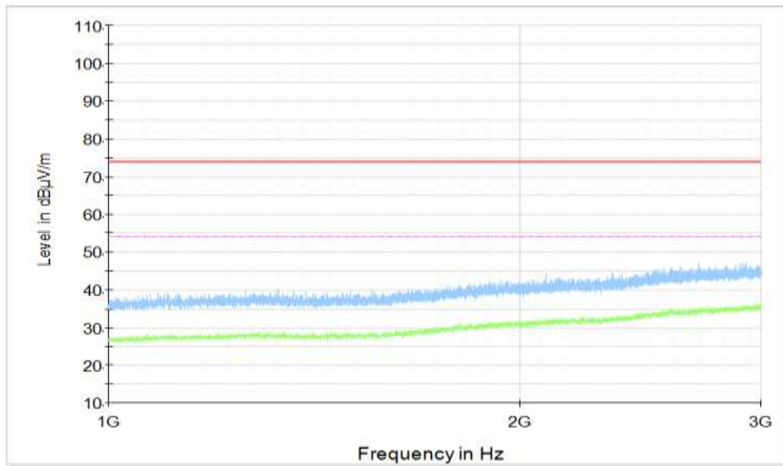
Figure A.17 Radiated Emission (Set.1, Charging and LTE Band 12 idle , 1GHz to 3GHz)
