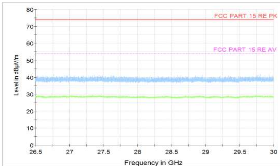
Figure A.55 Radiated Emission (Set.2, Video Player Mode, 26.5GHz to 30GHz)
