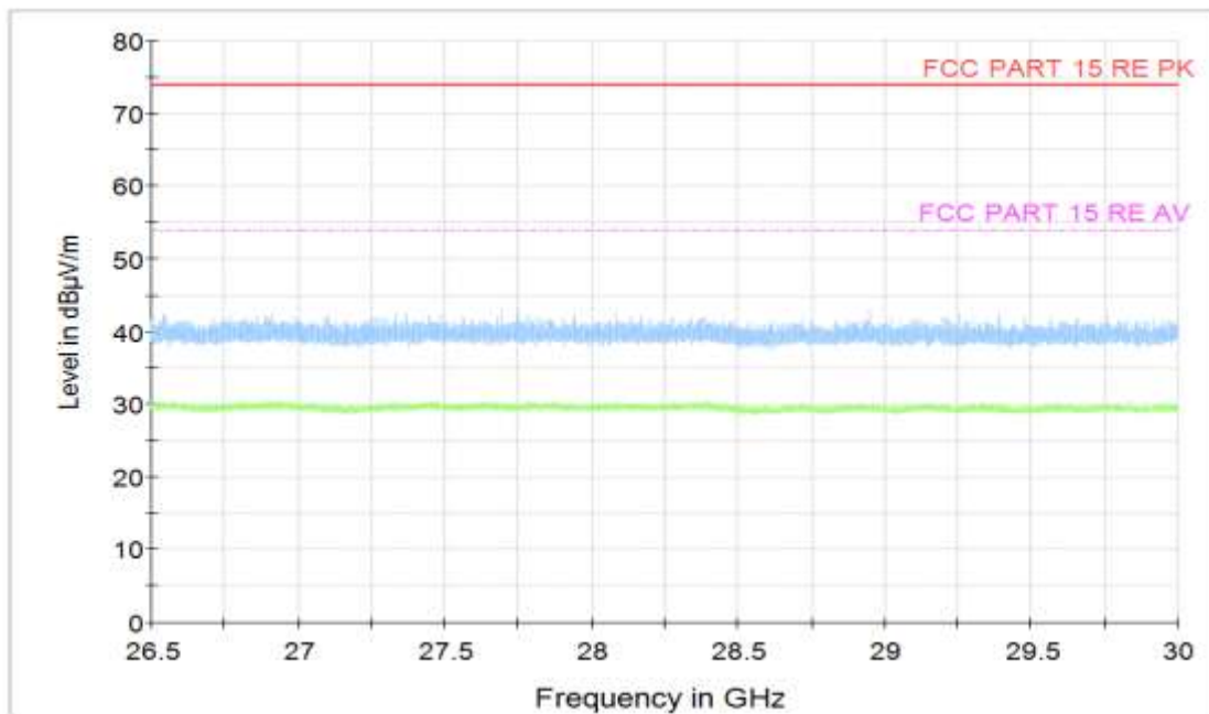
Figure A.60 Radiated Emission (Set.3, Data Transfer Mode: EUT To PC, 26.5GHz to 30GHz)
