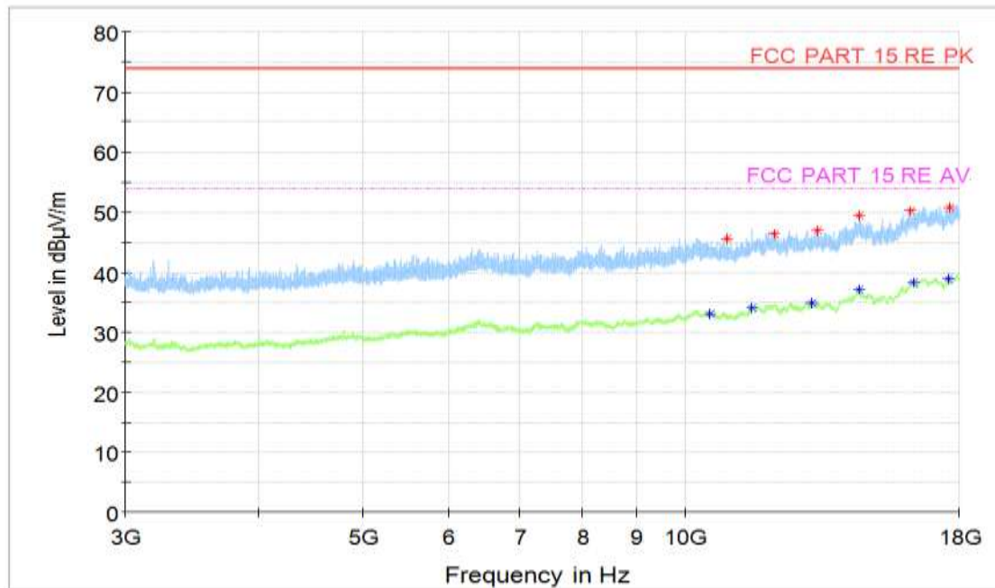
Figure A.63 Radiated Emission (Set.3, Data Transfer Mode: PC To EUT, 3GHz to 18GHz)
