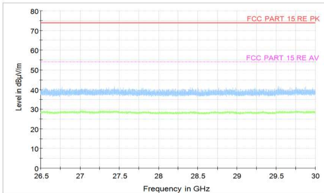
Figure A.20 Radiated Emission (Set.1, Charging and LTE Band 12 idle , 26.5GHz to 30GHz)
