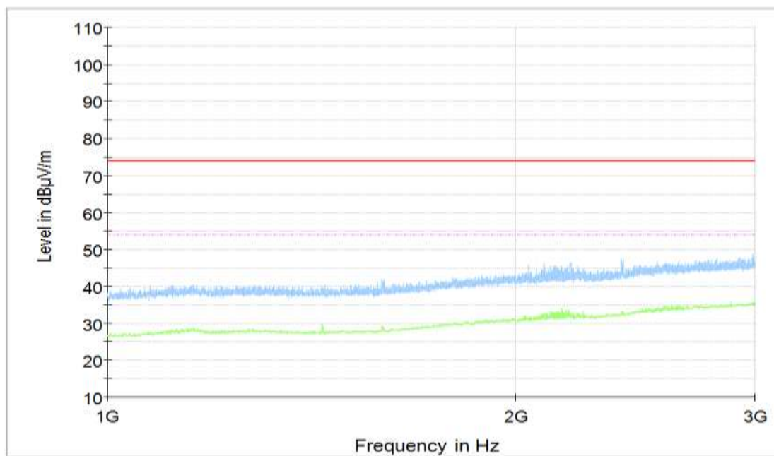
Figure A.62 Radiated Emission (Set.3, Data Transfer Mode: PC To EUT, 1GHz to 3GHz)
