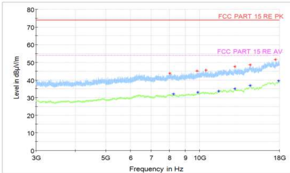
Figure A.33 Radiated Emission (Set.1, Charging and LTE Band 17 idle, 3GHz to 18GHz)
