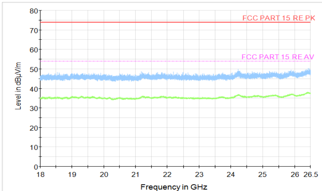
Figure A.24 Radiated Emission (Set.1, Charging and LTE Band 13 idle , 18GHz to 26.5GHz)
