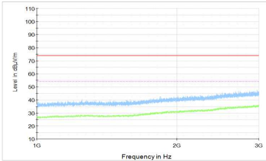
Figure A.32 Radiated Emission (Set.1, Charging and LTE Band 17 idle , 1GHz to 3GHz)
