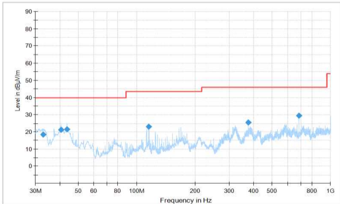
Figure A.31 Radiated Emission (Set.1, Charging and LTE Band 17 idle , 30MHz to 1GHz) Final_Result
