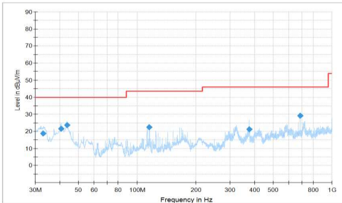
Figure A.36 Radiated Emission (Set.1, Charging and LTE Band 26 idle , 30MHz to 1GHz) Final_Result
