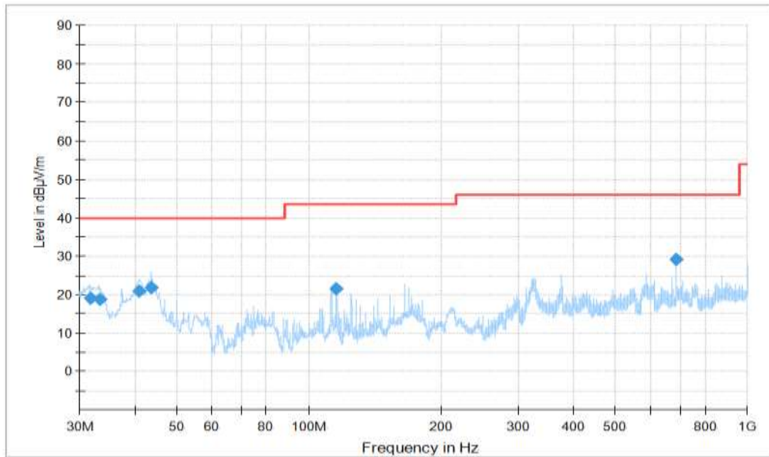
Figure A.11 Radiated Emission (Set.1, Charging and LTE Band 5 idle , 30MHz to 1GHz) Final_Result
