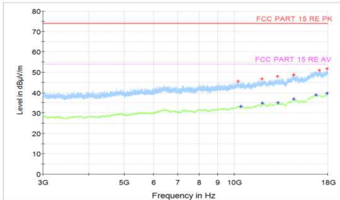
Figure A.53 Radiated Emission (Set.2, Video Player Mode, 3GHz to 18GHz)
