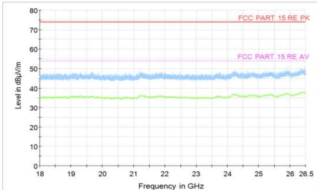
Figure A.74 Radiated Emission (Set.3, Data Transfer Mode: TF Card To PC, 18GHz to 26.5GHz)
