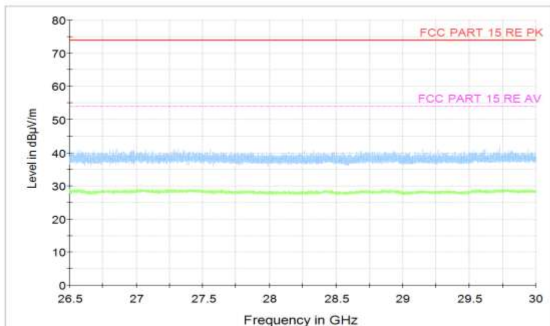
Figure A.35 Radiated Emission (Set.1, Charging and LTE Band 17 idle , 26.5GHz to 30GHz)
