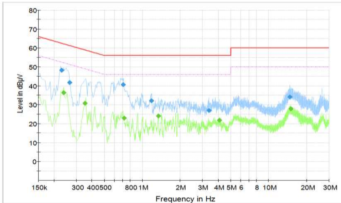
Figure B.5 Conducted Emission(Set.3, Data Transfer Mode: PC To EUT)
