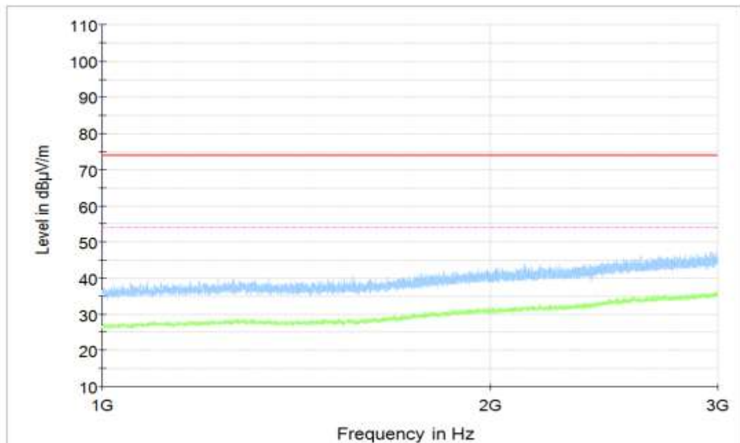
Figure A.22 Radiated Emission (Set.1, Charging and LTE Band 13 idle , 1GHz to 3GHz)
