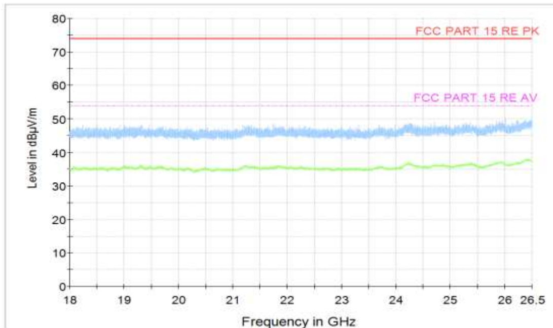
Figure A.34 Radiated Emission (Set.1, Charging and LTE Band 17 idle , 18GHz to 26.5GHz)
