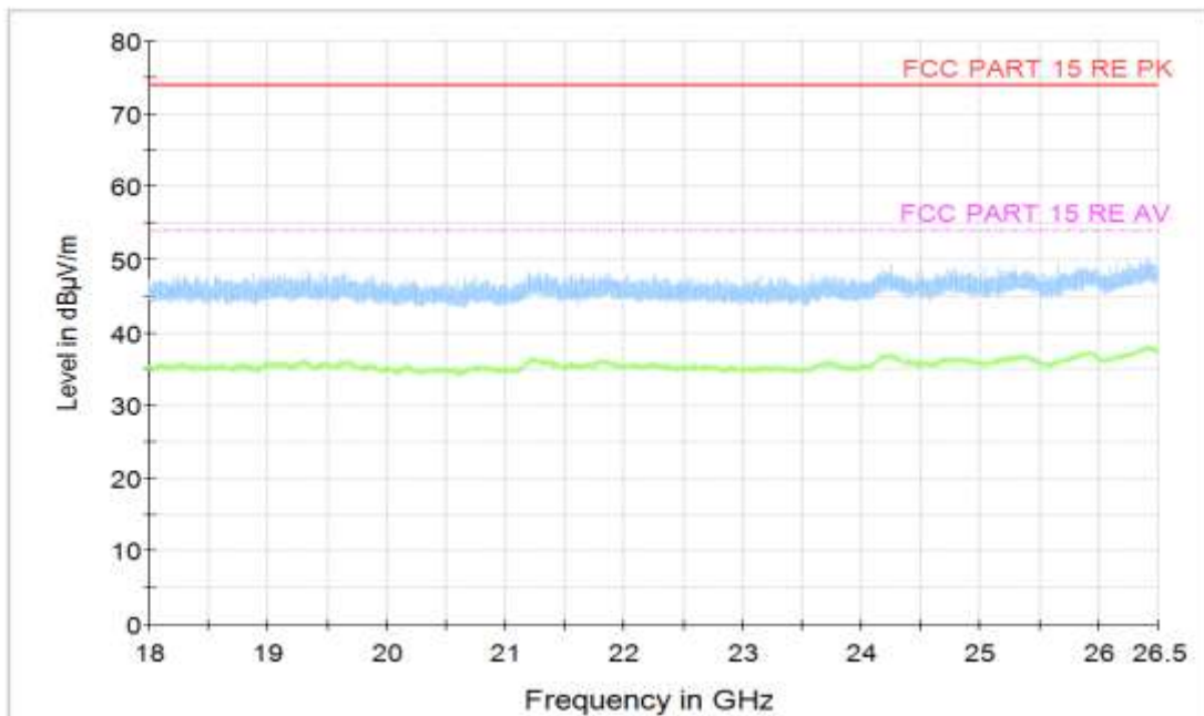
Figure A.44 Radiated Emission (Set.1, Camera Mode , 18GHz to 26.5GHz)
