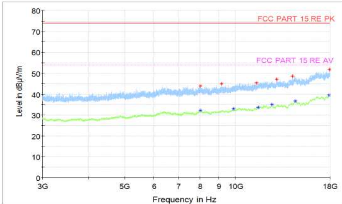
Figure A.18 Radiated Emission (Set.1, Charging and LTE Band 12 idle, 3GHz to 18GHz)
