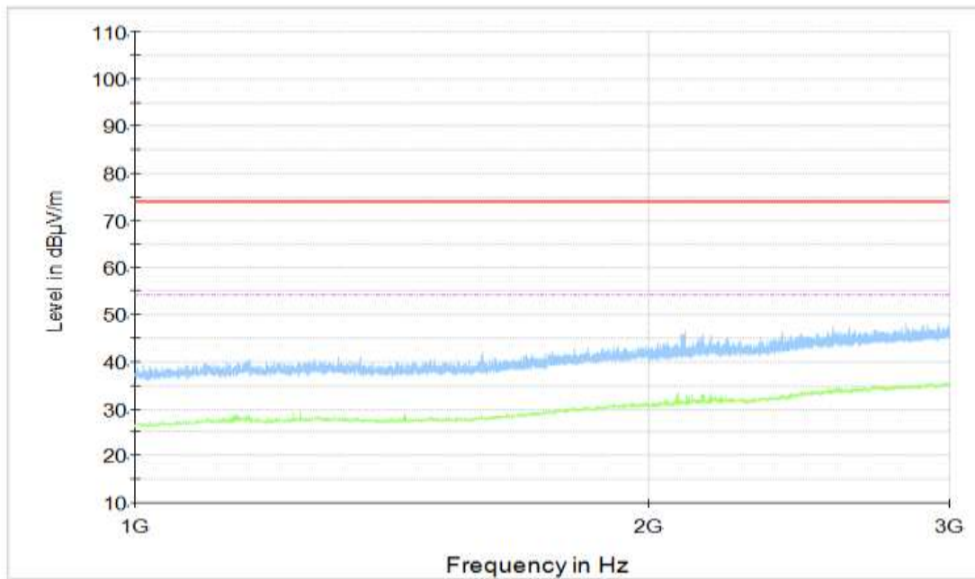
Figure A.67 Radiated Emission (Set.3, Data Transfer Mode: PC To TF Card, 1GHz to 3GHz)
