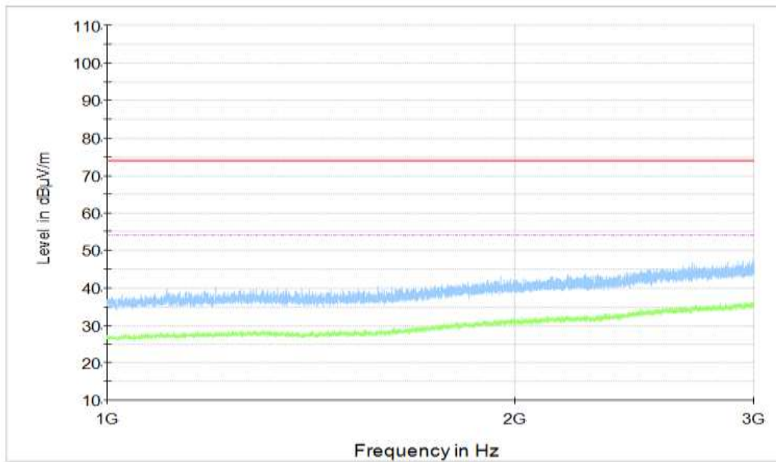
Figure A.37 Radiated Emission (Set.1, Charging and LTE Band 26 idle , 1GHz to 3GHz)
