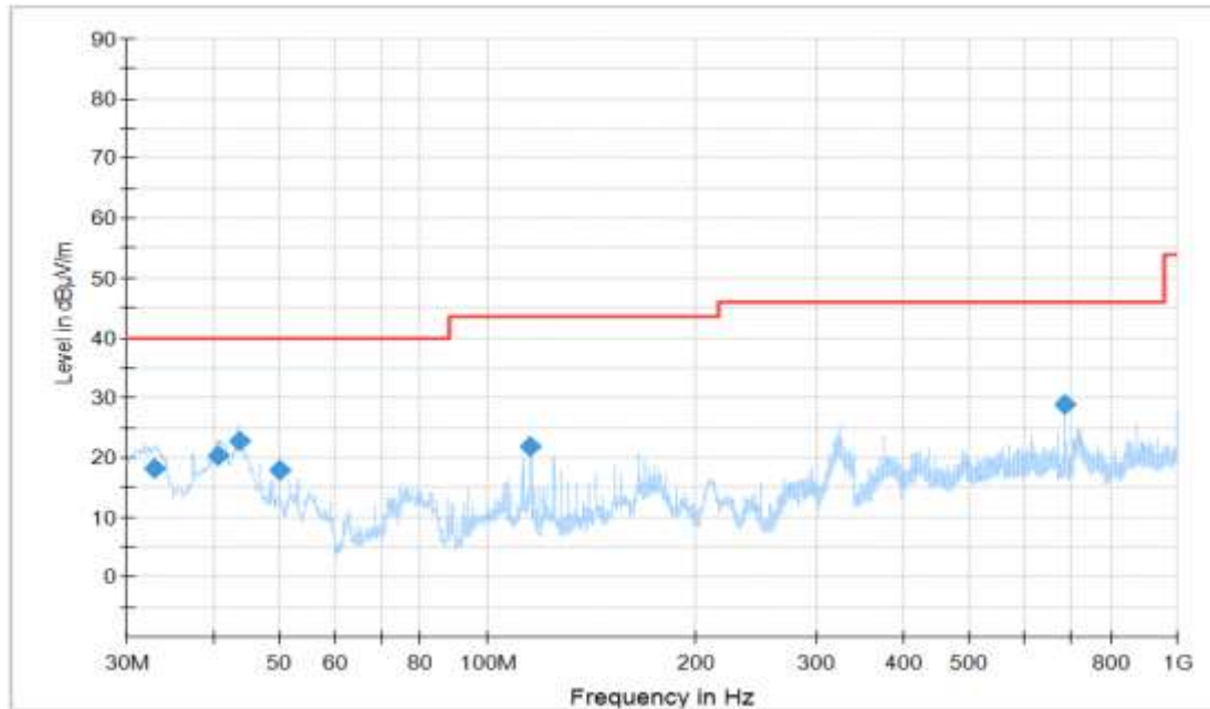
Figure A.6 Radiated Emission (Set.1, Charging and WCDMA Band 5 idle , 30MHz to 1GHz) Final_Result
