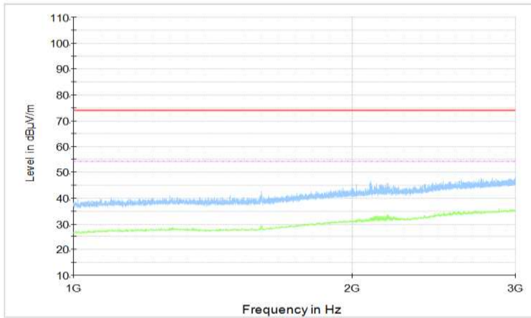
Figure A.57 Radiated Emission (Set.3, Data Transfer Mode: EUT To PC, 1GHz to 3GHz)
