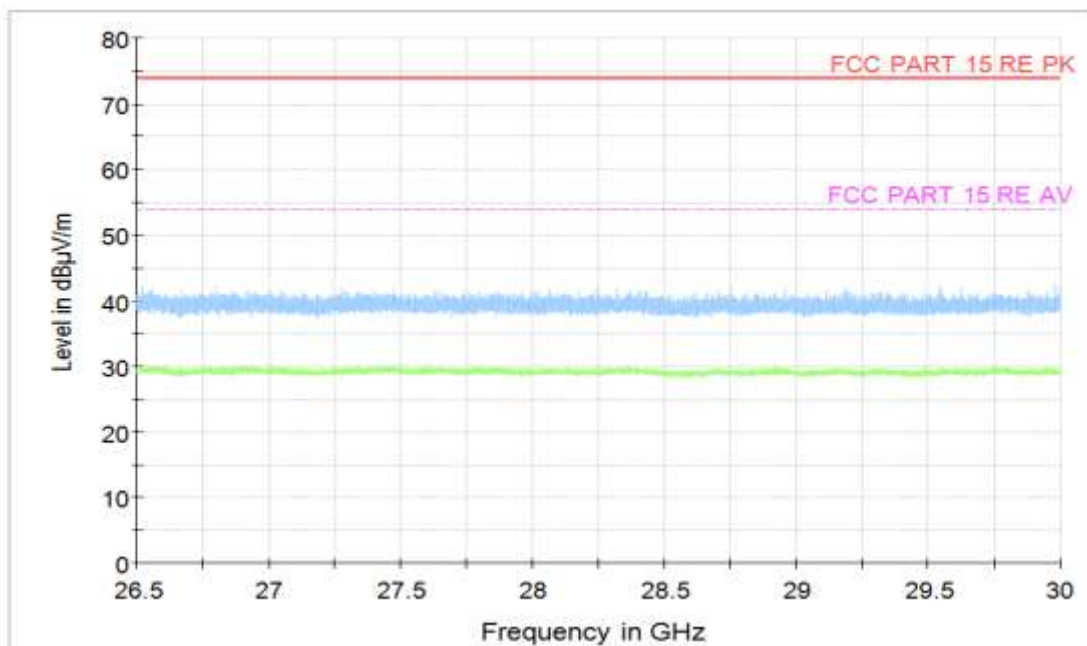
Figure A.65 Radiated Emission (Set.3, Data Transfer Mode: PC To EUT, 26.5GHz to 30GHz)
