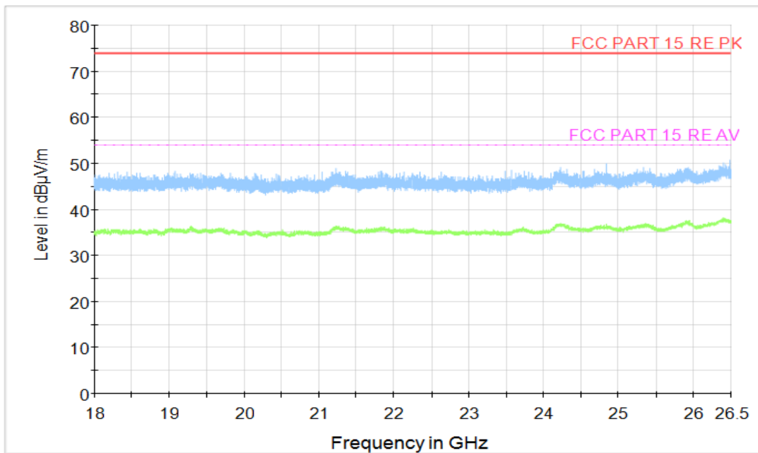
Figure A.64 Radiated Emission (Set.3, Data Transfer Mode: PC To EUT, 18GHz to 26.5GHz)
