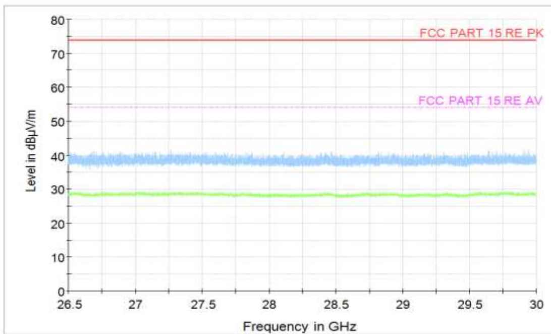
Figure A.25 Radiated Emission (Set.1, Charging and LTE Band 13 idle , 26.5GHz to 30GHz)
