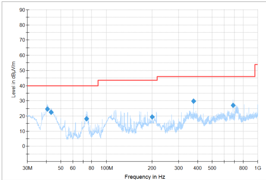
Figure A.51 Radiated Emission (Set.2, Video Player Mode , 30MHz to 1GHz)
