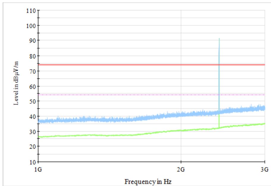
Fig. 50 Radiated Spurious Emission ( \pi/4 DQPSK, Ch0, 1GHz ~ 3GHz)
