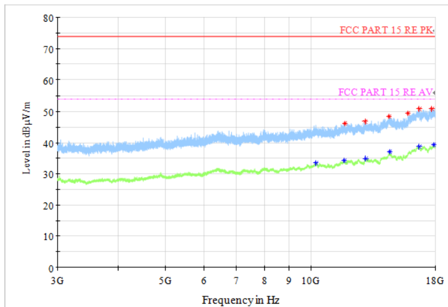
Fig.63 Radiated Spurious Emission (802.11n HT40, CH9, 3GHz-18GHz)
