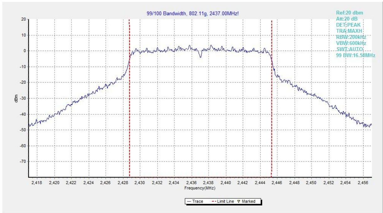
Fig.75 99% Occupied Bandwidth (802.11g, CH 6)
