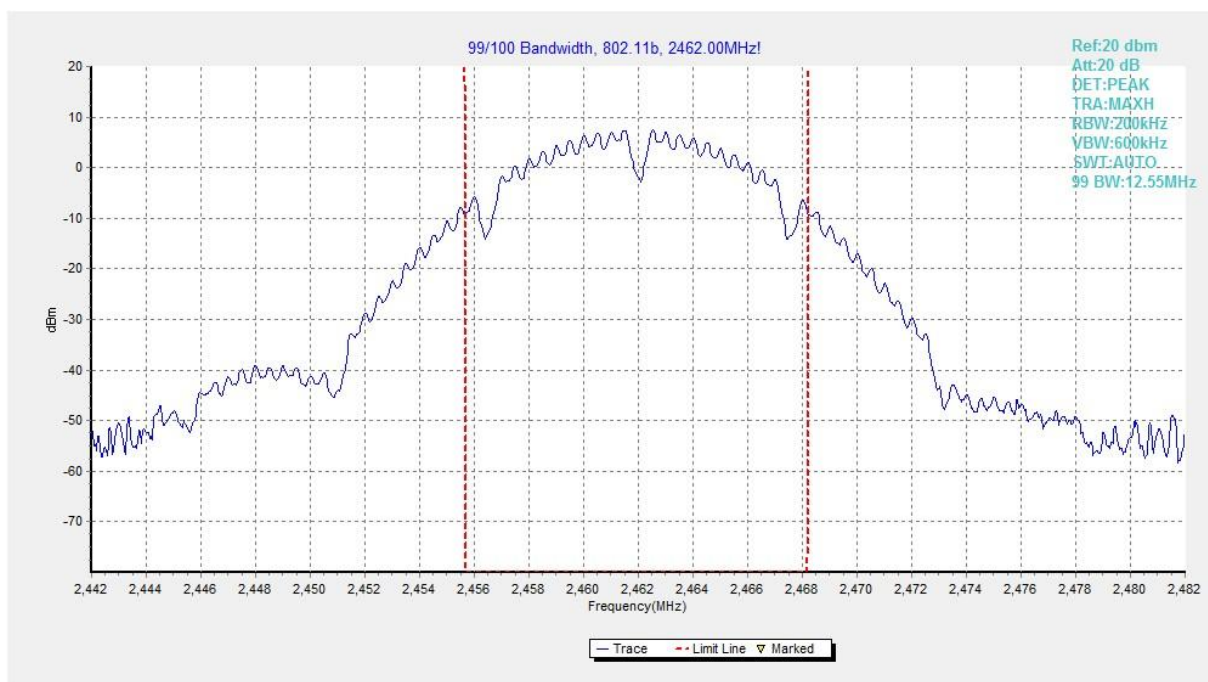
Fig.73 99% Occupied Bandwidth (802.11b, CH 11)
