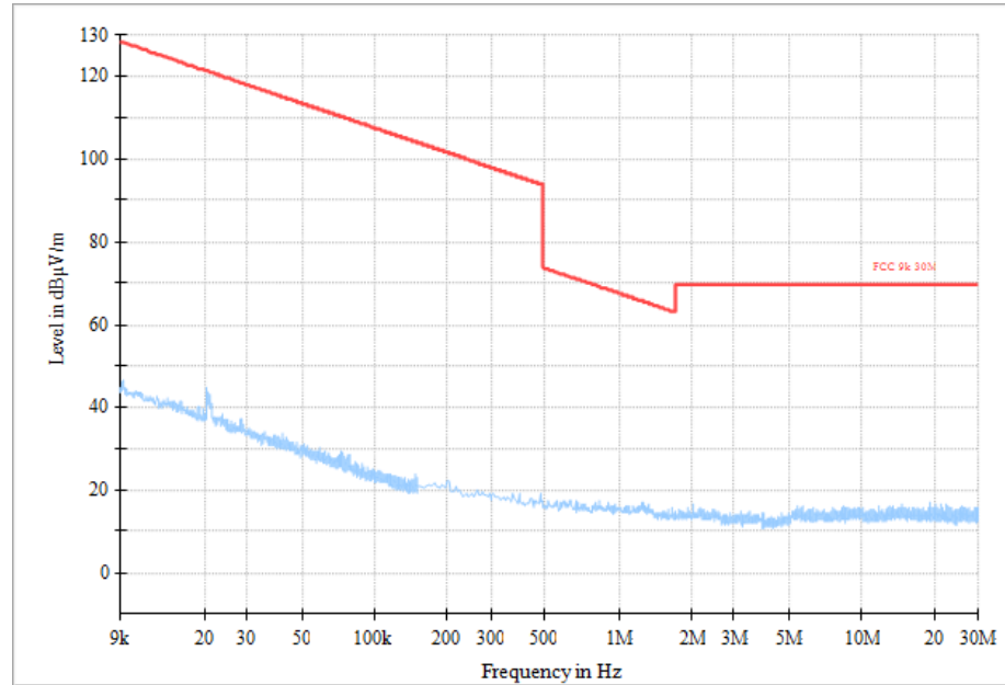
Fig.66 Radiated Spurious Emission (All Channels, 9KHz-30MHz)
