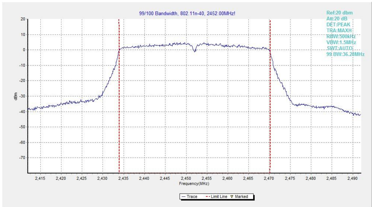
Fig.82 99% Occupied Bandwidth (802.11n HT40, CH 9)
