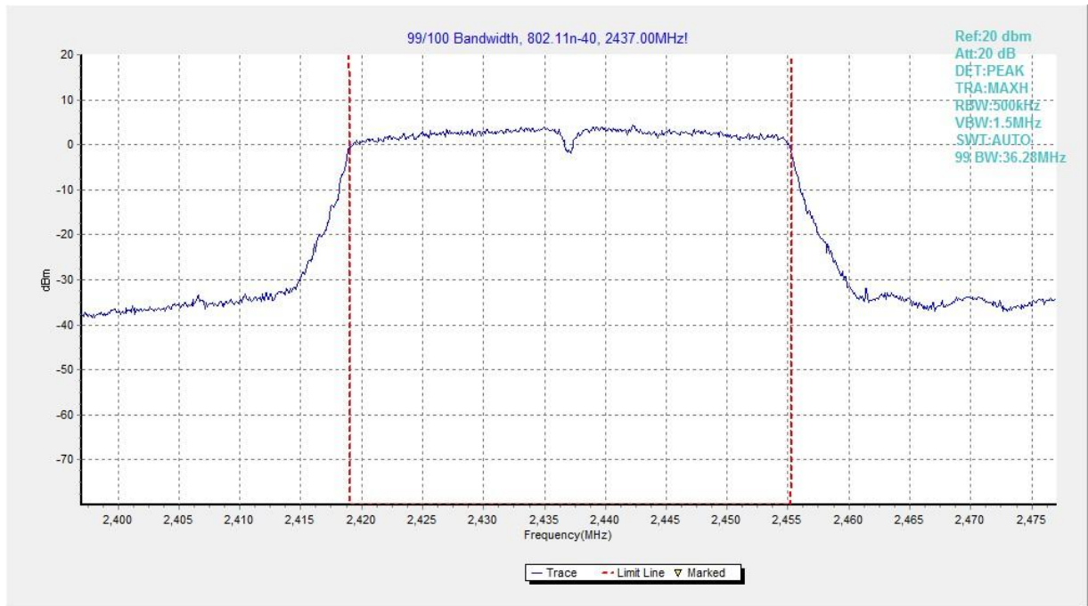
Fig.81 99% Occupied Bandwidth (802.11n HT40, CH 6)
