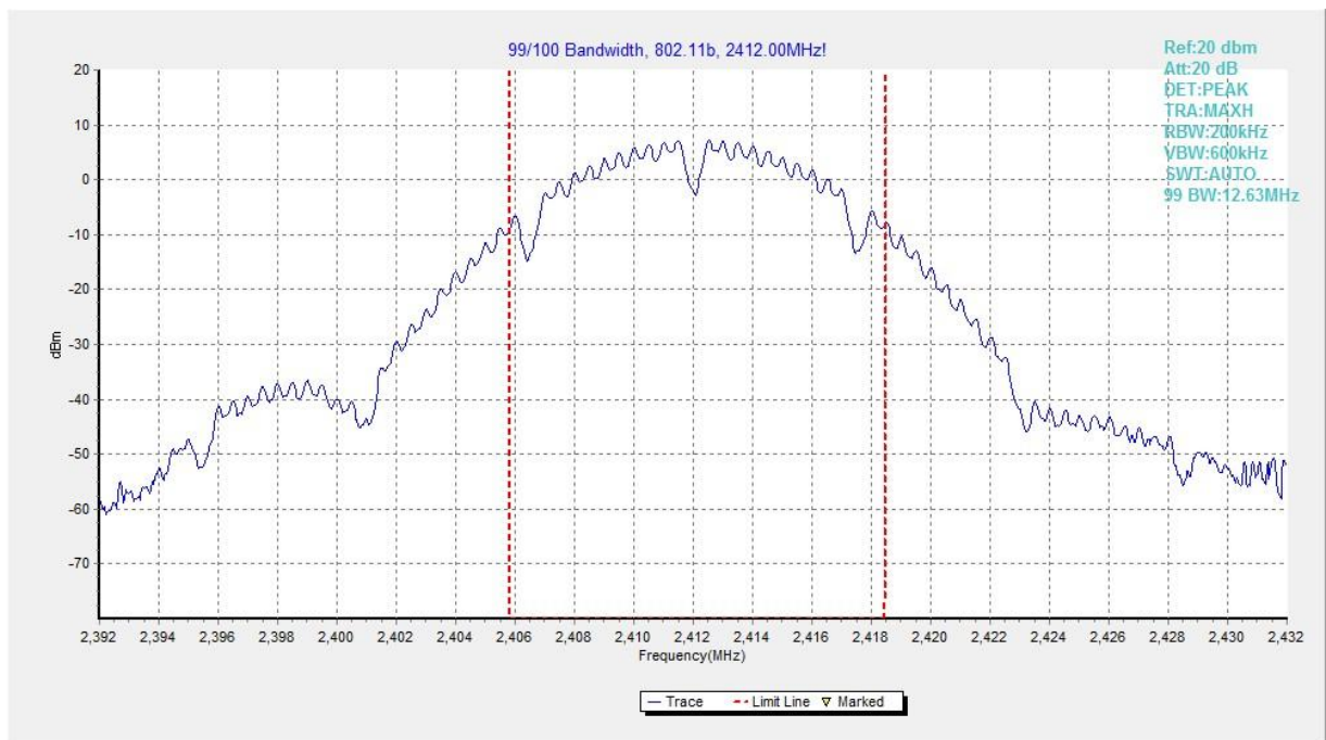
Fig.71 99% Occupied Bandwidth (802.11b, CH 1)
