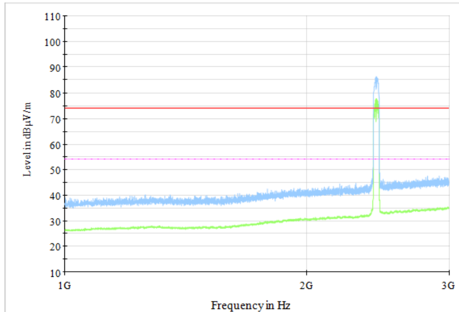
Fig.60 Radiated Spurious Emission (802.11n HT40, CH6, 1GHz-3GHz)
