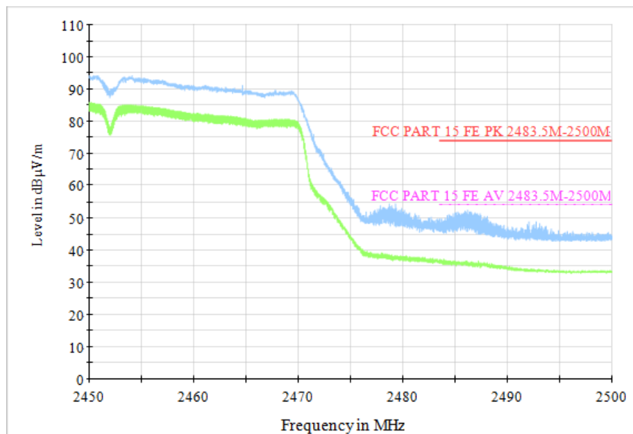
Fig.65 Radiated Restricted Band (802.11n HT40, CH9, 2.45GHz~2.5GHz)
