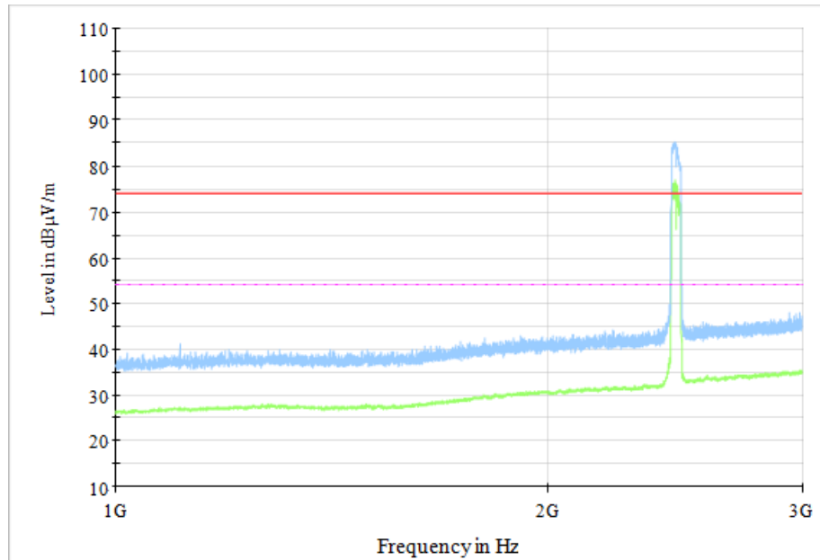
Fig.62 Radiated Spurious Emission (802.11n HT40, CH9, 1GHz-3GHz)
