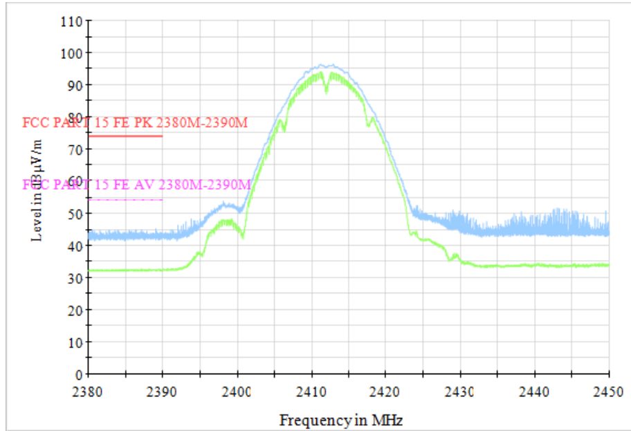
Fig.40 Radiated Restricted Band (802.11b, CH1, 2.38GHz~2.45GHz)
