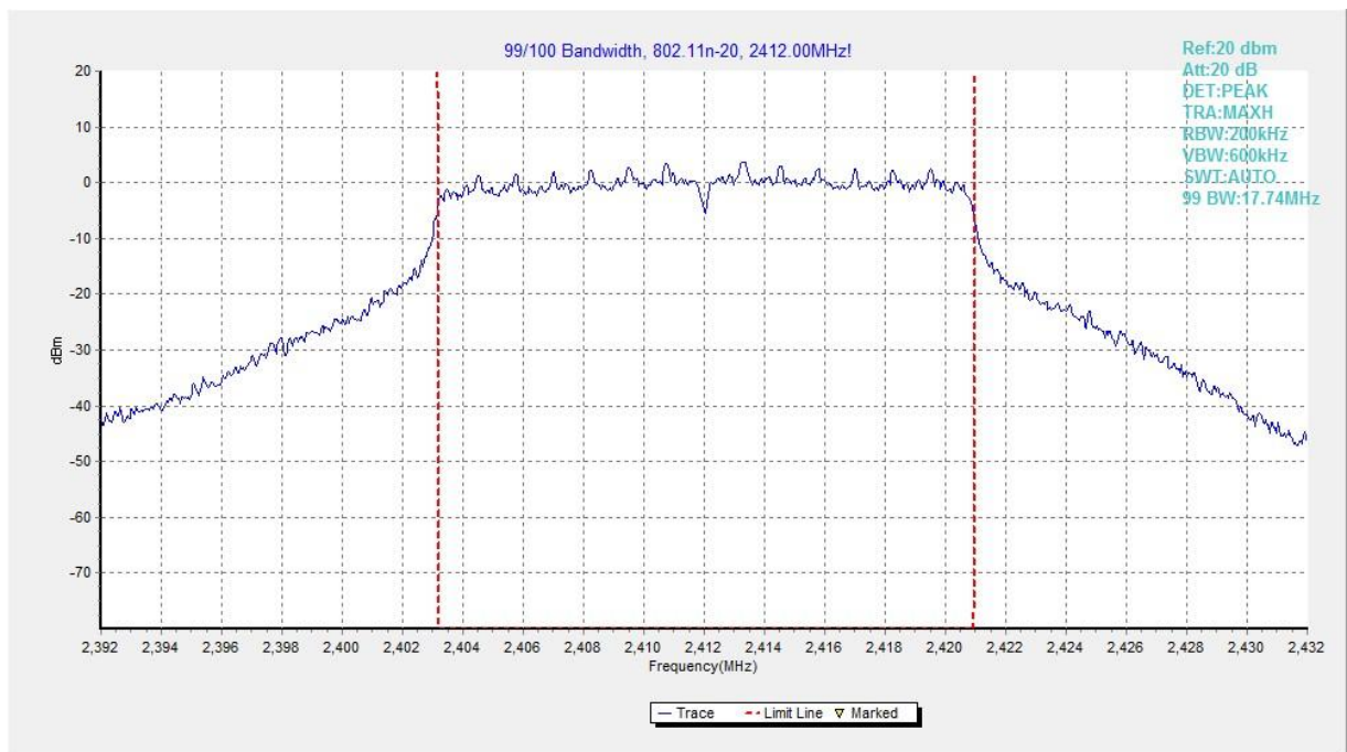
Fig.77 99% Occupied Bandwidth (802.11n HT20, CH 1)
