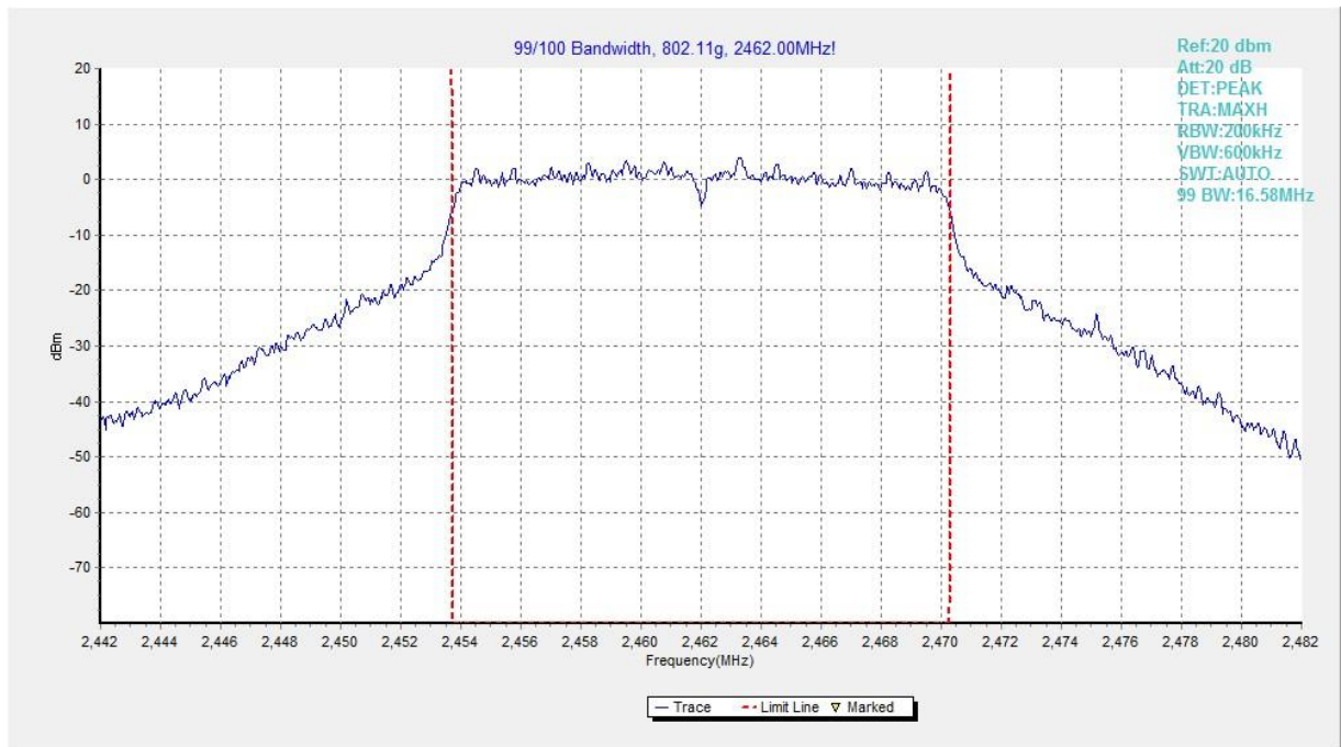
Fig.76 99% Occupied Bandwidth (802.11g, CH 11)
