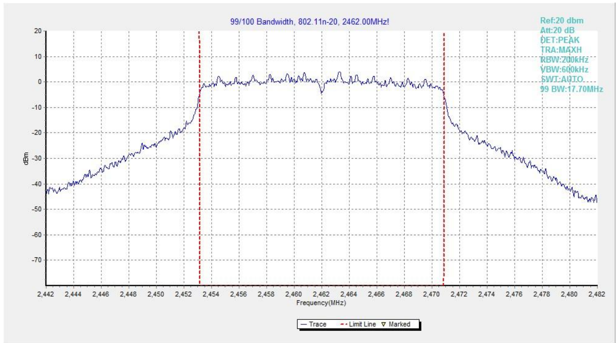
Fig.79 99% Occupied Bandwidth (802.11n HT20, CH 11)
