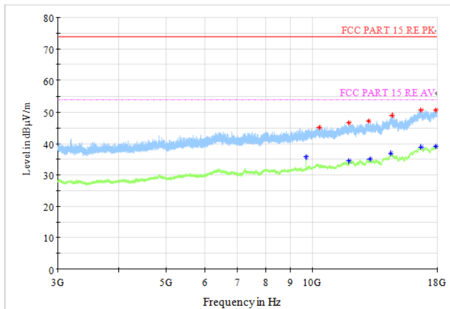
Fig.59 Radiated Spurious Emission (802.11n HT40, CH3, 3GHz-18GHz)
