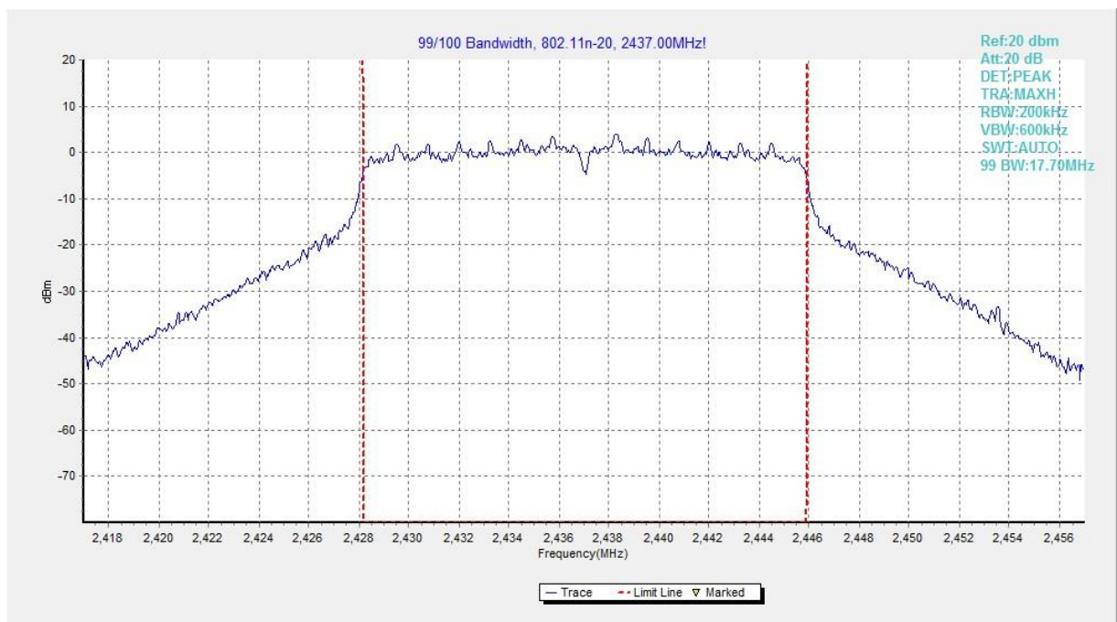
Fig.78 99% Occupied Bandwidth (802.11n HT20, CH 6)
