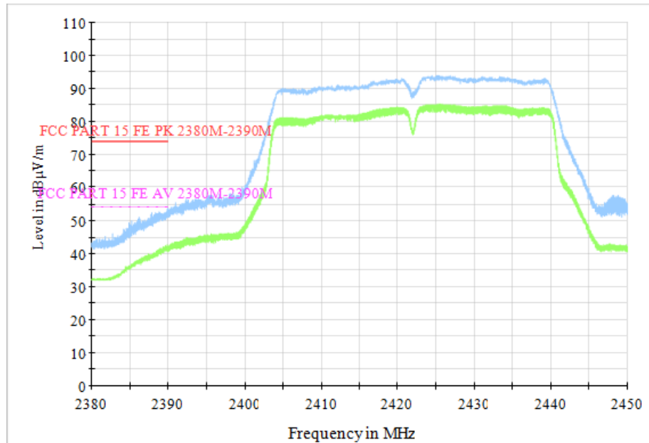
Fig.64 Radiated Restricted Band (802.11n HT40, CH3, 2.38GHz~2.45GHz)
