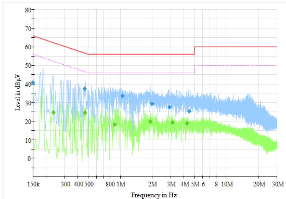
Fig.69 AC Power line Conducted Emission (Traffic, AE1, 120V)
