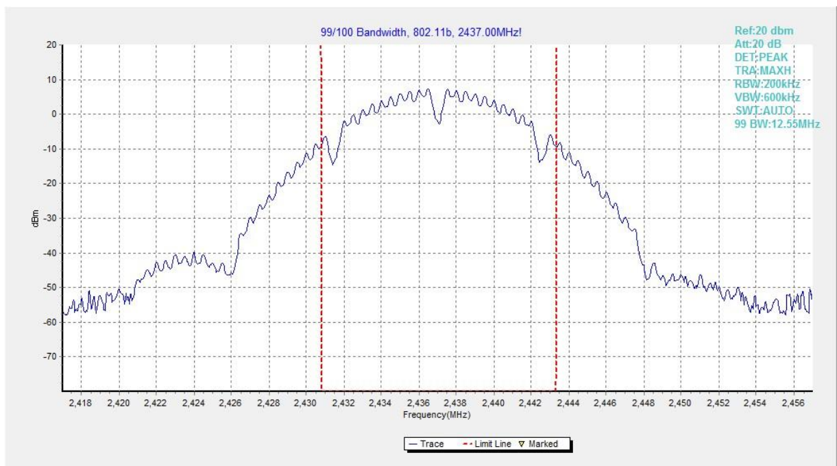
Fig.72 99% Occupied Bandwidth (802.11b, CH 6)
