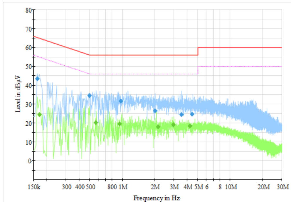
Fig.70 AC Power line Conducted Emission (Idle, AE1, 120V)
