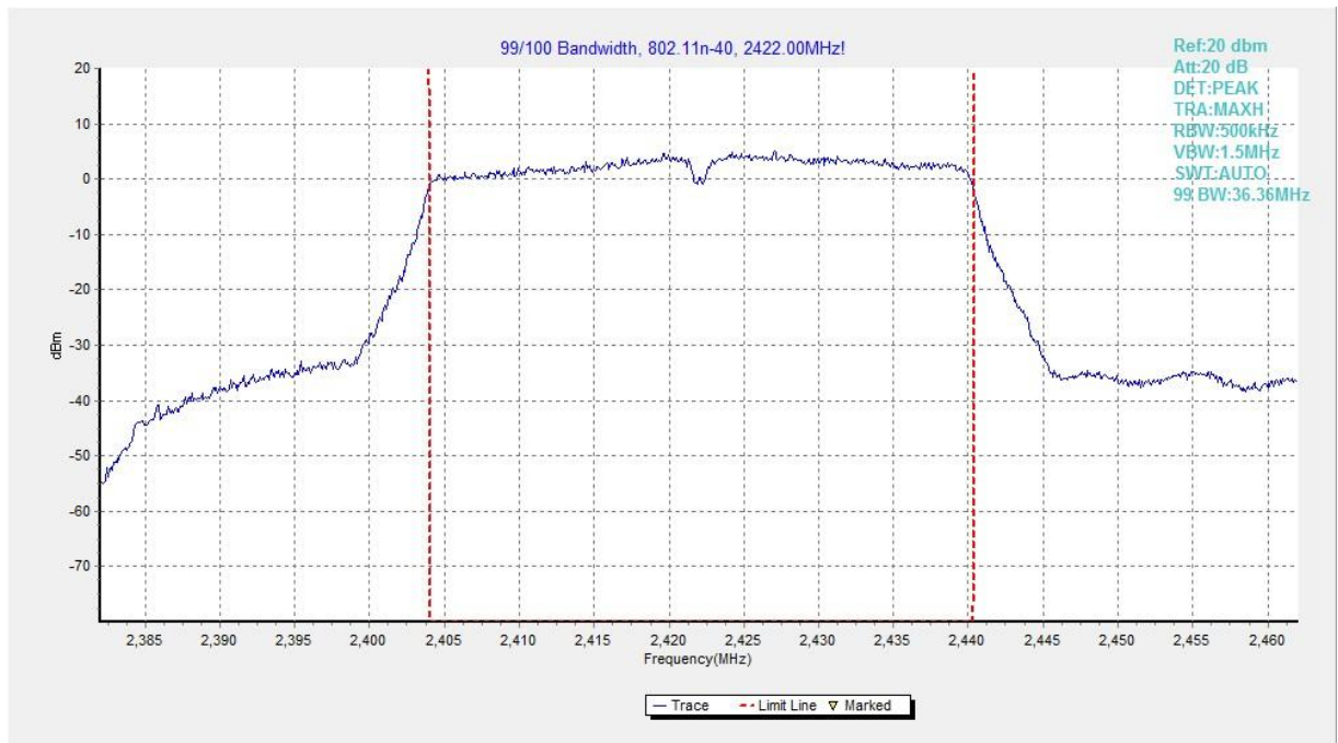
Fig.80 99% Occupied Bandwidth (802.11n HT40, CH 3)
