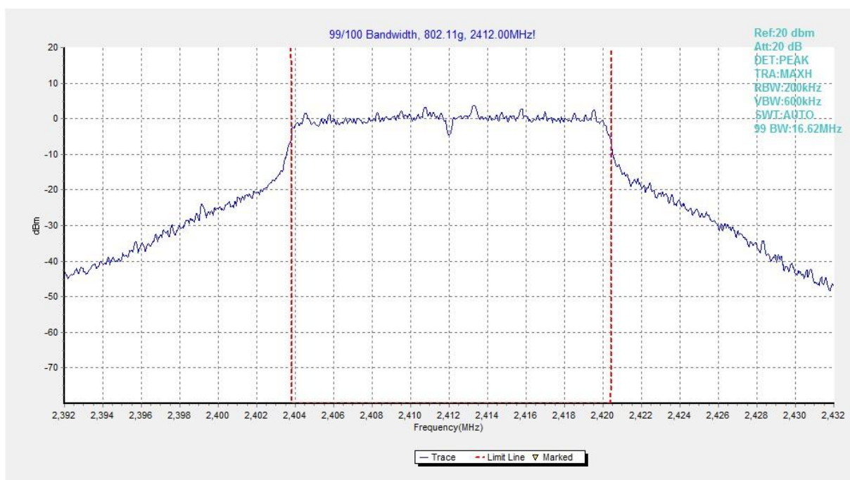
Fig.74 99% Occupied Bandwidth (802.11g, CH 1)
