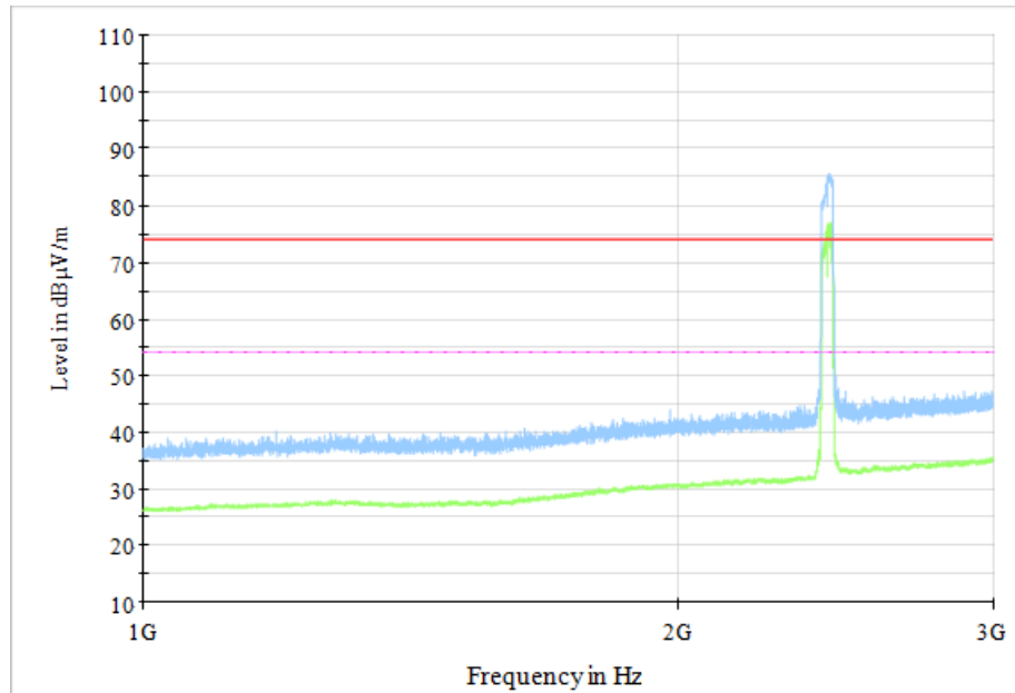
Fig.58 Radiated Spurious Emission (802.11n HT40, CH3, 1GHz-3GHz)
