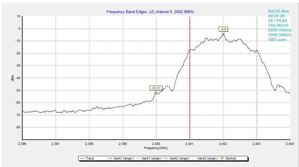
Fig.27 Band Edges (Ch 0), LE 2M
