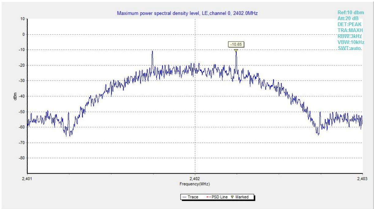
Fig.10 Power Spectral Density (Ch 0), LE Coded (S=2)
