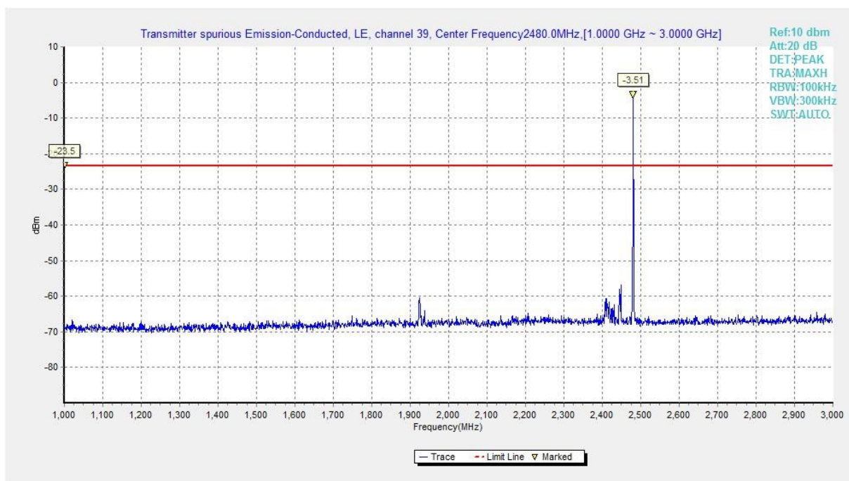
Fig.40 Conducted Spurious Emission (Ch39, 1 GHz-3 GHz), LE 1M
