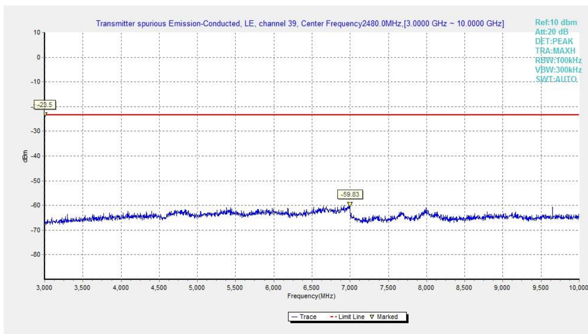
Fig.41 Conducted Spurious Emission (Ch39, 3 GHz-10 GHz), LE 1M
