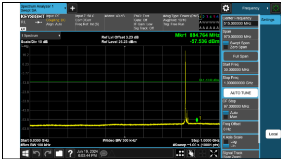
Band26_15MHz_QPSK_26865_1RB#0_30~1000_30~1000
