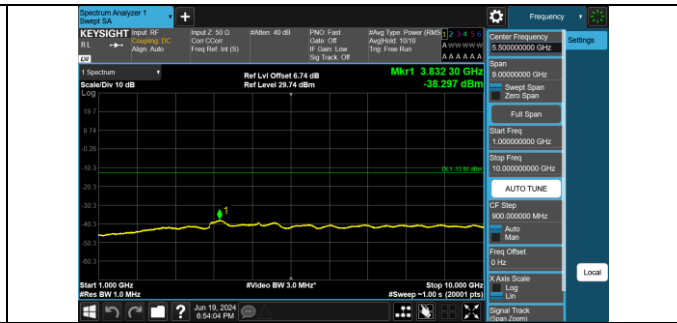
Band26_15MHz_QPSK_26865_1RB#0_1000~10000_1000~10000
