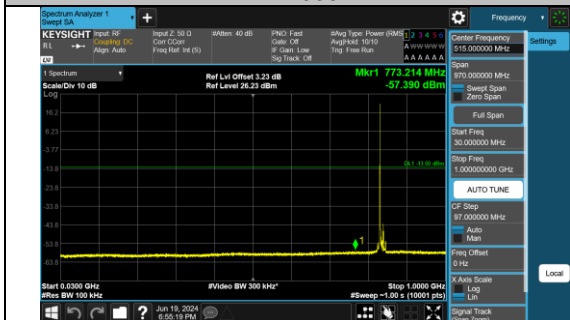
Band26_15MHz_QPSK_26965_1RB#0_30~1000_30~1000
