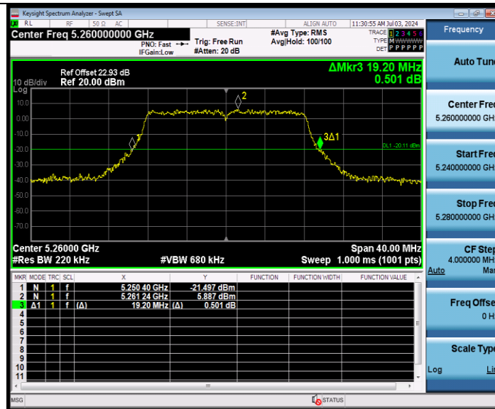
11A-CDD Ant9 5260
