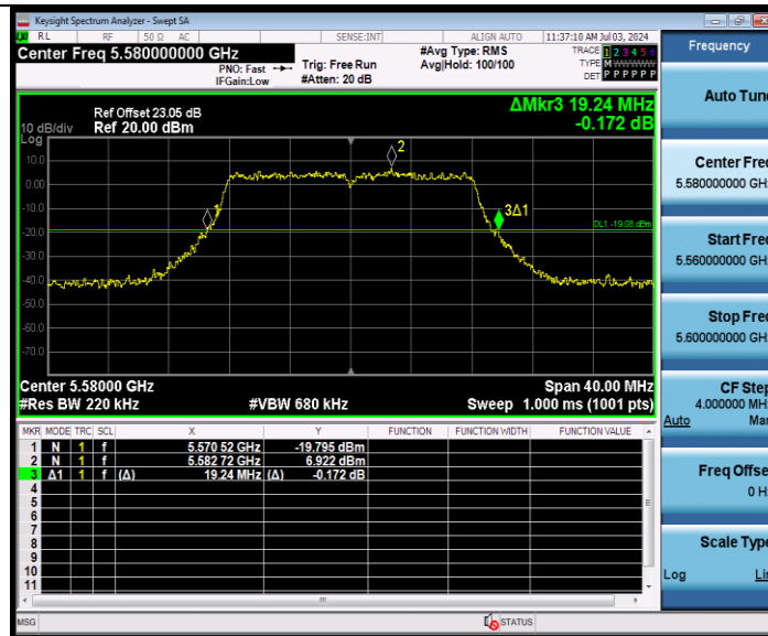
11A-CDD Ant9 5580
