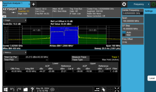
48-48-20MHz-20MHz-16QAM-16QAM-55891-56089-100 RB#0-100RB#0-PASS
