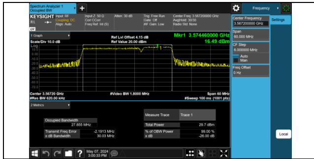
48-48-20MHz-10MHz-QPSK-QPSK-55340-55484-100R B#0-50RB#0-PASS
