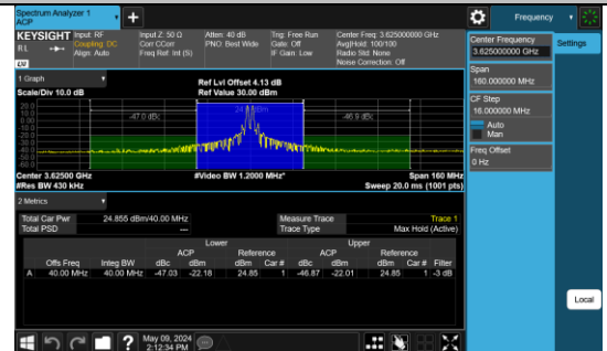
48-48-20MHz-20MHz-16QAM-16QAM-55891-56089-1R B#99-1RB#0-PASS
