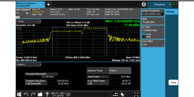
48-48-20MHz-15MHz-QPSK-QPSK-55916-56087-100R B#0-75RB#0-PASS
