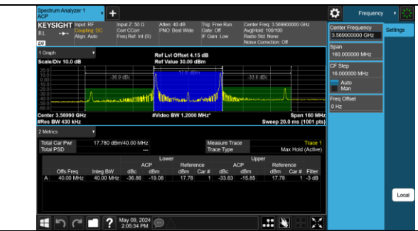
48-48-20MHz-20MHz-16QAM-16QAM-55340-55538-1R B#0-1RB#99-PASS
