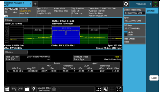
48-48-20MHz-20MHz-16QAM-16QAM-55340-55538-100 RB#0-100RB#0-PASS
