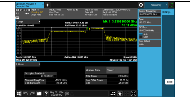
48-48-20MHz-10MHz-QPSK-QPSK-55941-56064-100R B#0-50RB#0-PASS
