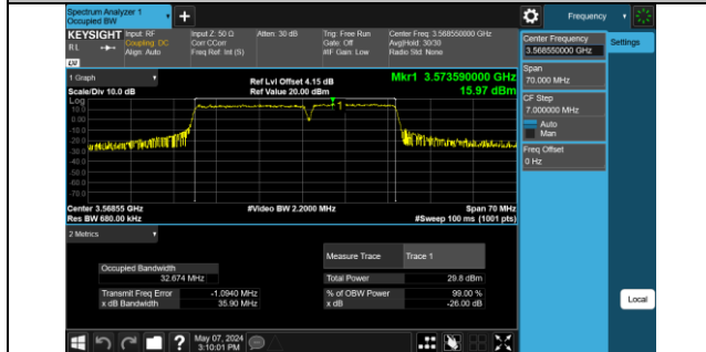
48-48-20MHz-15MHz-QPSK-QPSK-55340-55511-100RB #0-75RB#0-PASS
