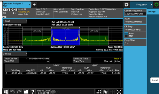
48-48-20MHz-20MHz-16QAM-16QAM-55891-56089-1R B#0-1RB#99-PASS
