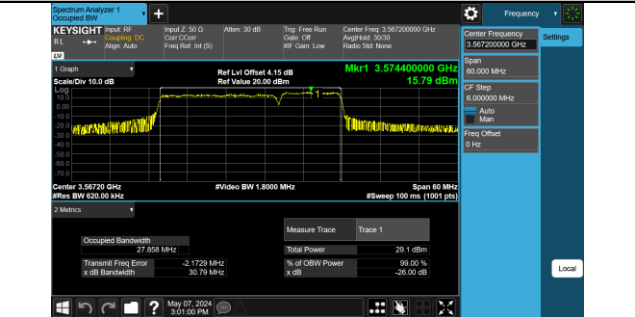
48-48-20MHz-10MHz-16QAM-16QAM-55340-55484-100 RB#0-50RB#0-PASS
