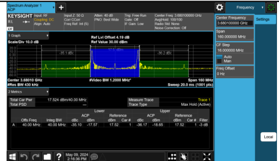
48-48-20MHz-20MHz-16QAM-16QAM-56442-56640-1R B#0-1RB#99-PASS
