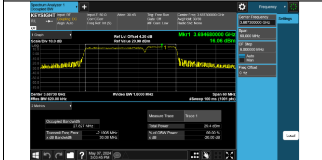
48-48-20MHz-10MHz-QPSK-QPSK-56541-56685-100R B#0-50RB#0-PASS
