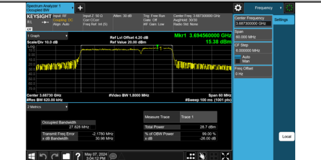
48-48-20MHz-10MHz-16QAM-16QAM-56541-56685-100 RB#0-50RB#0-PASS
