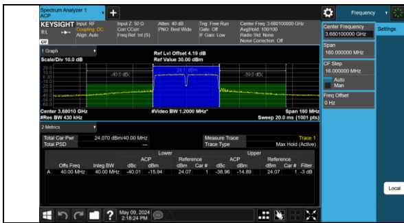
48-48-20MHz-20MHz-QPSK-QPSK-56442-56640-100R B#0-100RB#0-PASS
