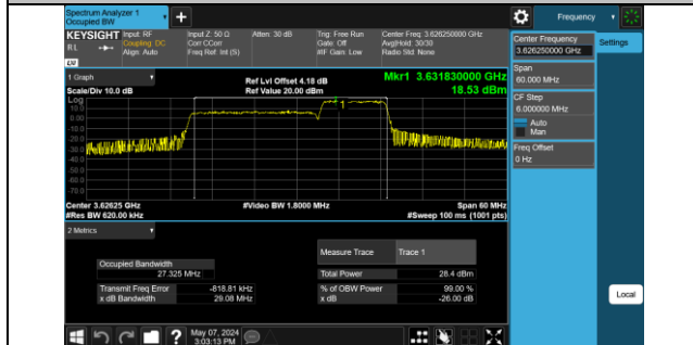
48-48-20MHz-10MHz-16QAM-16QAM-55941-56064-100 RB#0-50RB#0-PASS
