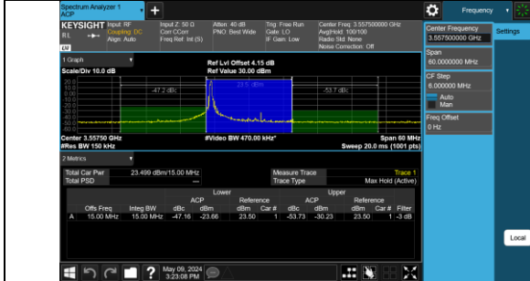
Band48-15MHz-QPSK-55315-1RB#0-PASS
