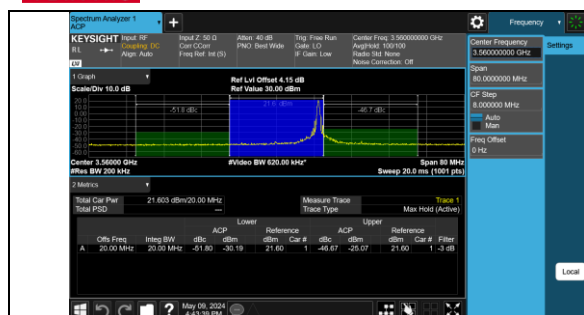
Band48-20MHz-16QAM-55340-1RB#99-PASS
