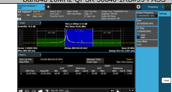
Band48-20MHz-16QAM-55340-1RB#0-PASS
