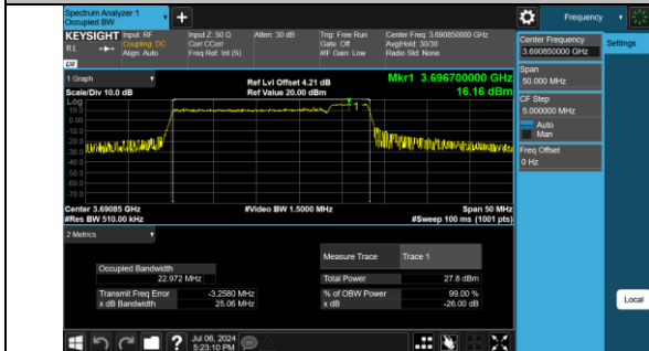
48-48-20MHz-5MHz-QPSK-QPSK-56590-56707-100RB #0-25RB#0-PASS
