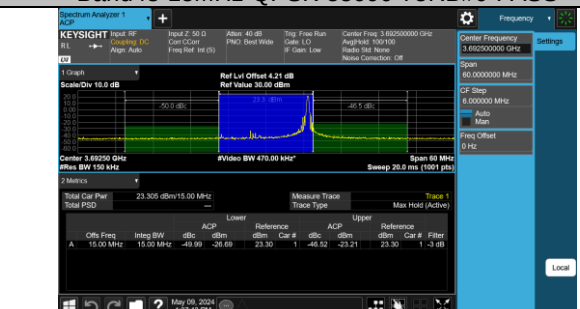
Band48-15MHz-QPSK-56665-1RB#74-PASS
