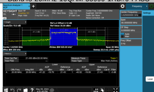
Band48-20MHz-16OAM-55990-100RB#0-PASS
