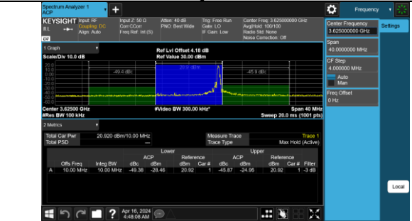
Band48-10MHz-16QAM-55990-1RB#49-PASS
