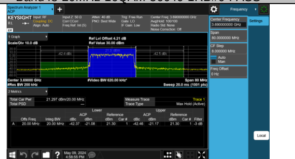
Band48-20MHz-16QAM-56640-100RB#0-PASS
