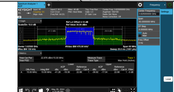
Band48-15MHz-QPSK-55990-75RB#0-PASS
