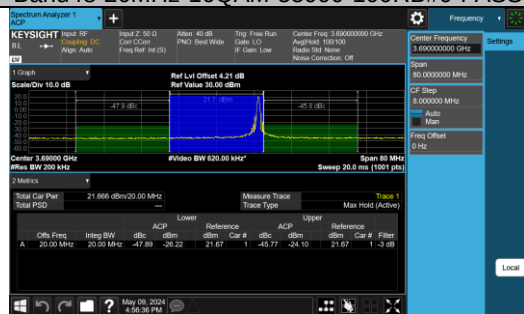
Band48-20MHz-16QAM-56640-1RB#99-PASS
