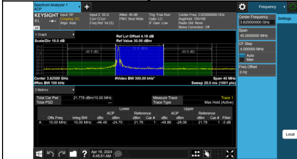
Band48-10MHz-16QAM-55990-1RB#0-PASS
