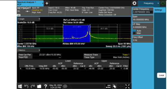
Band48-15MHz-QPSK-55315-1RB#74-PASS
