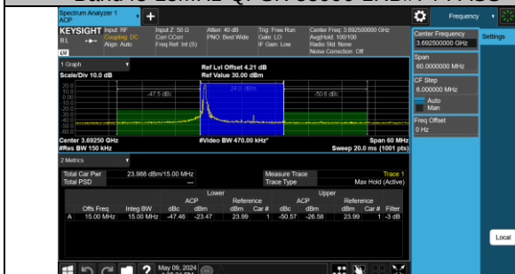
Band48-15MHz-QPSK-56665-1RB#0-PASS
