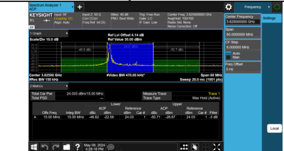
Band48-15MHz-QPSK-55990-1RB#0-PASS
