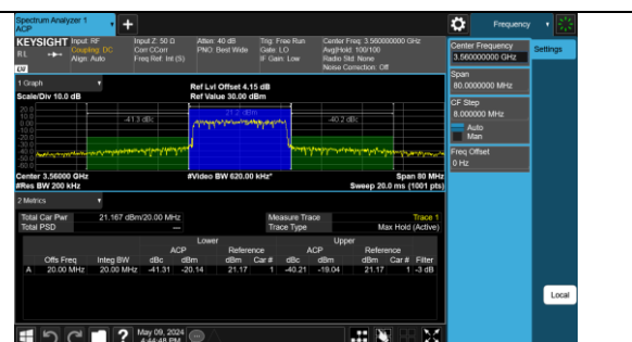
Band48-20MHz-16QAM-55340-100RB#0-PASS
