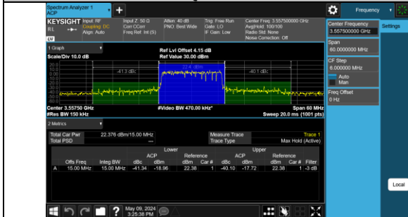
Band48-15MHz-QPSK-55315-75RB#0-PASS
