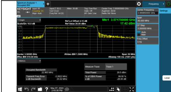
48-48-20MHz-5MHz-QPSK-QPSK-55340-55457-100RB #0-25RB#0-PASS
