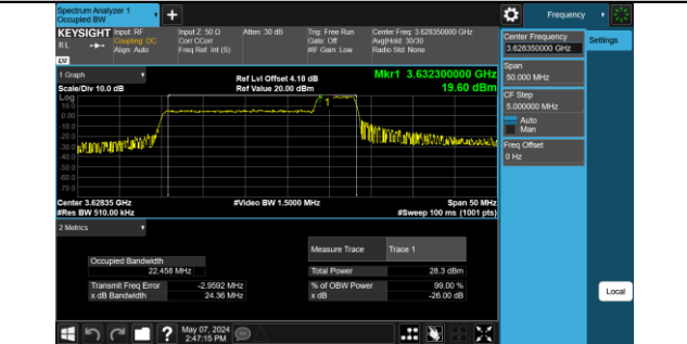
48-48-20MHz-5MHz-QPSK-QPSK-55965-56082-100RB #0-25RB#0-PASS
