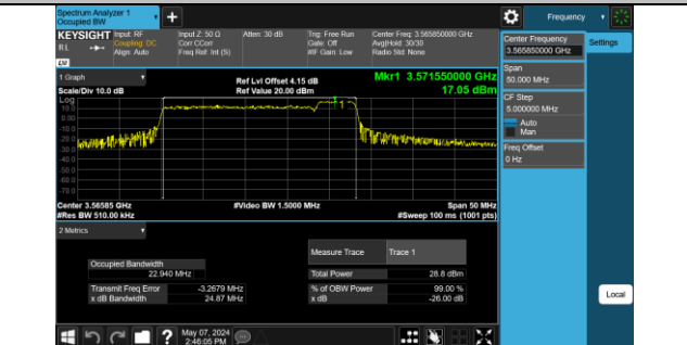
48-48-20MHz-5MHz-16QAM-16QAM-55340-55457-100R B#0-25RB#0-PASS
