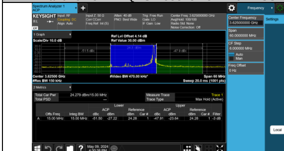
Band48-15MHz-QPSK-55990-1RB#74-PASS
