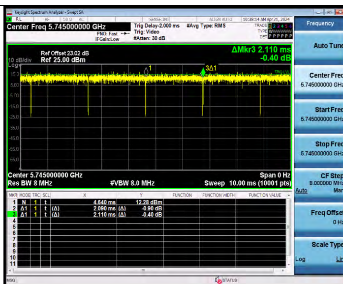
11A-CDD Ant9 5745
