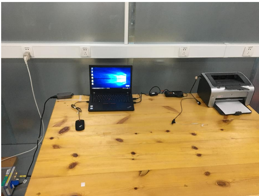
16. Conducted Emission (Part 15B Data transfer mode)
