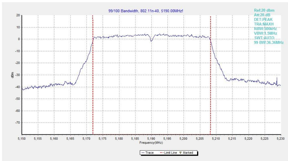
Fig. 36 99% Occupied Bandwidth (802.11n-HT40, 5190MHz)
