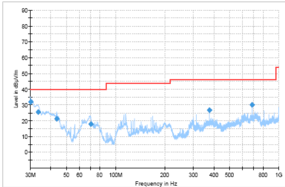
Figure A.1 Radiated Emission (Set.1, Video Play Mode, 30MHz to 1GHz)
