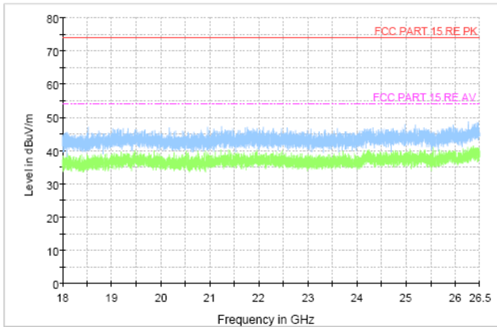
Figure A.9 Radiated Emission (Set.1, Camera Mode , 18GHz to 26.5GHz)
