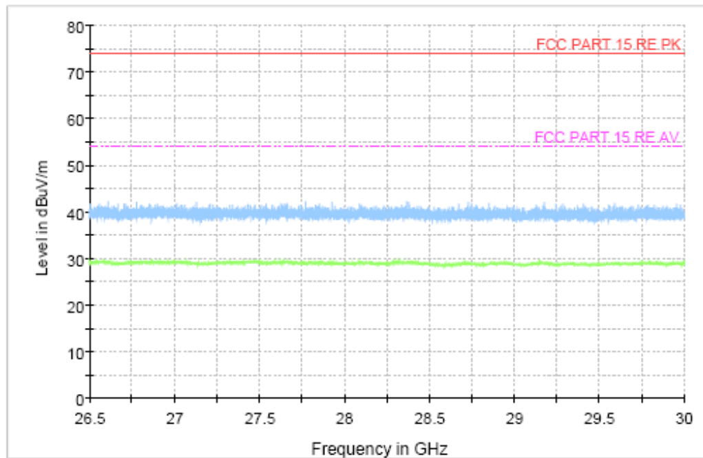
Figure A.25 Radiated Emission (Set.2, Data Transfer Mode Mode/EUT to PC, 26.5GHz to 30GHz)
