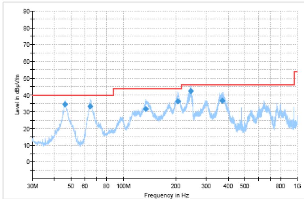
Figure A.16 Radiated Emission (Set.3,Data Transfer Mode Mode/PC to EUT, 30MHz to 1GHz)
