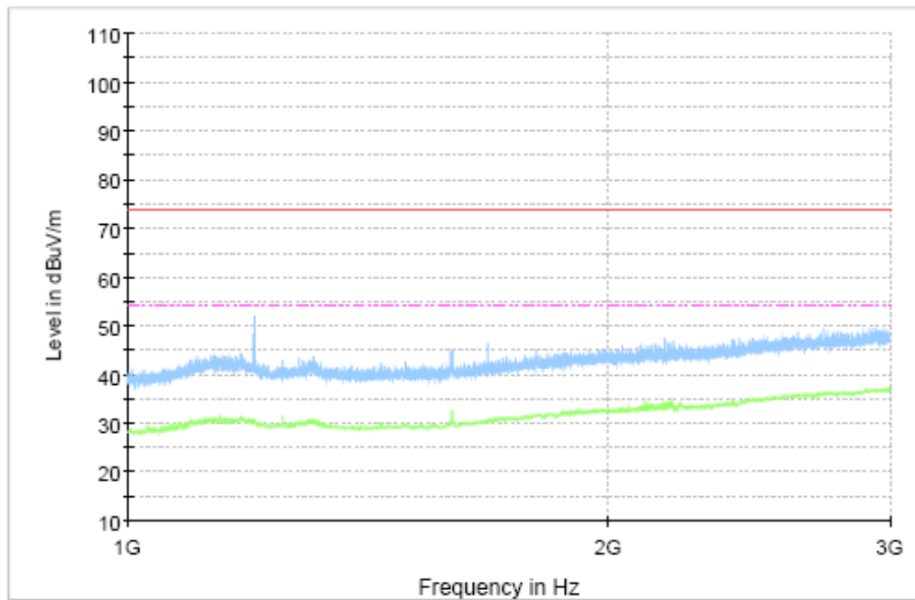
Figure A.17 Radiated Emission (Set.2, Data Transfer Mode Mode/PC to EUT, 1GHz to 3GHz)
