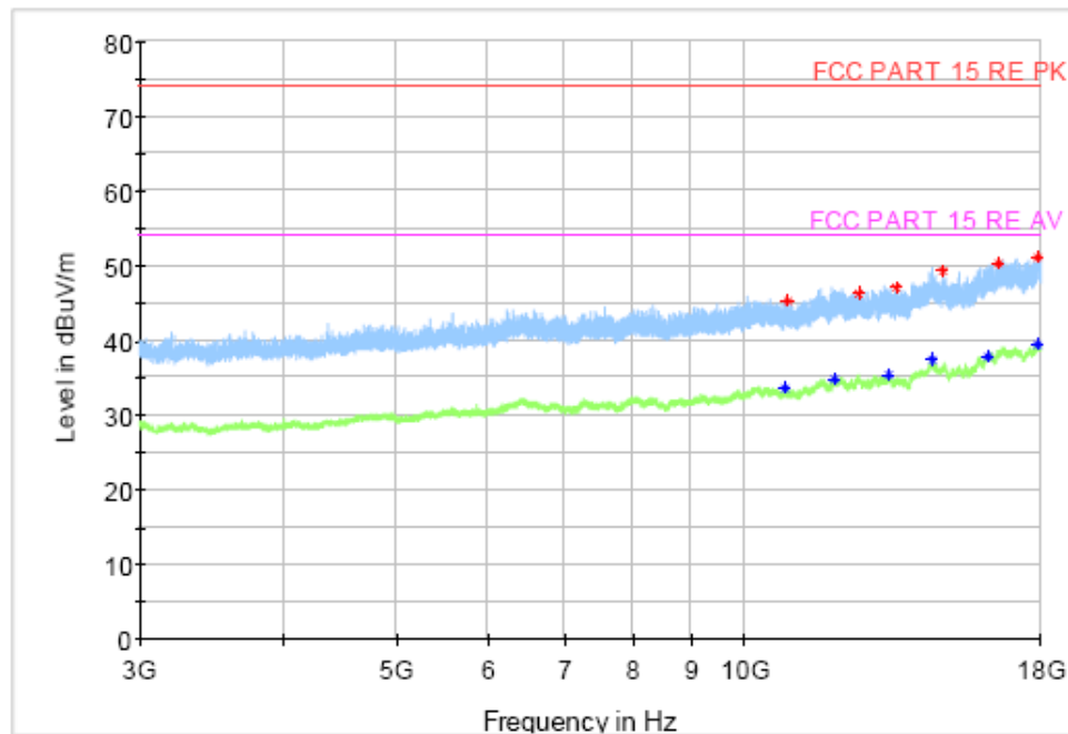
Figure A.18 Radiated Emission (Set.2, Data Transfer Mode Mode/PC to EUT, 3GHz to 18GHz)
