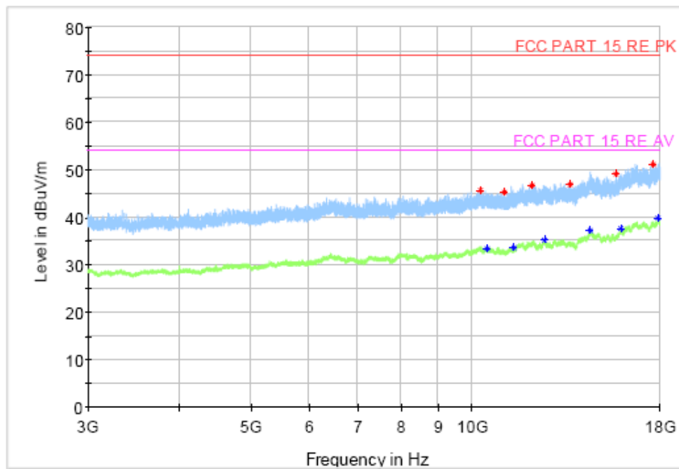
Figure A.23 Radiated Emission (Set.2, Data Transfer Mode Mode/EUT to PC, 3GHz to 18GHz)
