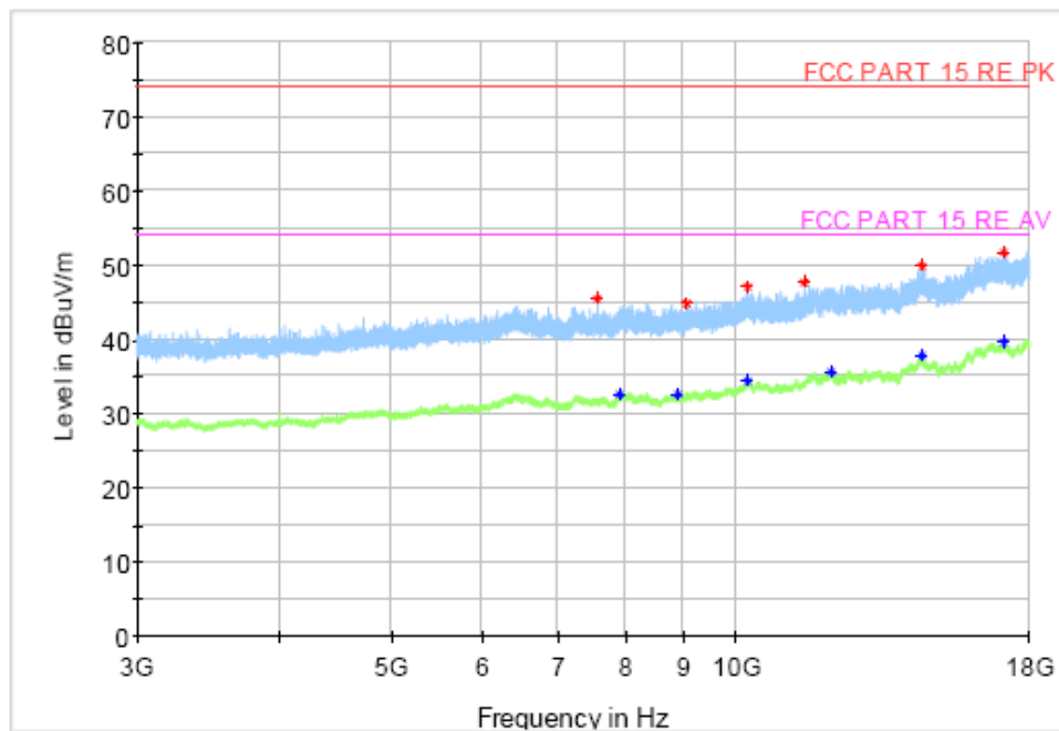
Figure A.28 Radiated Emission (Set.2, Data Transfer Mode Mode/PC to TF Card, 3GHz to 18GHz)
