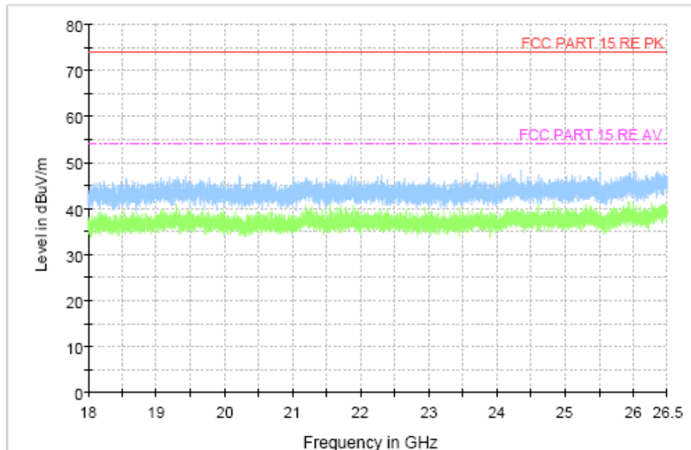
Figure A.14 Radiated Emission (Set.1,Charging Mode , 18GHz to 26.5GHz)
