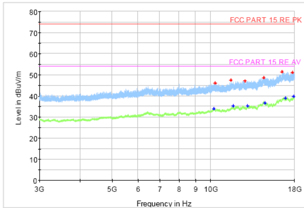
Figure A.33 Radiated Emission (Set.2, Data Transfer Mode Mode/TF Card to PC, 3GHz to 18GHz)
