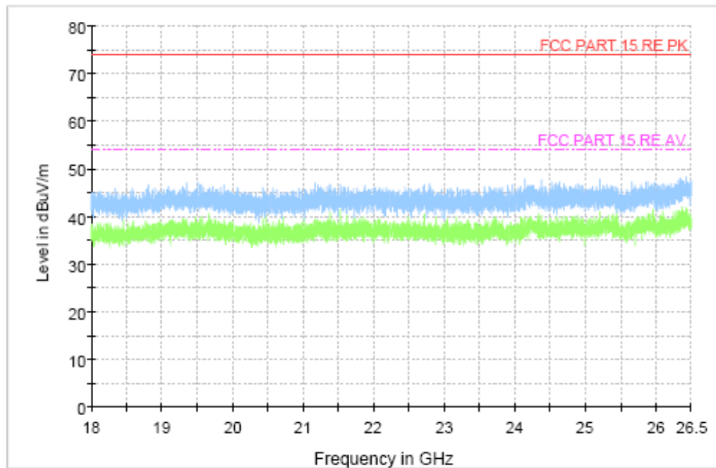
Figure A.29 Radiated Emission (Set.2, Data Transfer Mode Mode/PC to TF Card, 18GHz to 26.5GHz)
