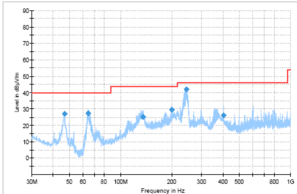
Figure A.31 Radiated Emission (Set.3, Data Transfer Mode Mode/TF Card to PC, 30MHz to 1GHz)
