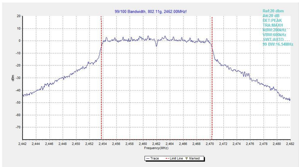
Fig.70 99% Occupied Bandwidth (802.11g, CH 11)
