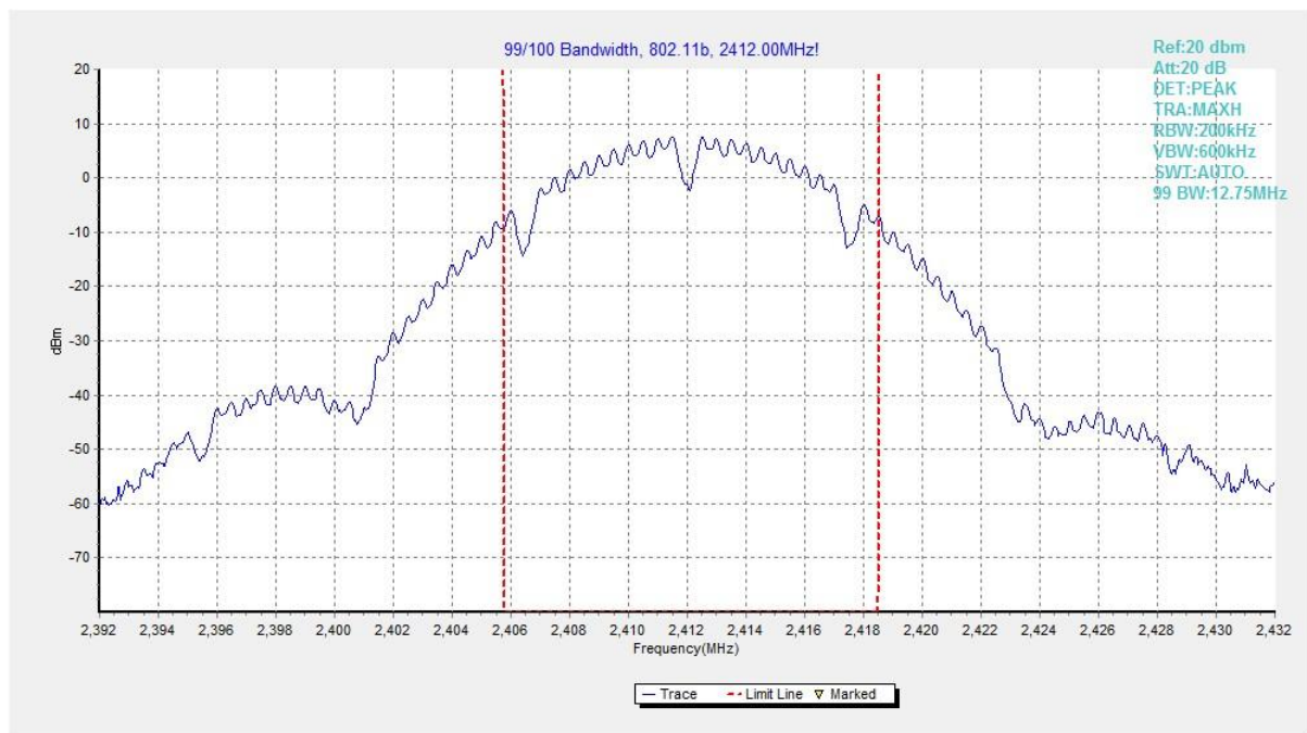
Fig.65 99% Occupied Bandwidth (802.11b, CH 1)
