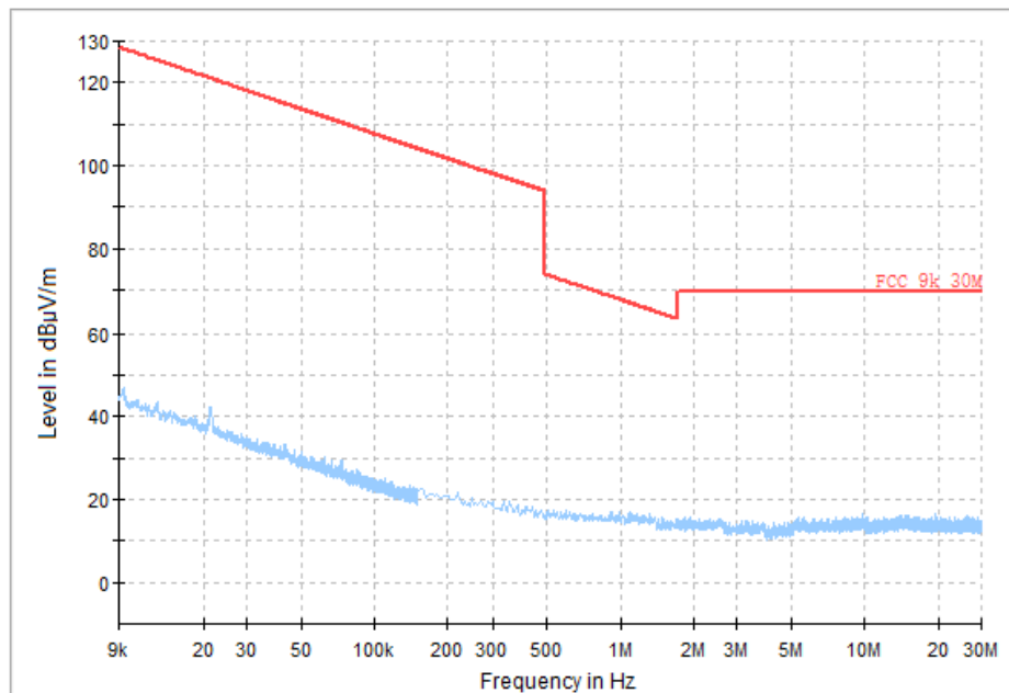
Fig.41 Radiated Spurious Emission (Ch19, 9 kHz - 30 MHz), 1M
