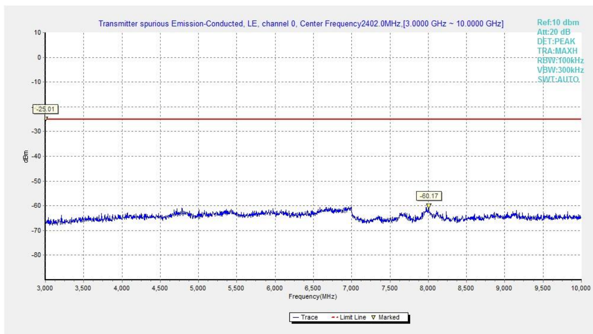
Fig.19 Conducted Spurious Emission (Ch0, 3 GHz-10 GHz), LE 1M
