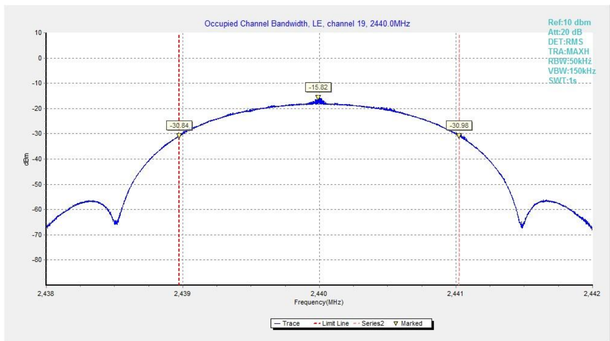
Fig.69 Occupied Bandwidth (Ch 19), 2M
