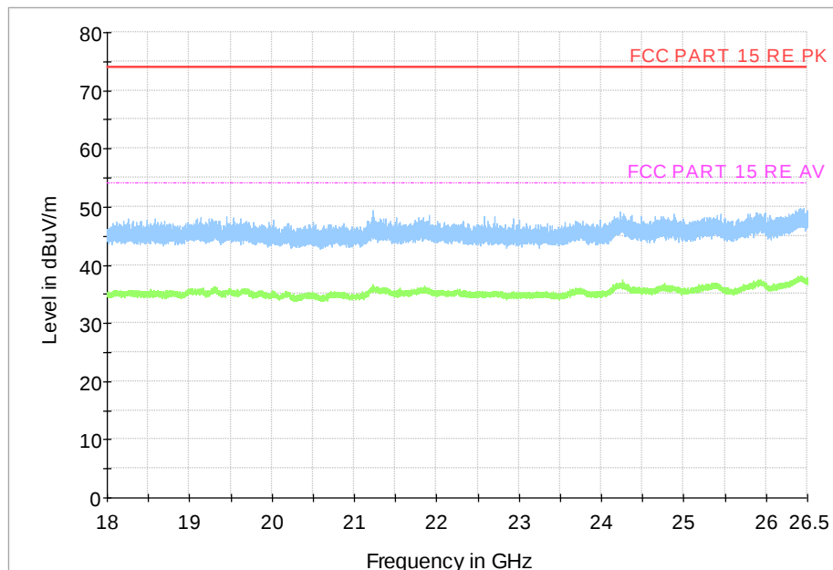
Fig.56 Radiated Spurious Emission (Ch19, 18 GHz - 26.5 GHz), 2M
