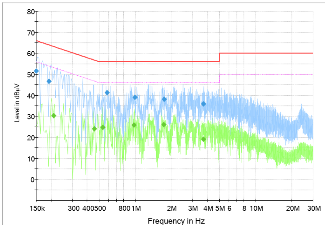
Fig.63 AC Power line Conducted Emission (Traffic, AE1, 240V), 1M
