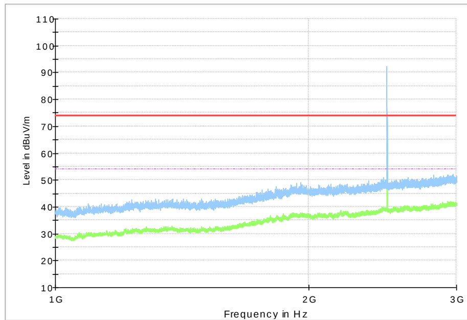
Fig.46 Radiated Spurious Emission (Ch39, 1 GHz - 3 GHz), 1M
