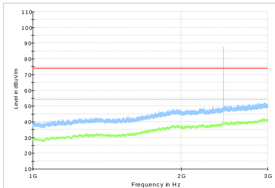
Fig.54 Radiated Spurious Emission (Ch19, 1 GHz - 3 GHz), 2M
