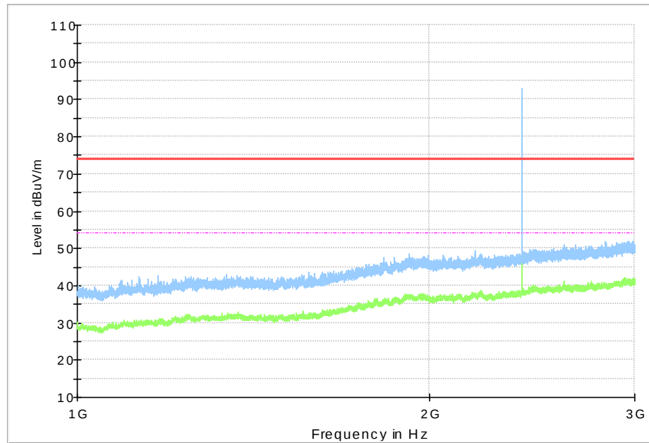
Fig.39 Radiated Spurious Emission (Ch0, 1 GHz - 3 GHz), 1M
