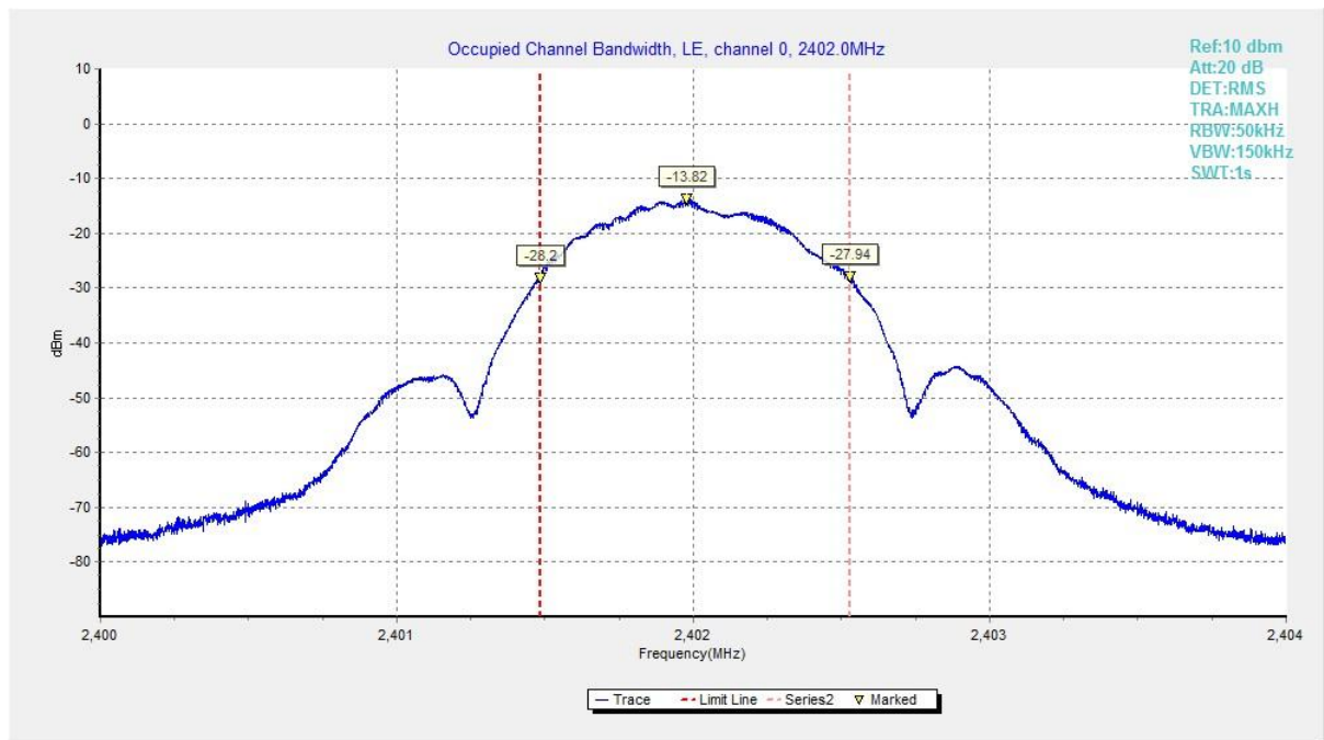
Fig.65 Occupied Bandwidth (Ch 0), 1M
