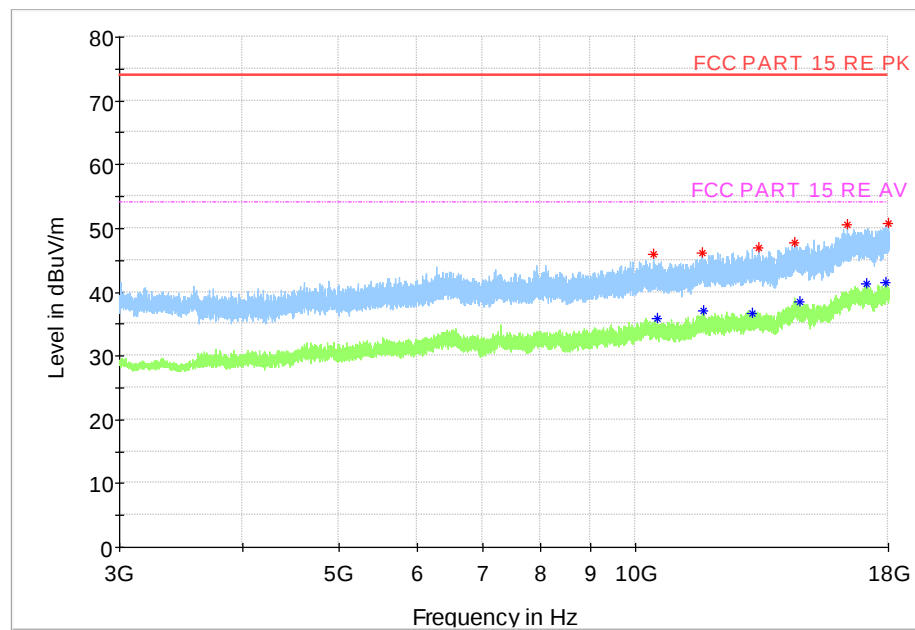
Fig.58 Radiated Spurious Emission (Ch39, 3 GHz - 18 GHz), 2M
