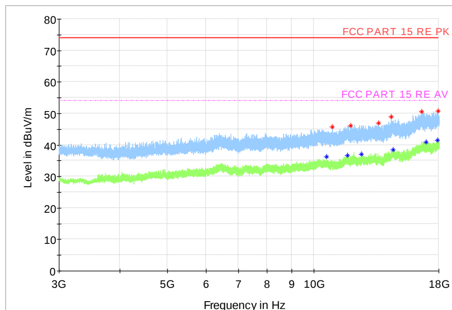
Fig.40 Radiated Spurious Emission (Ch0, 3 GHz - 18 GHz), 1M
