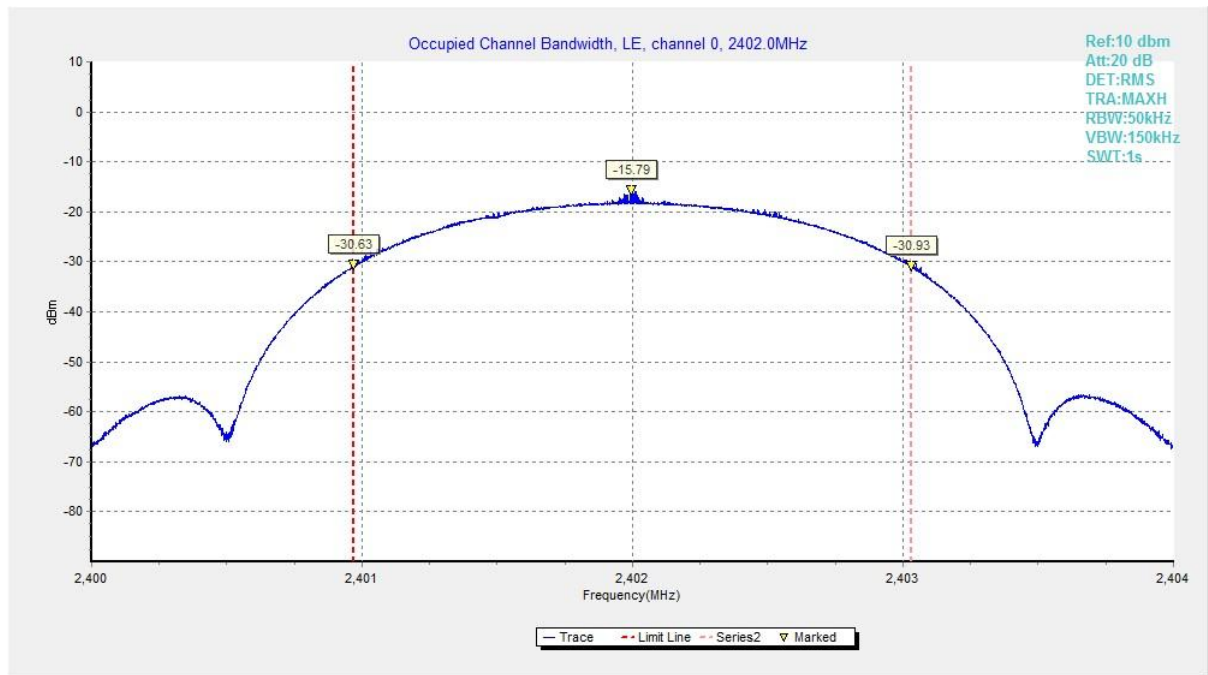
Fig.68 Occupied Bandwidth (Ch 0), 2M
