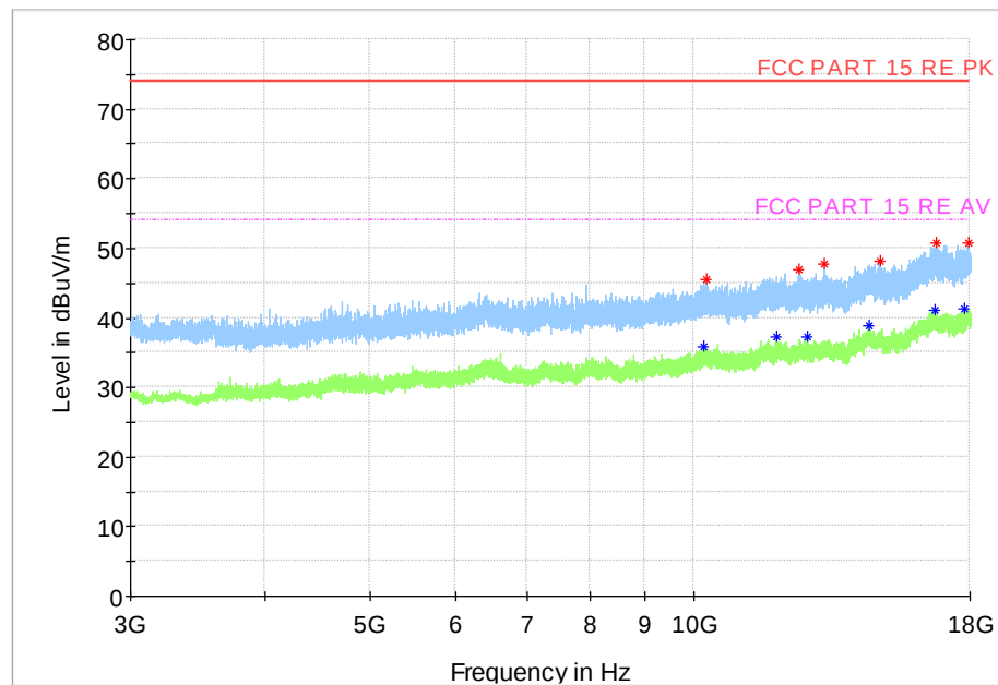
Fig.47 Radiated Spurious Emission (Ch39, 3 GHz - 18 GHz), 1M
