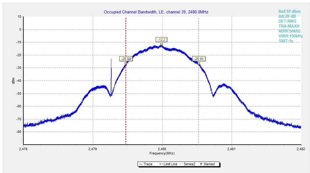
Fig.67 Occupied Bandwidth (Ch 39), 1M
