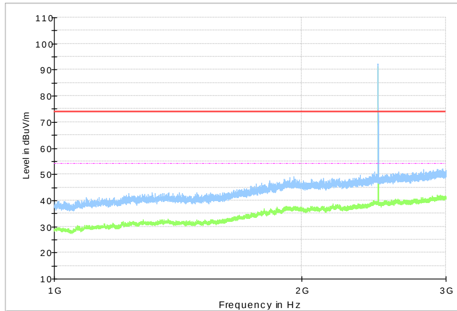
Fig.57 Radiated Spurious Emission (Ch39, 1 GHz - 3 GHz), 2M
