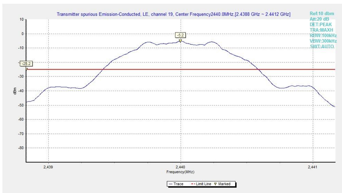
Fig.20 Conducted Spurious Emission (Ch19, Center Frequency), LE 1M
