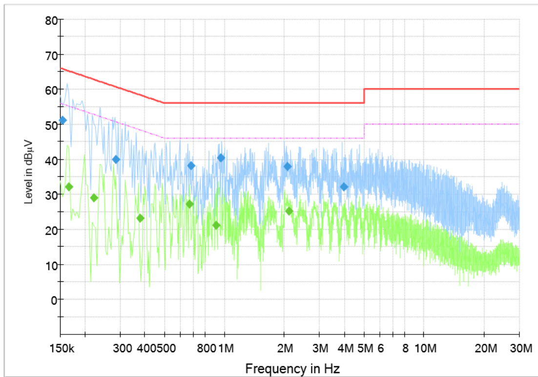
Fig.64 AC Power line Conducted Emission (Idle, AE1, 240V), 1M
