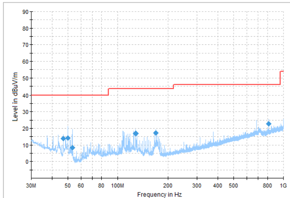
Fig.53 Radiated Spurious Emission (Ch19, 30 MHz - 1 GHz), 2M
