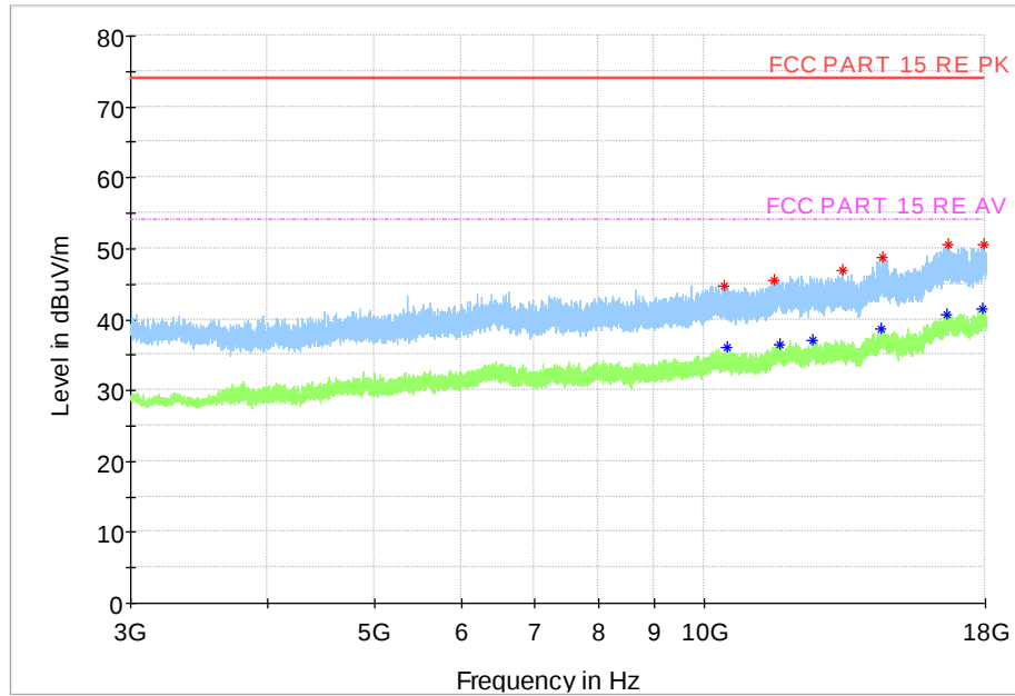
Fig.55 Radiated Spurious Emission (Ch19, 3 GHz - 18 GHz), 2M
