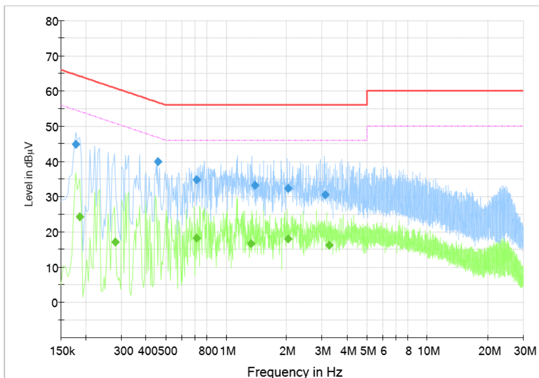
Fig.61 AC Power line Conducted Emission (Traffic, AE1, 120V), 1M
