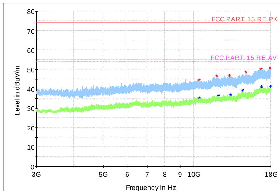
Fig.44 Radiated Spurious Emission (Ch19, 3 GHz - 18 GHz), 1M
