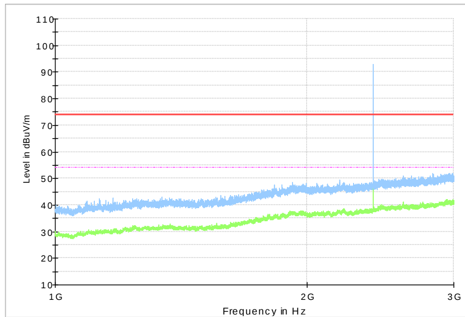
Fig.50 Radiated Spurious Emission (Ch0, 1 GHz - 3 GHz), 2M
