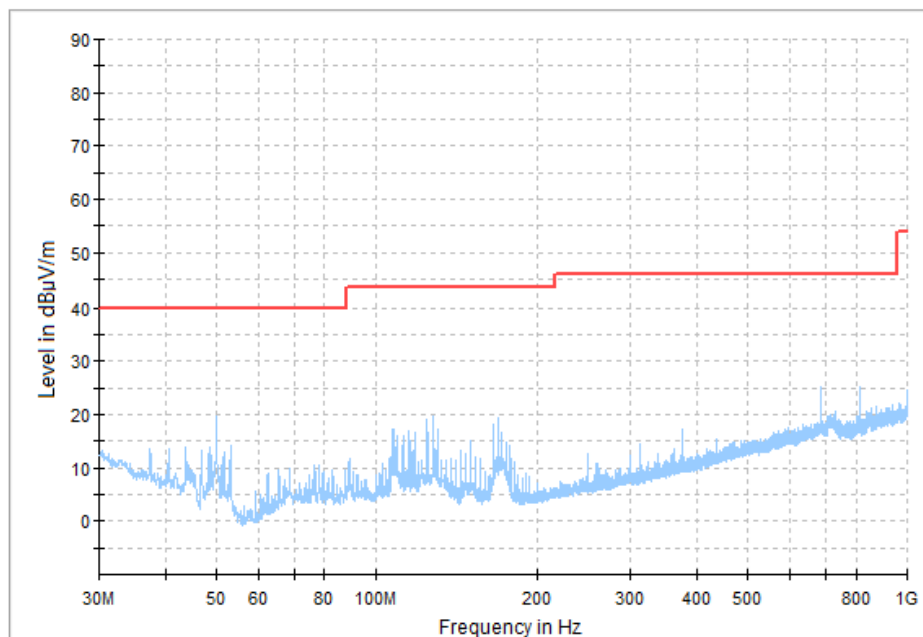
Fig.42 Radiated Spurious Emission (Ch19, 30 MHz - 1 GHz), 1M
