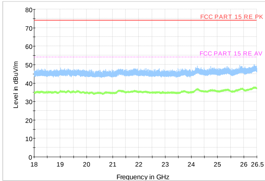
Fig.45 Radiated Spurious Emission (Ch19, 18 GHz - 26.5 GHz), 1M
