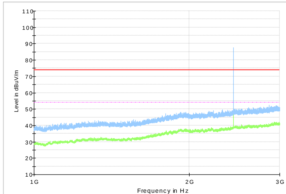
Fig.43 Radiated Spurious Emission (Ch19, 1 GHz - 3 GHz), 1M
